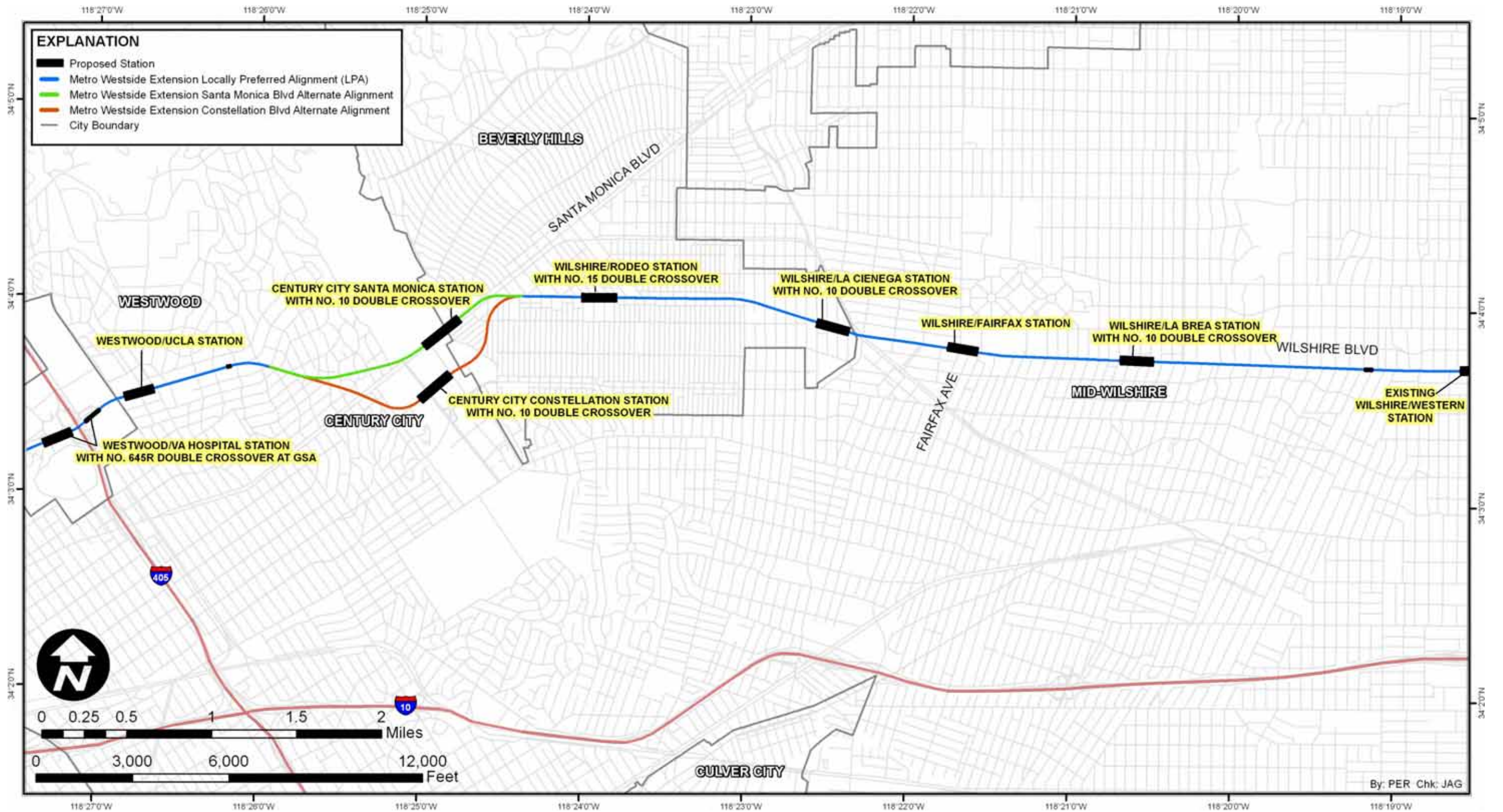
Figure 2-1: Tunnel Alignment
