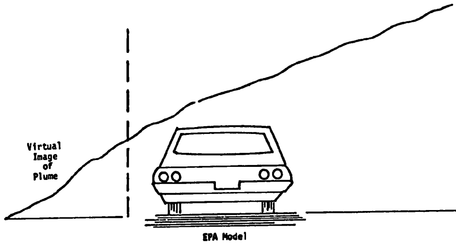
FIGURE VI-2 DISPERSION FROM VIRTUAL IMAGE (EPA MODEL) AND MIXING CELL (CALIFORNIA MODEL).
