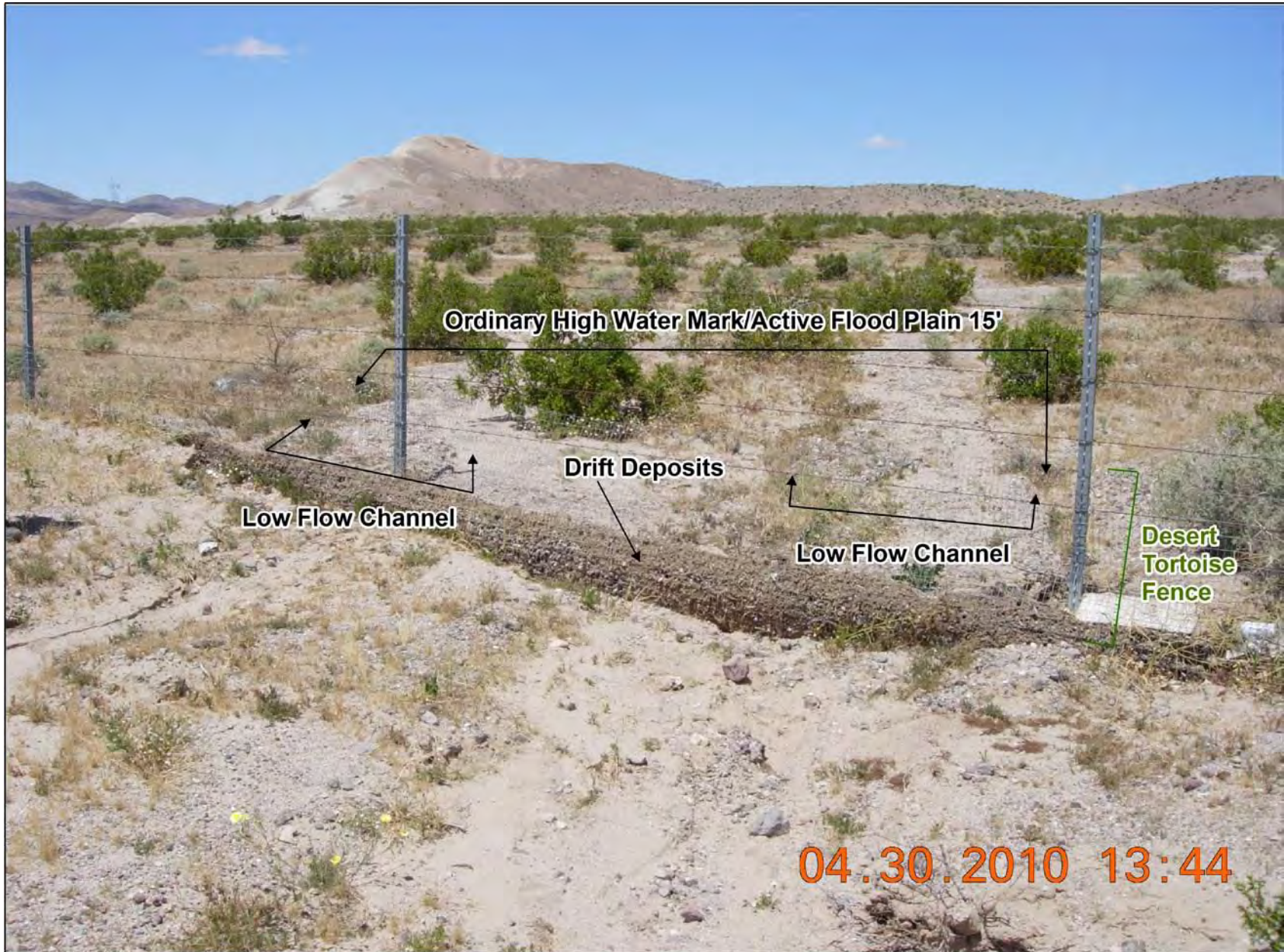
Exhibit A. Figure 11. Typical examples of field indicators of active surface water flow and Ordinary High Water Marks found within ephemerals drainages occurring within the DesertXpress Project Study Area. F-1.2-55
