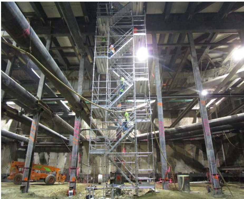
EXPOSITION STATION – Stair tower in operation.
