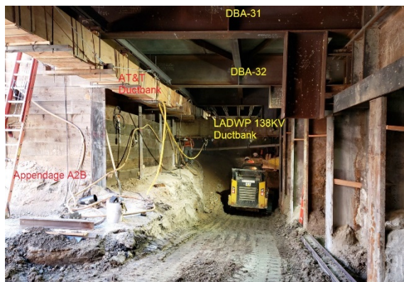
Excavating Emergency Exit at Wilshire/Fairfax Station
