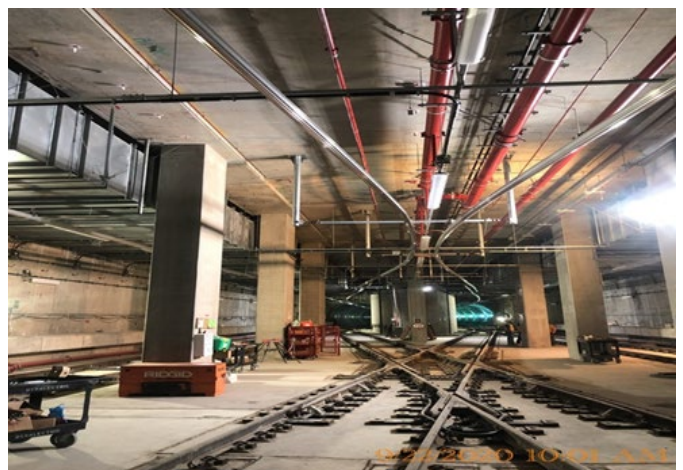
Expo/Crenshaw Station- Installing supports and fixtures for the crossover lighting at the invert level.
