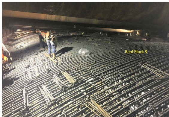
Roof Rebar Placement at Wilshire/Fairfax Station
