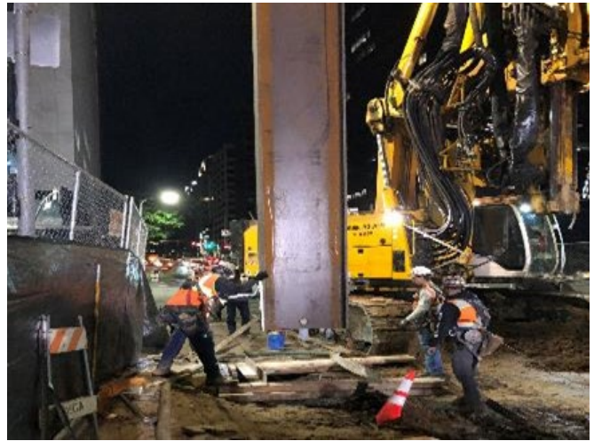
SOE Pile Installation North Side Wilshire Blvd.
