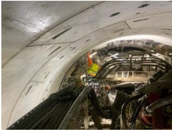
Ring Installation in the BL Tunnel
