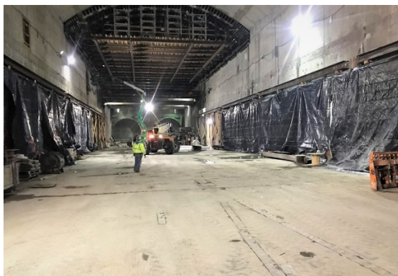
Track Level View of Wilshire/La Cienega Station
