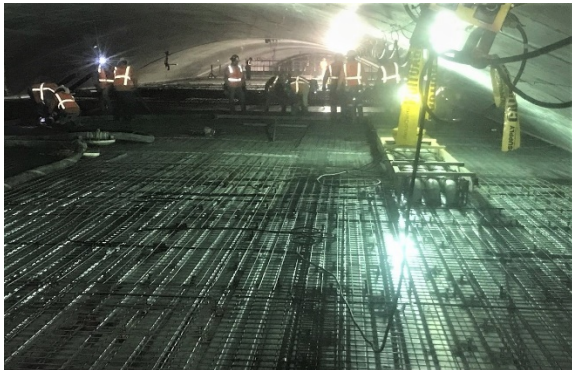
Plenum Concrete Placement at Wilshire/La Brea Station
