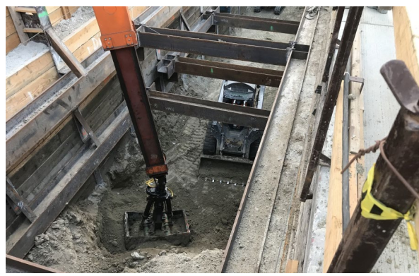
Appendage AE Excavation at Wilshire/La Cienega Station
