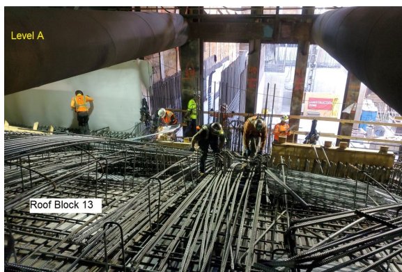
Roof Rebar Placement at Wilshire/Fairfax Station
