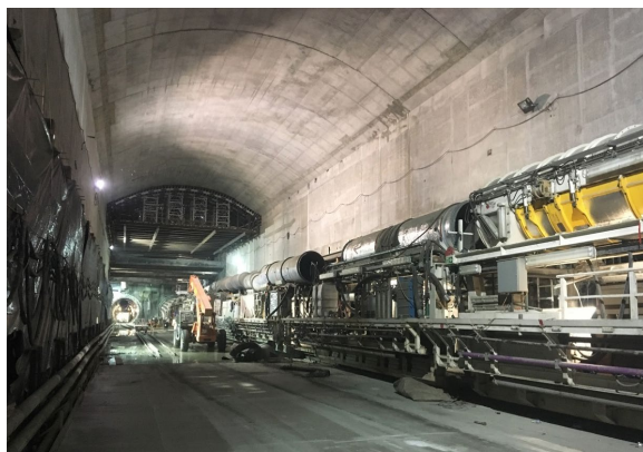
Removal of TBM Gantries at Wilshire/La Cienega Station
