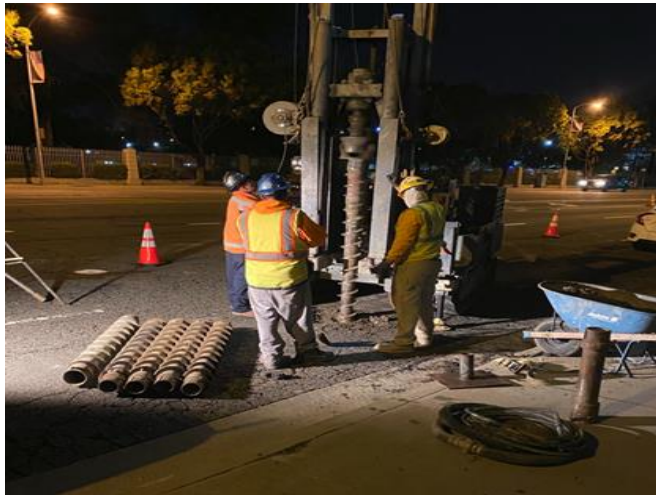
Instrumentation Installation on Wilshire at VA
