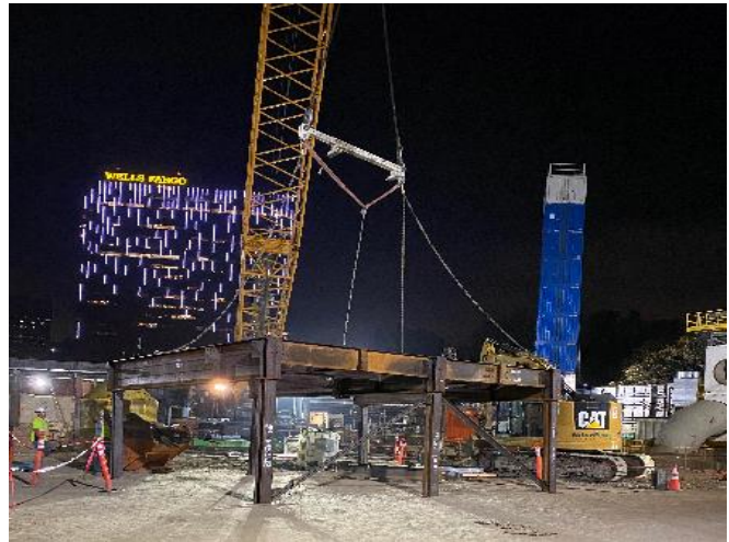
Deck Structure Assembly at Tail Track Exit Shaft
