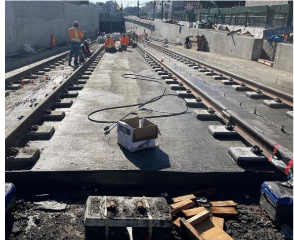
Alameda Leg embedded track concrete placement
