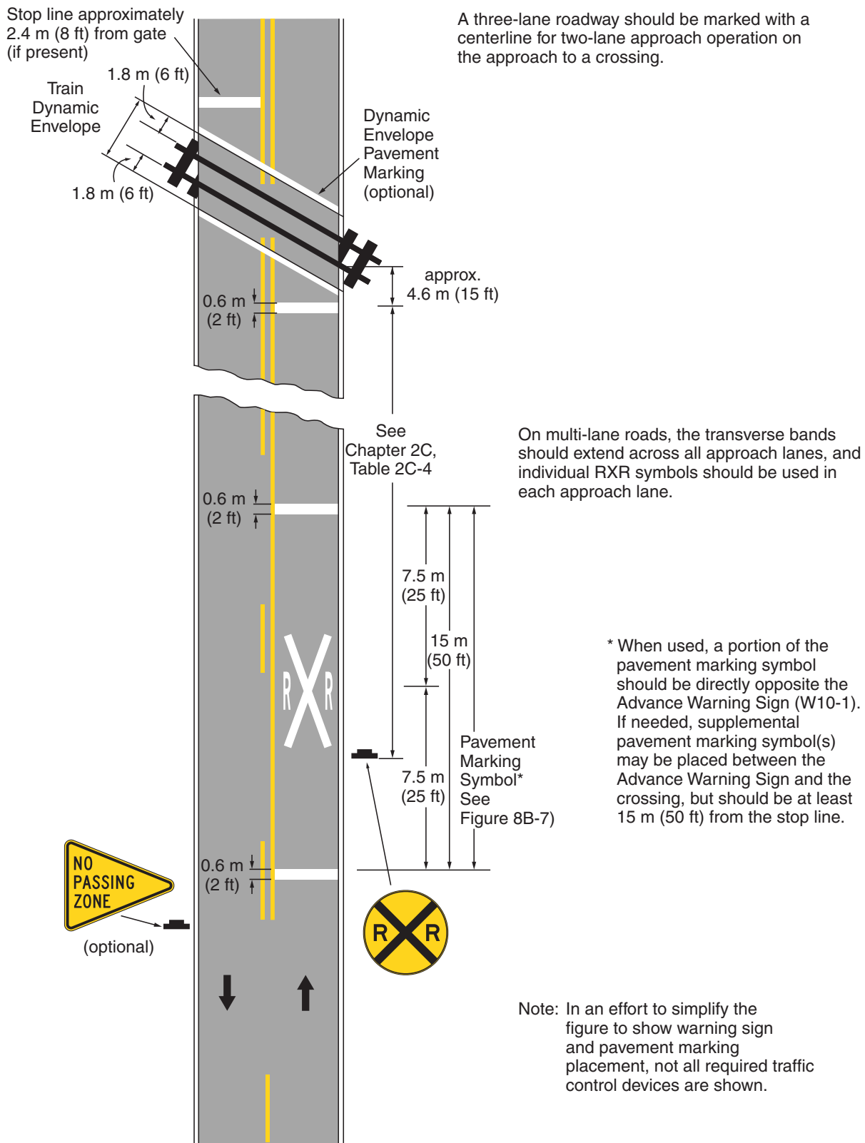
Figure 8B-6. Example of Placement of Warning Signs and Pavement Markings at Highway-Rail Grade Crossings
