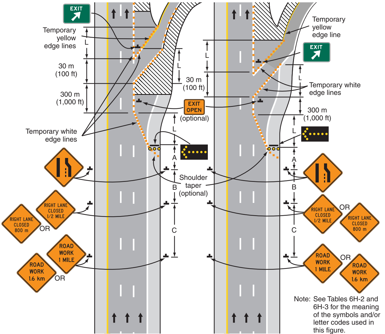
Typical Application 42
