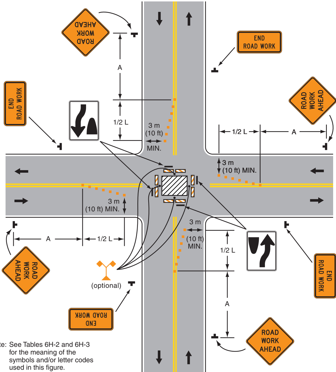
Typical Application 26
