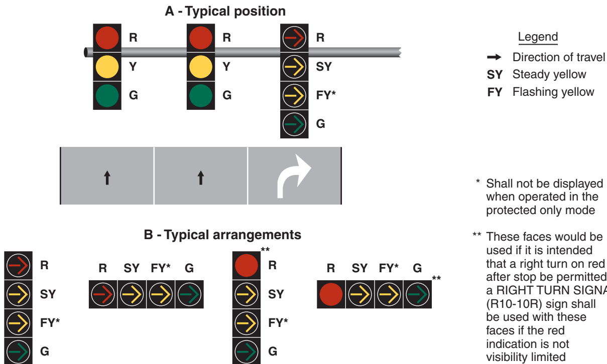
Figure 4D-19. Typical Position and Arrangements of Separate Signal Faces with Flashing Yellow Arrow for Protected/Permisive Mode and Protected Only Mode Right Turns
