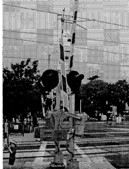
Exhibit 2 Large flasher mounted to pole adjacent to quad gate
