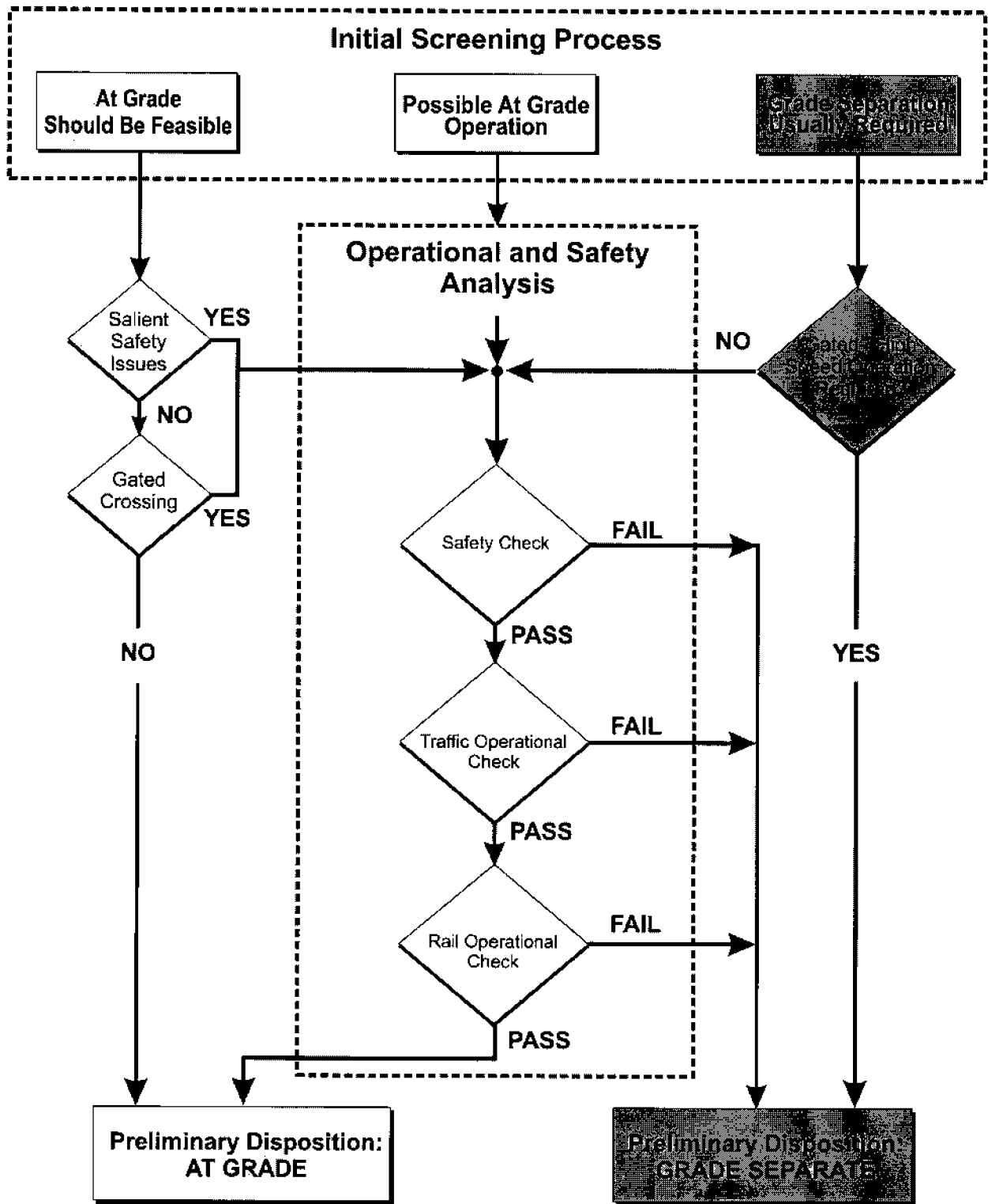
Figure 2 – Evaluation Flowchart
