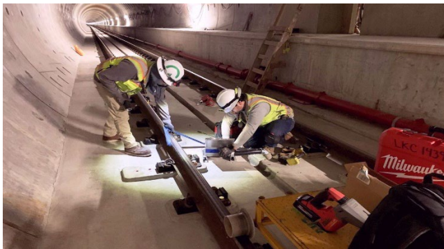
Reach 1 (BR) Train Control Installation
