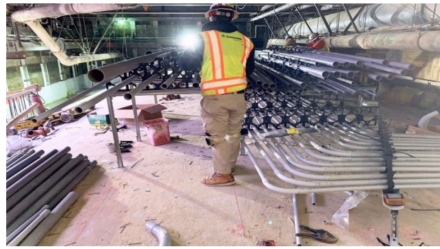
Above Roof Electrical Ductbank at Wilshire/La Cienega Station
