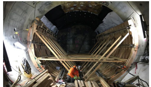
Reach 4 BL Tunnel Final Liner at TBM Shield
