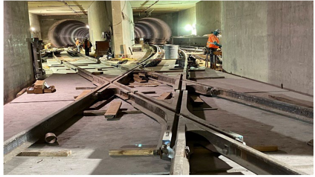
Track Crossover Diamond Placement at Wilshire/La Brea Station
