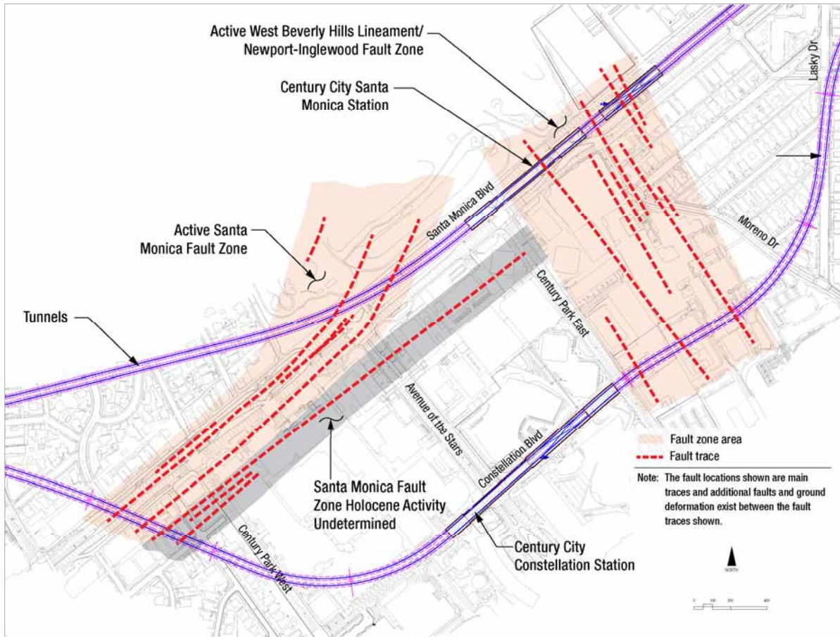
Figure 1: Fault Zone
