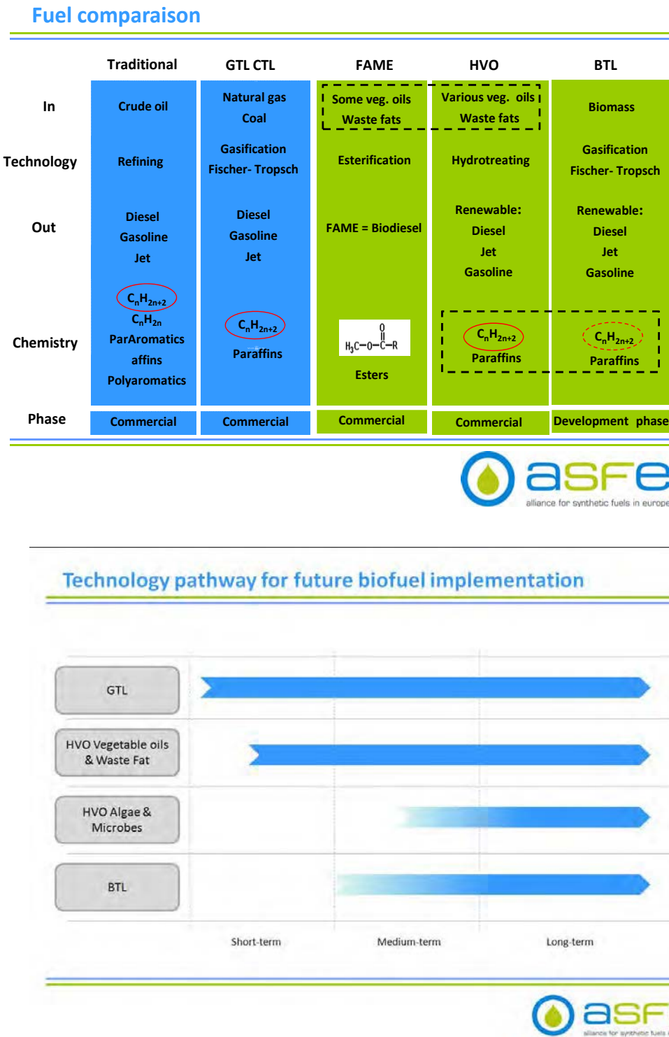
Fig. 8: Fuel comparison and technology pathways for future biofuel implementation (Source: ASFE)
