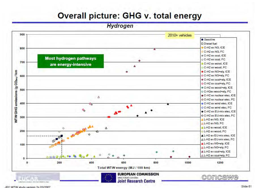
Fig. 9: CO 2 emissions versus energy consumption for hydrogen powered vehicles over the whole fuel chain for different hydrogen production pathways (JEC Well-To-Wheels study, Version 2c, March 2007)
