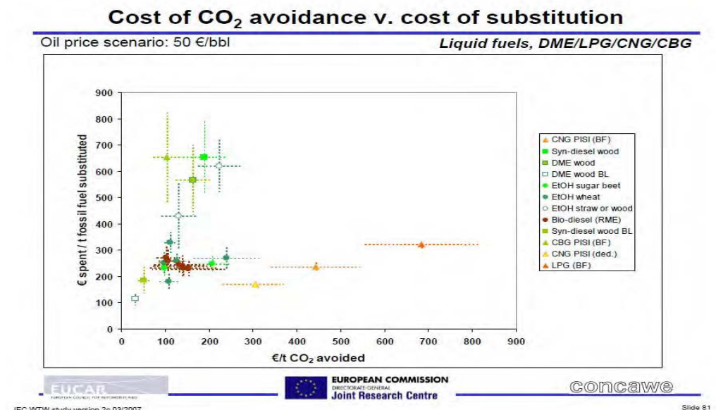
Fig. 13: Cost of oil substitution versus cost of CO 2 emissions reduction for different alternative fuel pathways, over the whole fuel chain (JEC Well-To-Wheels study)
