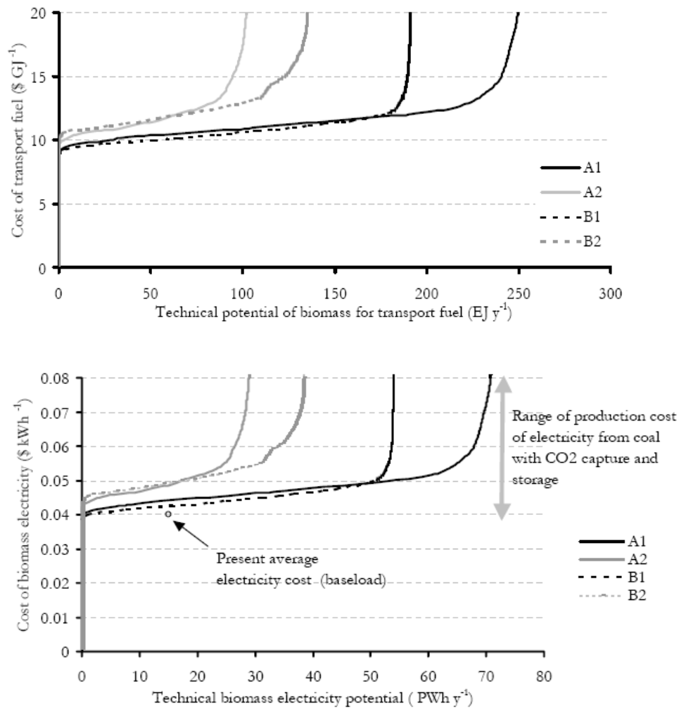
Fig. 7: Cost-supply curve for biomass based liquid fuel (synthetic FT diesel), using energy crop produced on abandoned agricultural land and rest land as feedstock, globally for 2050.
