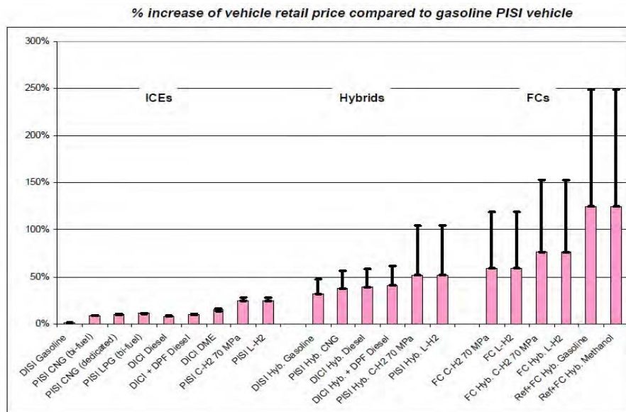
Figure 12: Relative increase of the vehicle retail price for different fuel and vehicle technologies, compared to a gasoline powered vehicle (JEC Well-To-Wheels study 2008)
