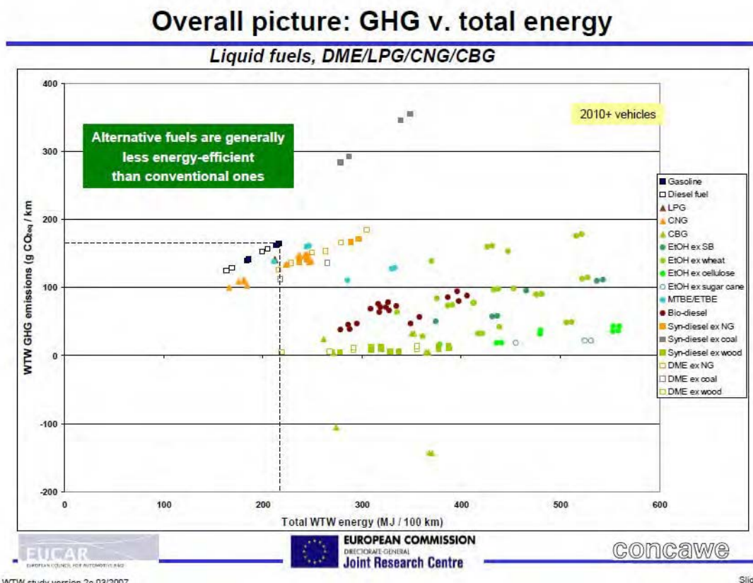
Fig. 10: CO 2 emissions versus energy consumption over the whole fuel chain for different alternative fuel pathways (JEC Well-To-Wheels study, Version 2c, March 2007)
