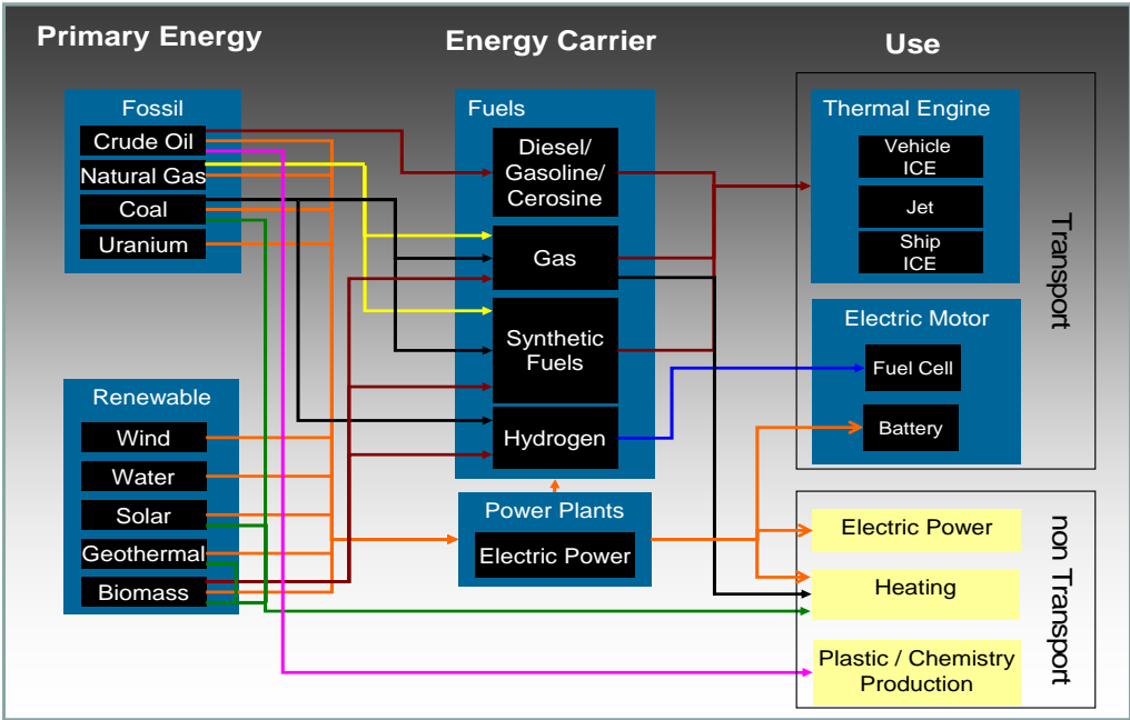
Figure 4: Energy pathways in transport and other sectors (Source: ERTRAC)
