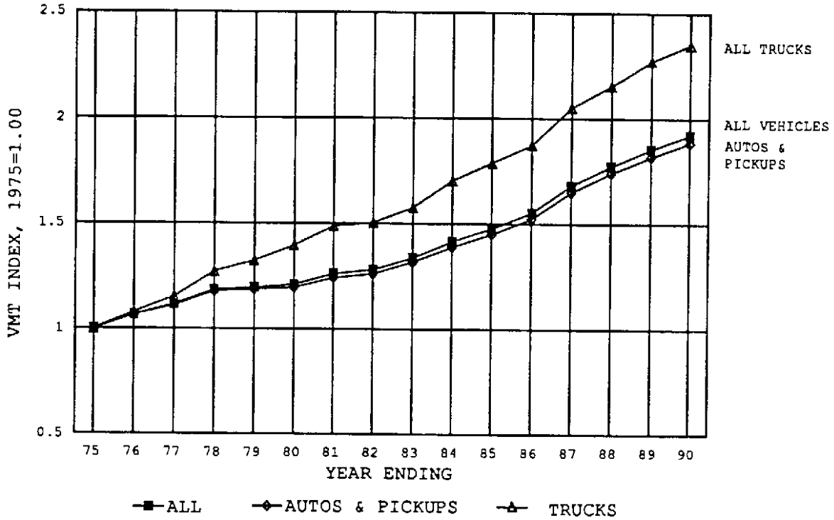
Figure A-2 VEHICLE MILES OF TRAVEL INDEX BY VEHICLE TYPE For the California State Highway System, 1975=1.00
