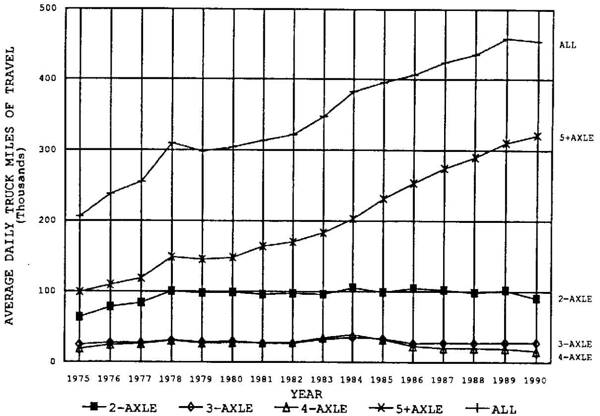
DISTRICT 9 - AVERAGE DAILY TRUCK MILES OF TRAVEL -----BY AXLE GROUP-----
