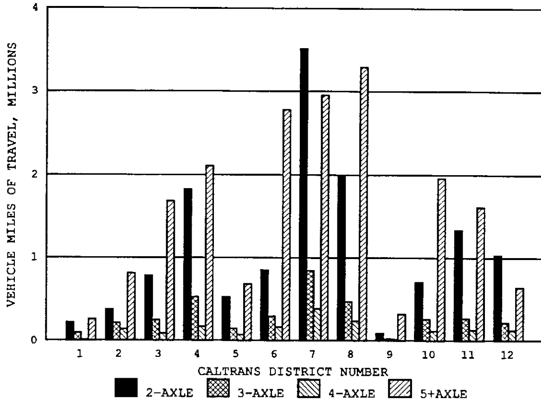
DAILY TRUCK MILES OF TRAVEL BY DISTRICT -----IN MILLIONS-----
