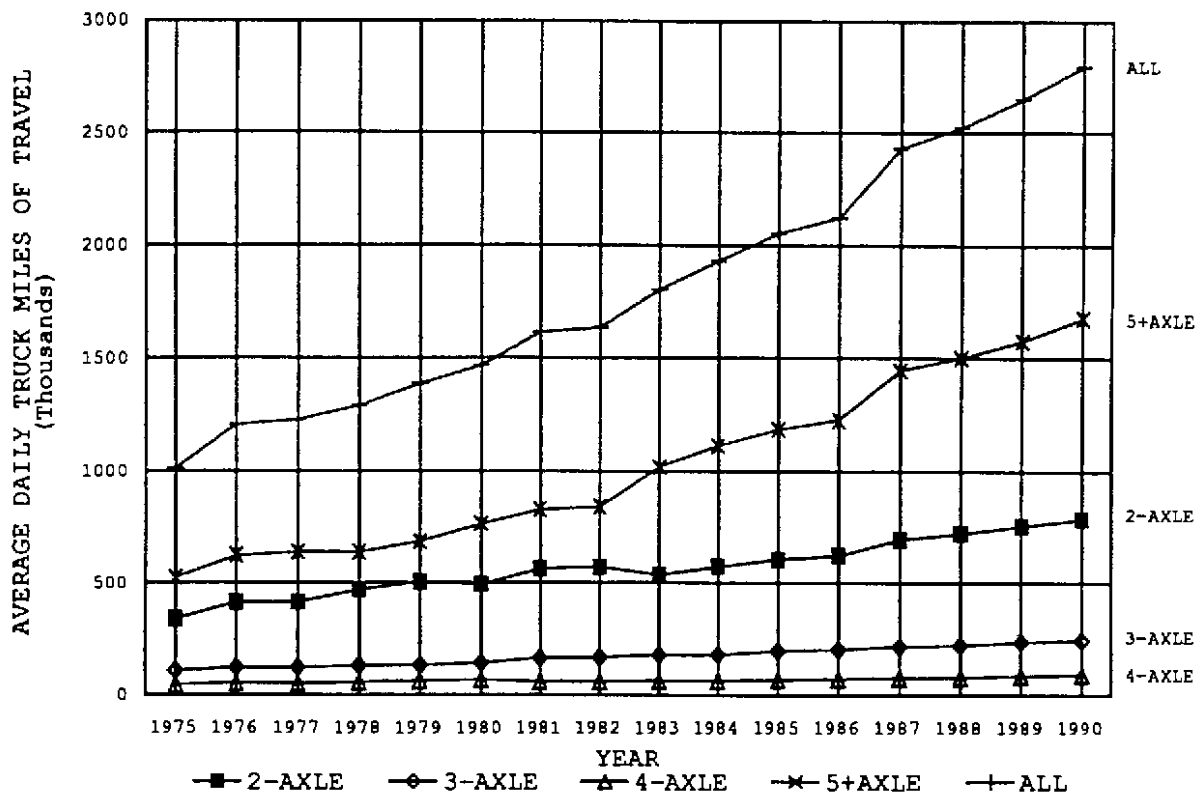
DISTRICT 3 - AVERAGE DAILY TRUCK MILES OF TRAVEL -----BY AXLE GROUP-----
