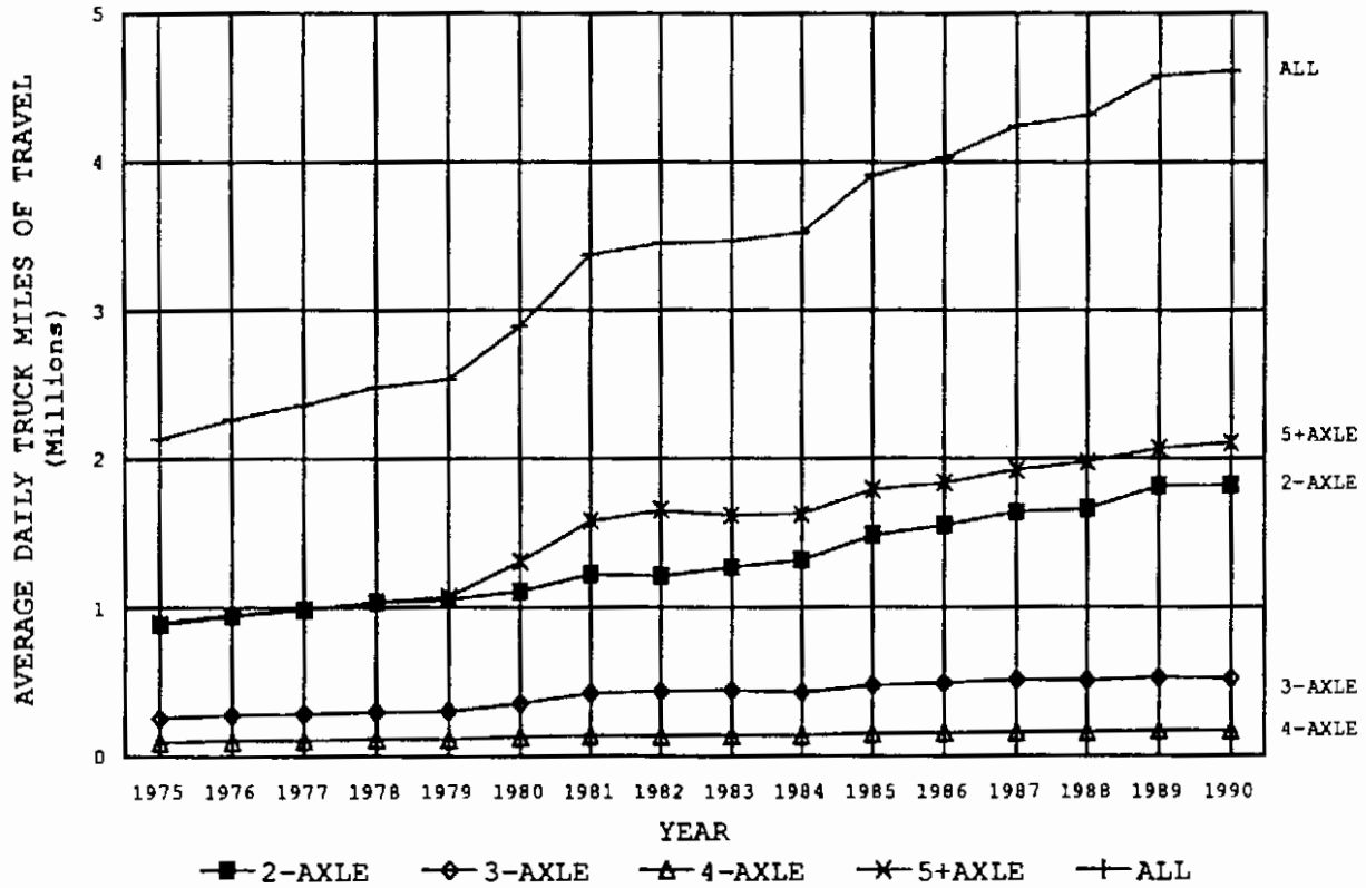
DISTRICT 4 - AVERAGE DAILY TRUCK MILES OF TRAVEL -----BY AXLE GROUP-----
