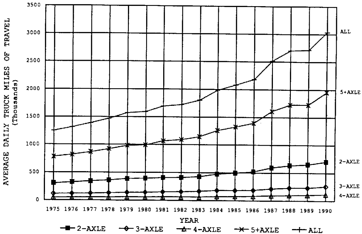
DISTRICT 10 - AVERAGE DAILY TRUCK MILES OF TRAVEL -----BY AXLE GROUP-----
