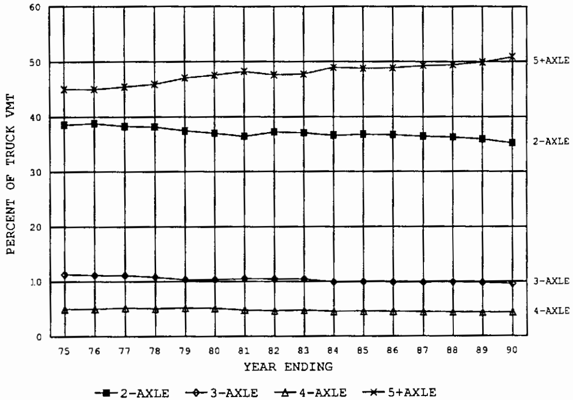
PERCENT TRUCK VMT BY AXLE GROUP
