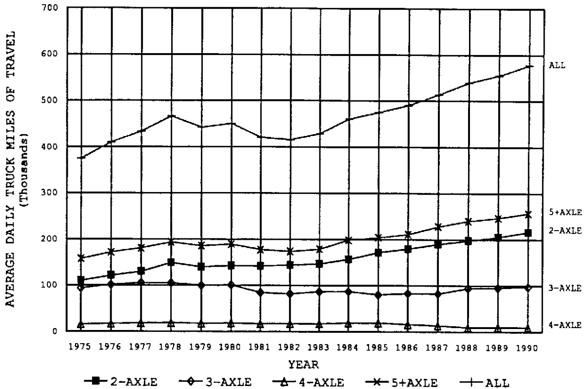
DISTRICT 1 - AVERAGE DAILY TRUCK MILES OF TRAVEL -----BY AXLE GROUP-----
