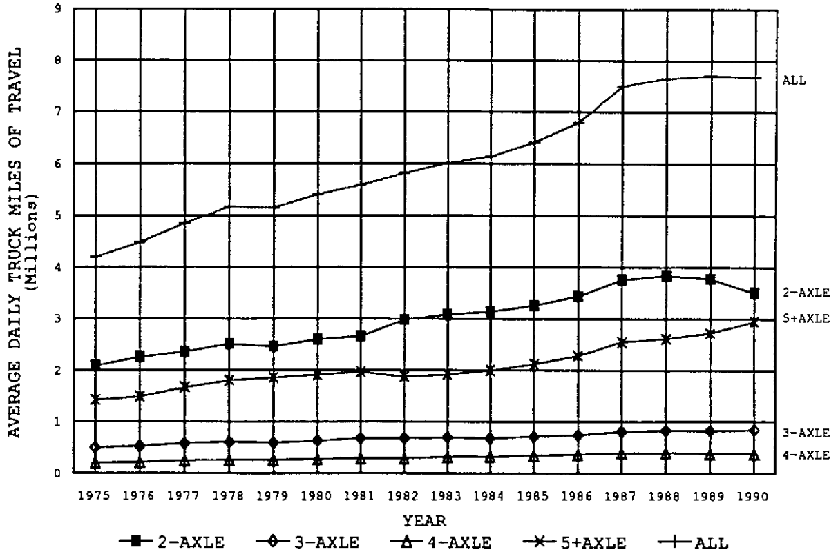
DISTRICT 7 - AVERAGE DAILY TRUCK MILES OF TRAVEL -----BY AXLE GROUP-----
