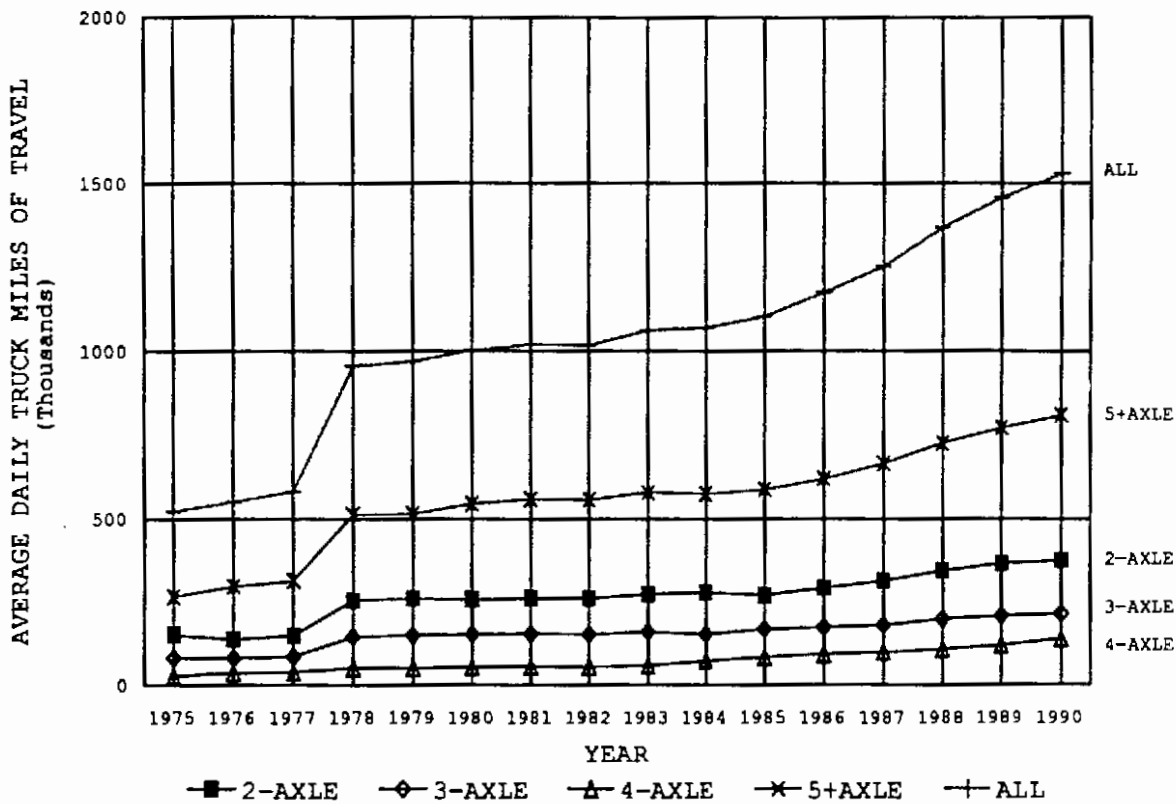
DISTRICT 2 - AVERAGE DAILY TRUCK MILES OF TRAVEL -----BY AXLE GROUP-----
