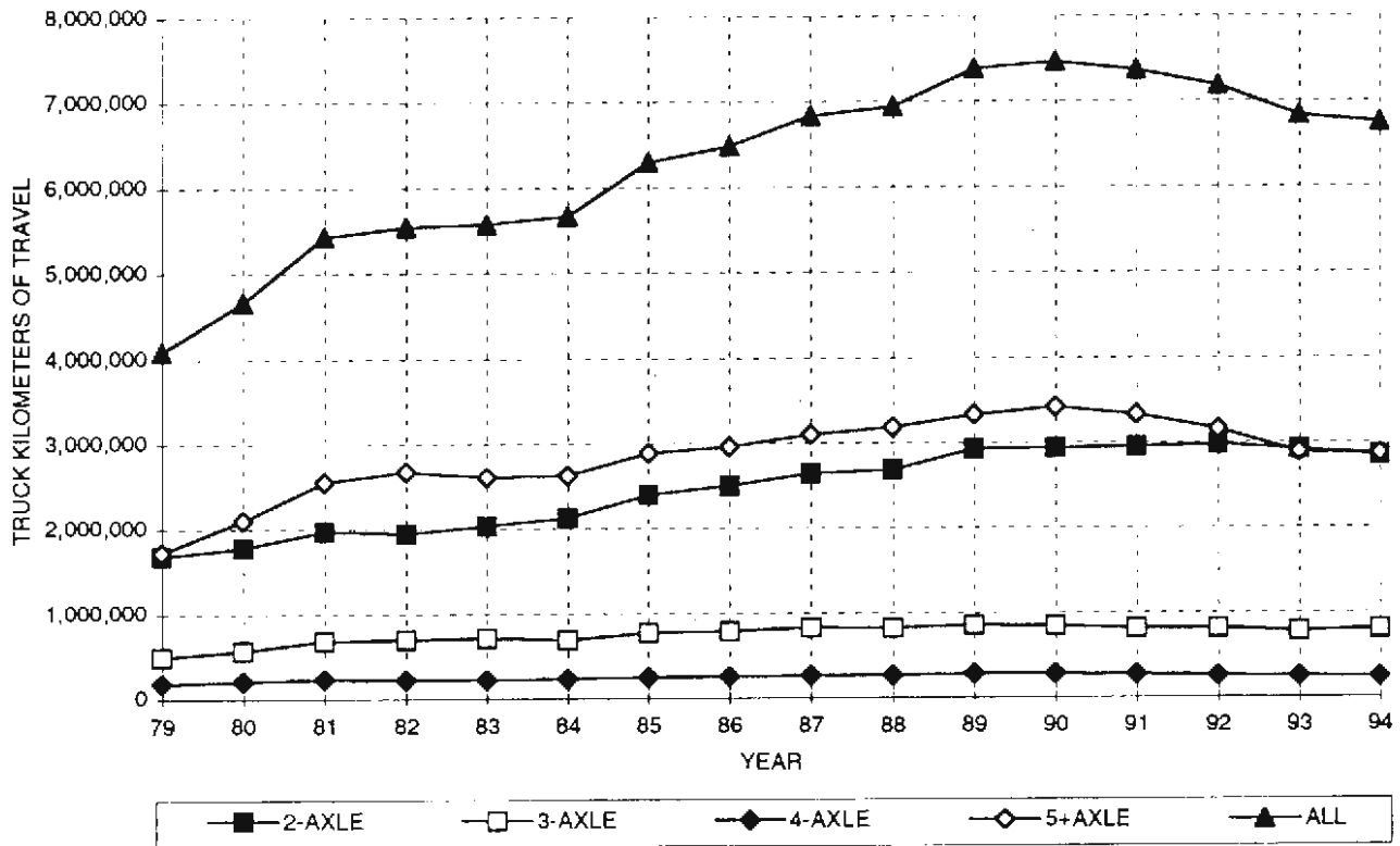
DISTRICT 4 - AVERAGE DAILY TRUCK KILOMETERS OF TRAVEL BY AXLE GROUP
