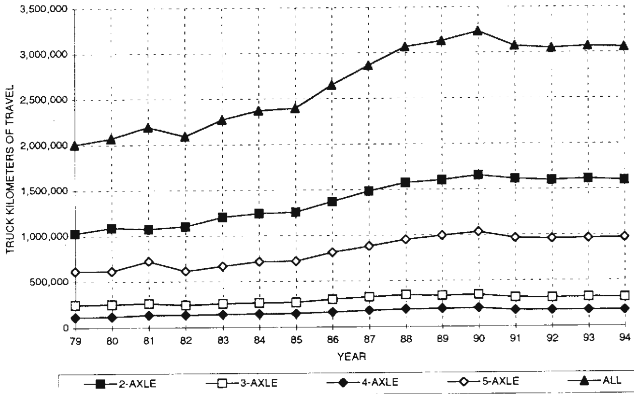
DISTRICT 12 - AVERAGE DAILY TRUCK KILOMETERS OF TRAVEL BY AXLE GROUP
