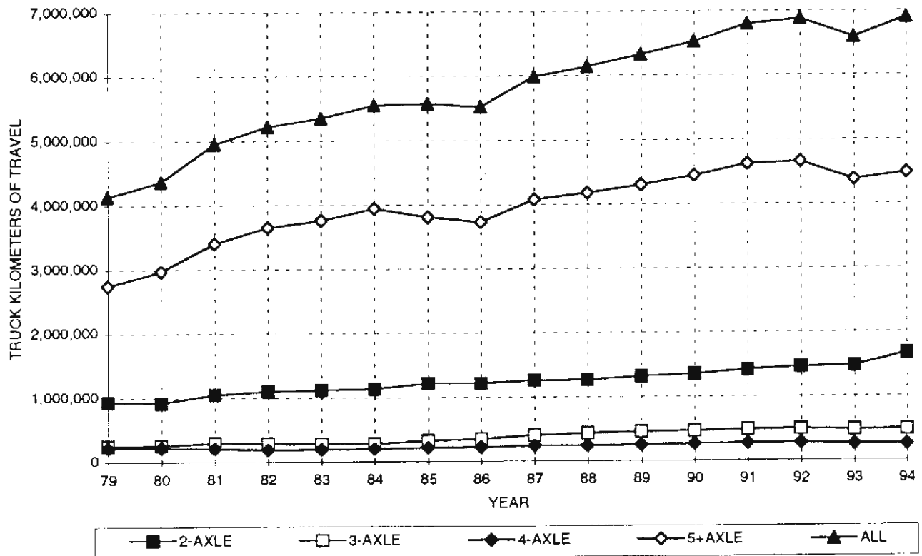
DISTRICT 6 - AVERAGE DAILY TRUCK KILOMETERS OF TRAVEL BY AXLE GROUP
