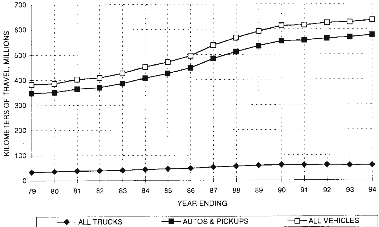
FIGURE A-1 AVERAGE DAILY VEHICLE KILOMETERS OF TRAVEL BY VEHICLE TYPE On the California State Highway System
