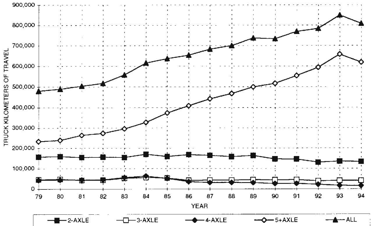
DISTRICT 9 - AVERAGE DAILY TRUCK KILOMETERS OF TRAVEL BY AXLE GROUP
