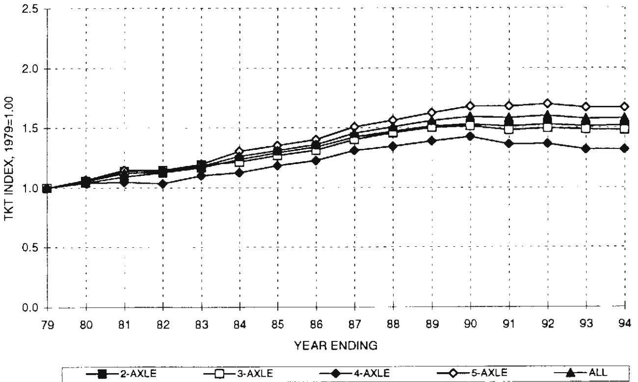
FIGURE A-6 TRUCK KILOMETERS OF TRAVEL INDEX BY AXLE GROUP On the California State Highway System, 1979=1.00
