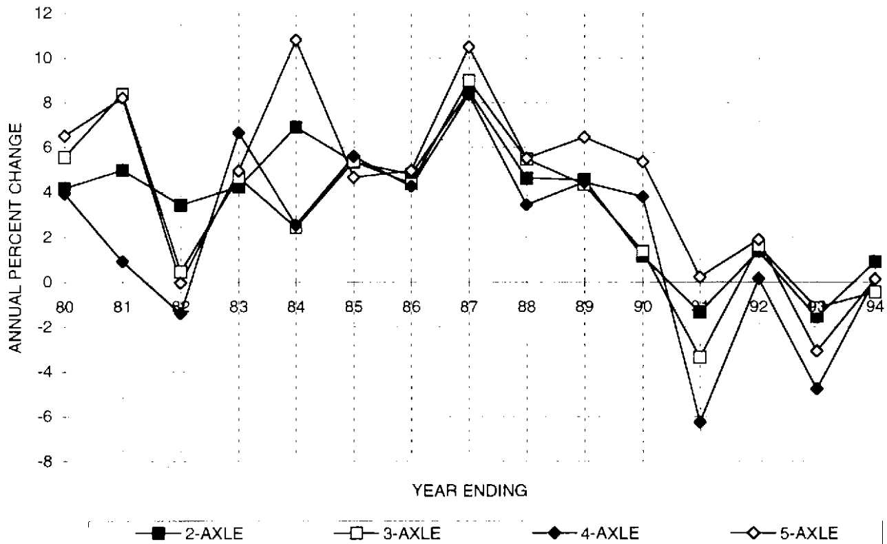
ANNUAL PERCENT CHANGE IN TRUCK KILOMETERS OF TRAVEL
