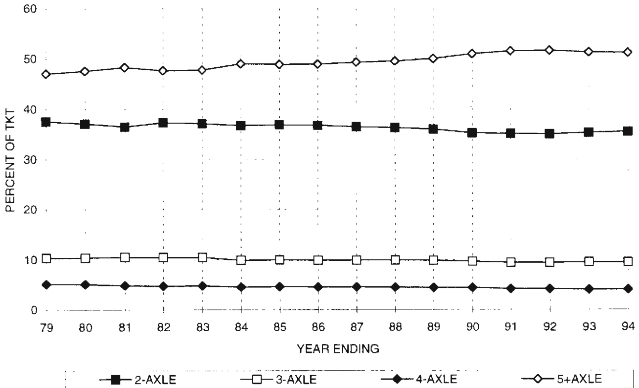
PERCENT OF TRUCK KILOMETERS OF TRAVEL BY AXLE GROUP
