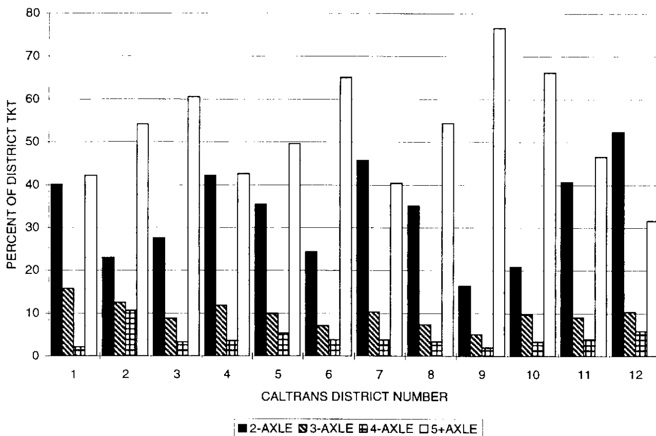
FIGURE B-6 PERCENT OF 1994 TRUCK KILOMETERS OF TRAVEL ACROSS AXLE GROUPS BY DISTRICT
