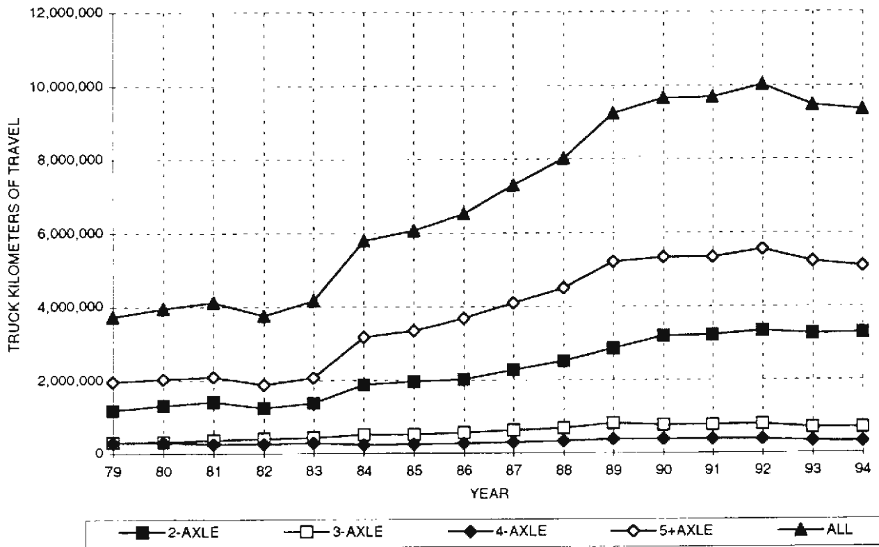
DISTRICT 8 - AVERAGE DAILY TRUCK KILOMETERS OF TRAVEL BY AXLE GROUP
