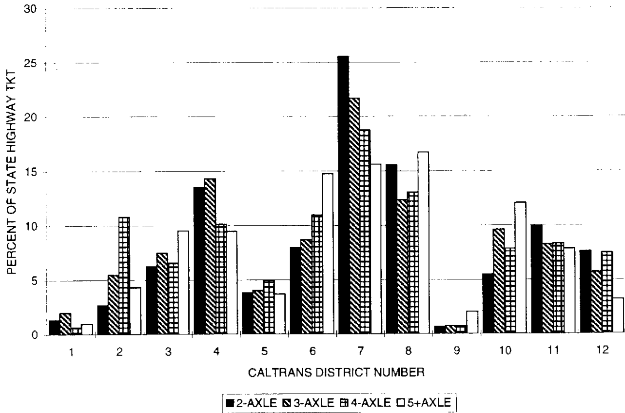
FIGURE B-5 PERCENT OF 1994 TRUCK KILOMETERS OF TRAVEL ACROSS DISTRICTS BY AXLE GROUP
