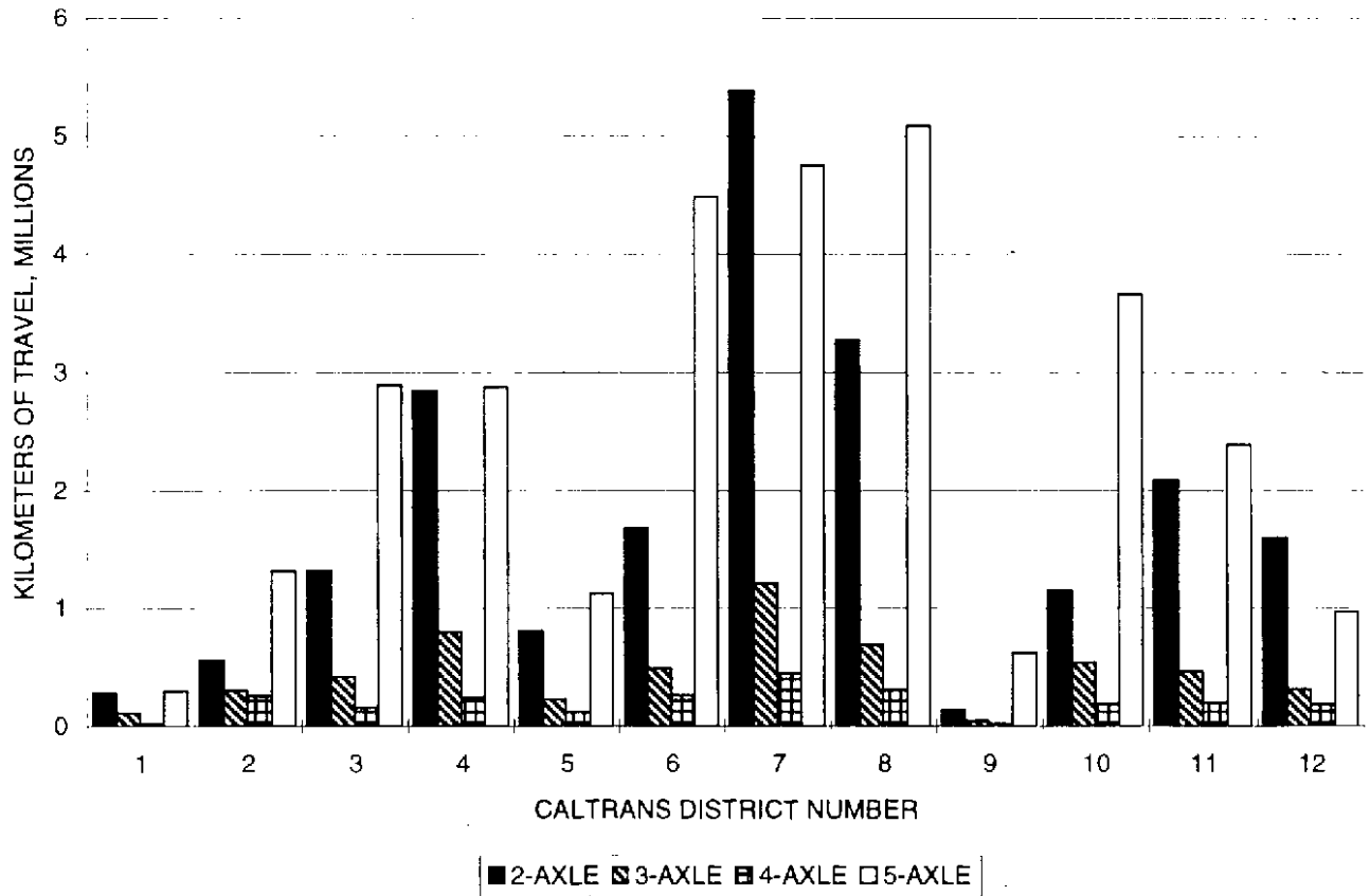
FIGURE B-4 1994 DAILY TRUCK KILOMETERS OF TRAVEL BY DISTRICT AND AXLE GROUP
