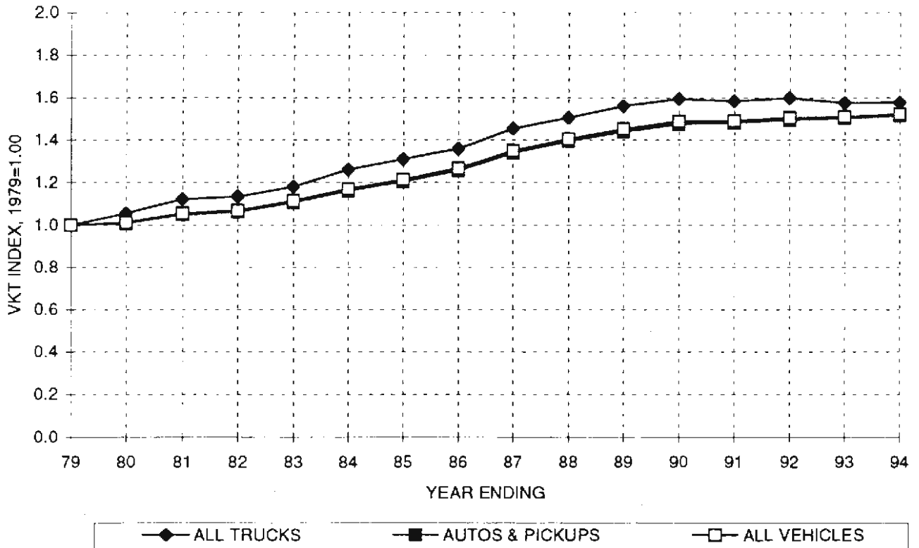
FIGURE A-2 VEHICLE KILOMETERS OF TRAVEL INDEX BY VEHICLE TYPE On the California State Highway System, 1979=1.00
