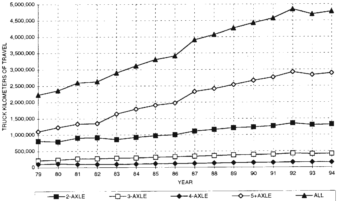
DISTRICT 3 - AVERAGE DAILY TRUCK KILOMETERS OF TRAVEL BY AXLE GROUP
