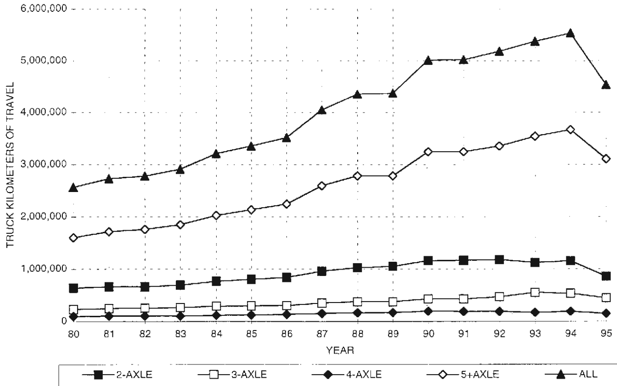
DISTRICT 10 - AVERAGE DAILY TRUCK KILOMETERS OF TRAVEL BY AXLE GROUP
