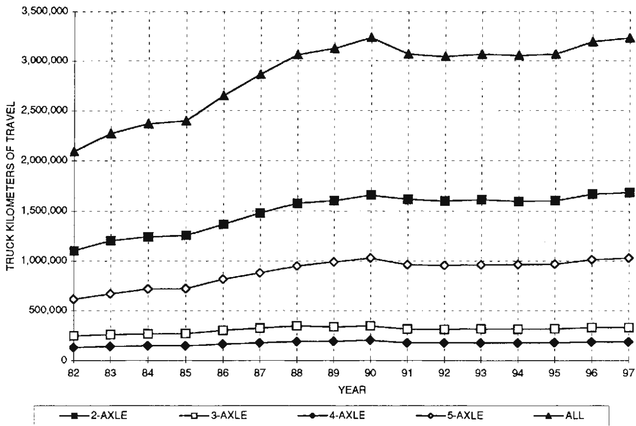
FIGURE B-18 DISTRICT 12-AVERAGE DAILY TRUCK KILOMETERS OF TRAVEL BY AXLE GROUP
