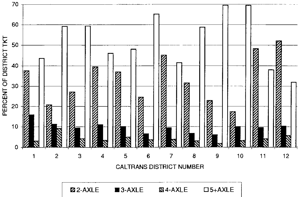
FIGURE B-6 PERCENT OF 1997 TRUCK KILOMETERS OF TRAVEL ACROSS AXLE GROUPS BY DISTRICT
