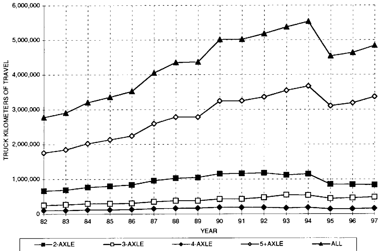
FIGURE B-16 DISTRICT 10-AVERAGE DAILY TRUCK KILOMETERS OF TRAVEL BY AXLE GROUP
