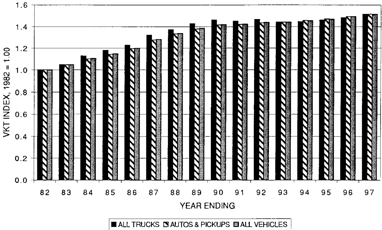
FIGURE A-2 VEHICLE KILOMETERS OF TRAVEL INDEX BY VEHICLE TYPE On the California State Highway System, 1982=1.00
