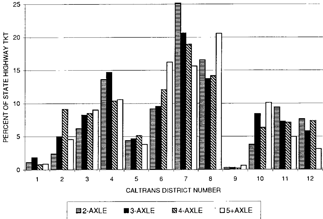
FIGURE B-5 PERCENT OF 1997 TRUCK KILOMETERS OF TRAVEL ACROSS DISTRICTS BY AXLE GROUP
