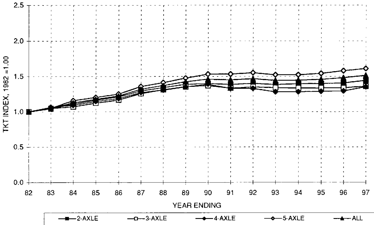
FIGURE A-6 TRUCK KILOMETERS OF TRAVEL INDEX BY AXLE GROUP On the California State Highway System, 1982 = 1.00
