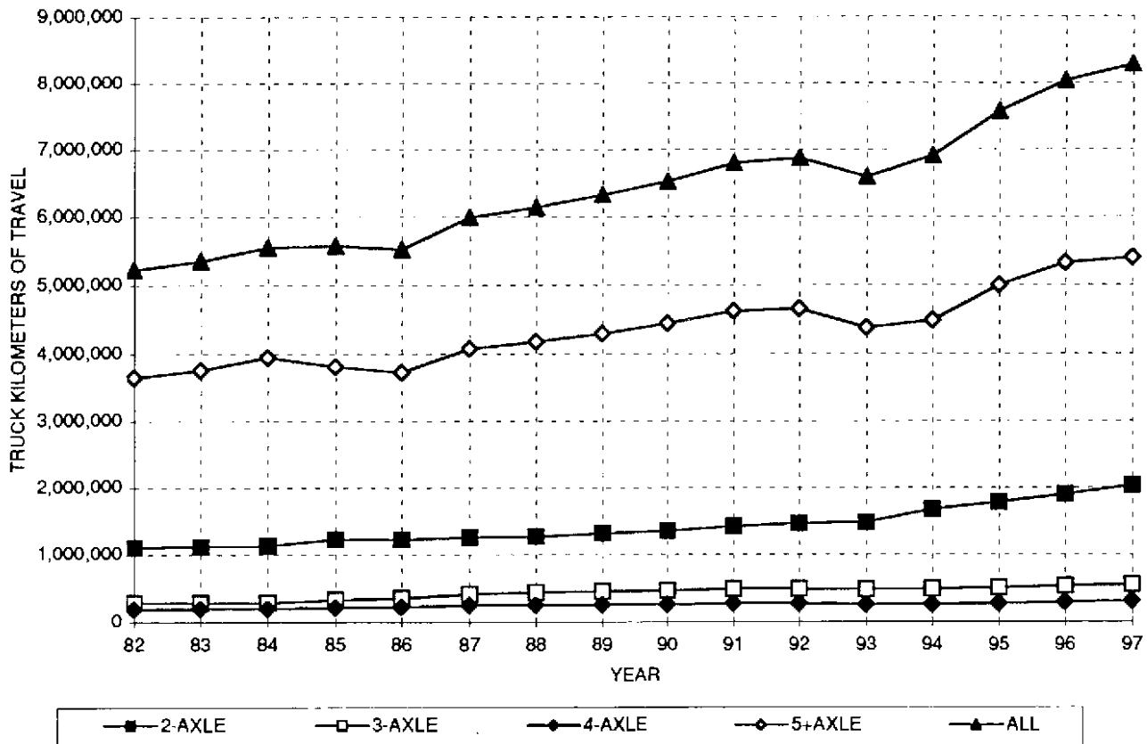
FIGURE B-12 DISTRICT 6-AVERAGE DAILY TRUCK KILOMETERS OF TRAVEL BY AXLE GROUP
