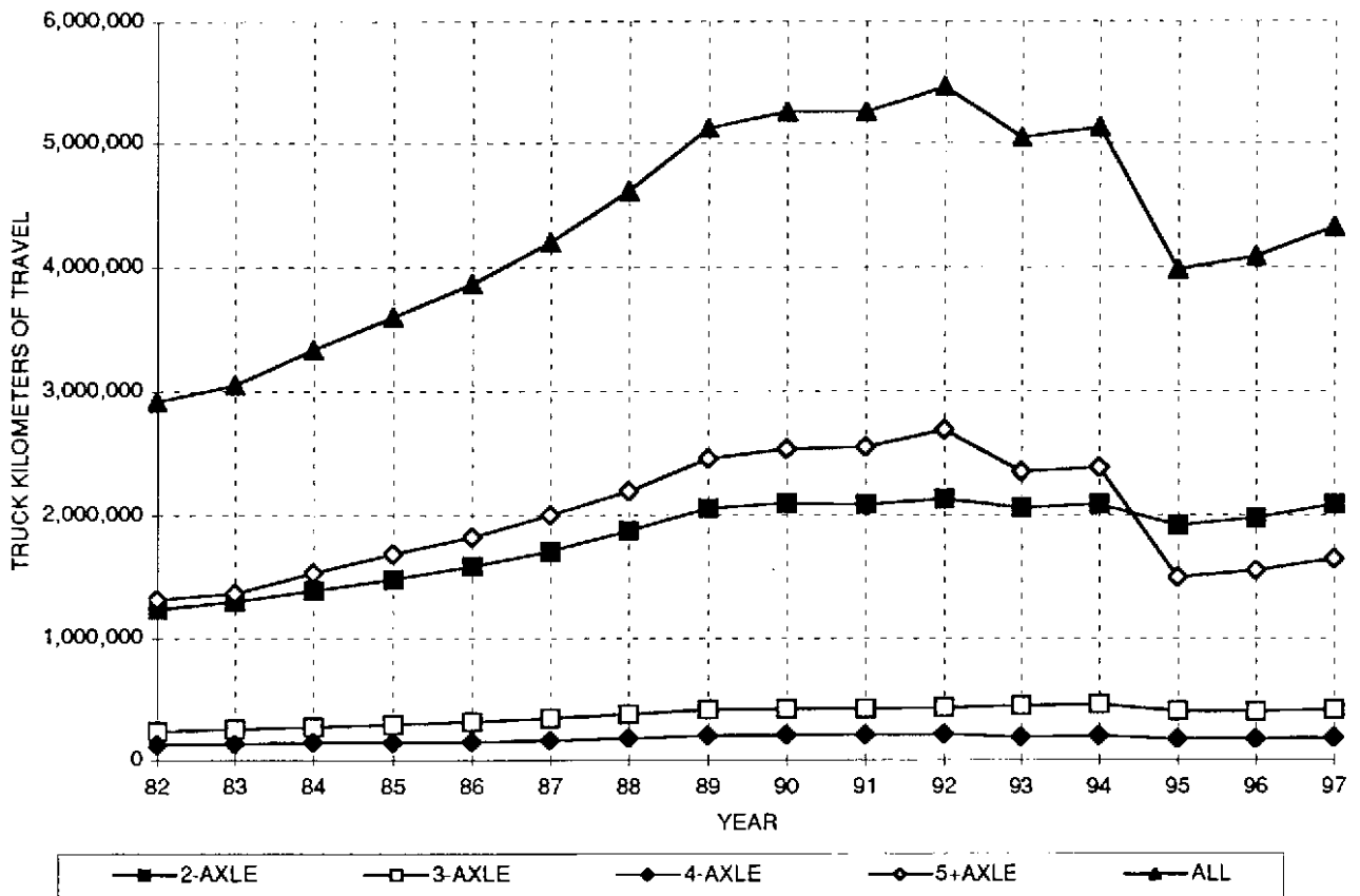
FIGURE B-17 DISTRICT 11-AVERAGE DAILY TRUCK KILOMETERS OF TRAVEL BY AXLE GROUP
