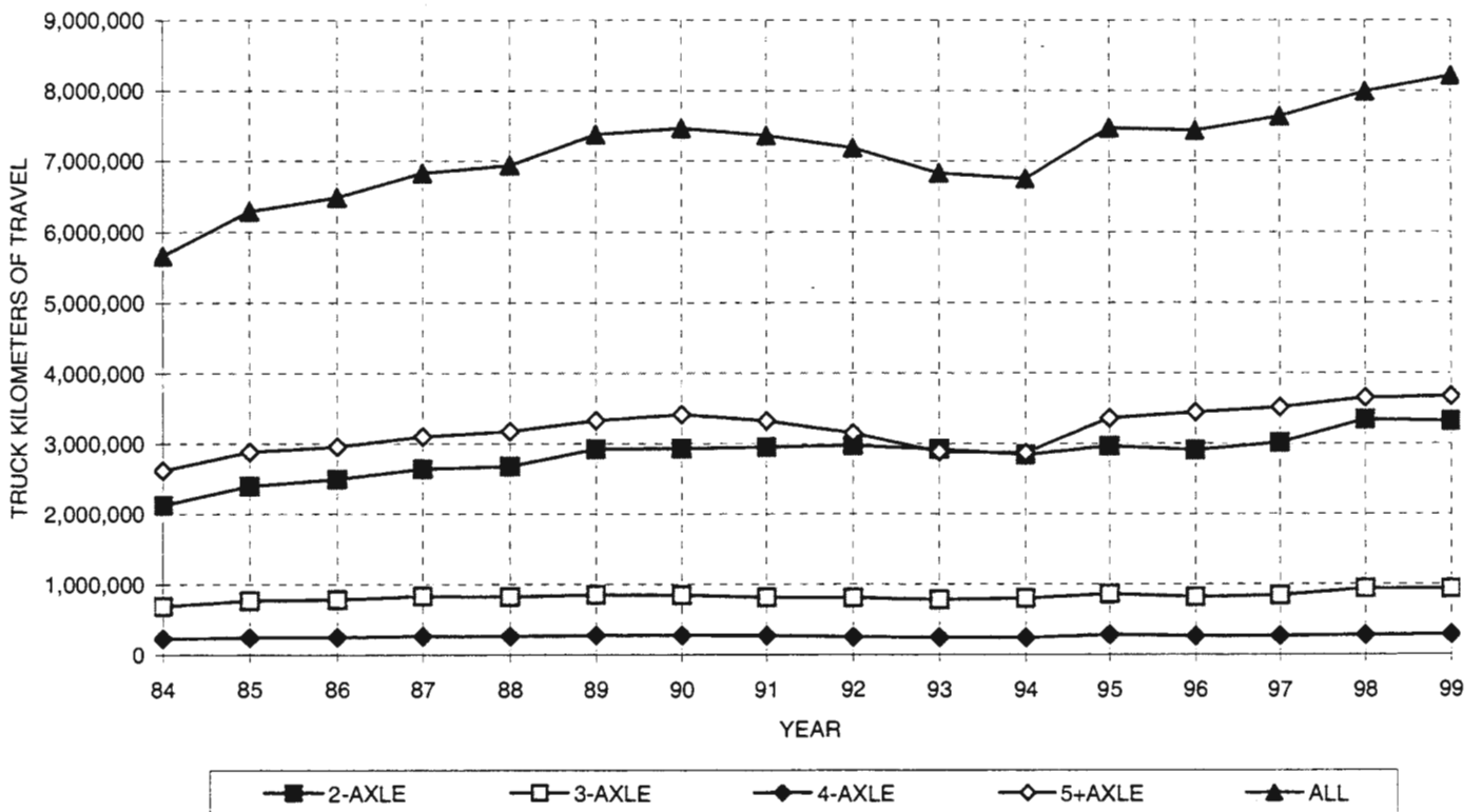
DISTRICT 4 - AVERAGE DAILY TRUCK KILOMETERS OF TRAVEL BY AXLE GROUP
