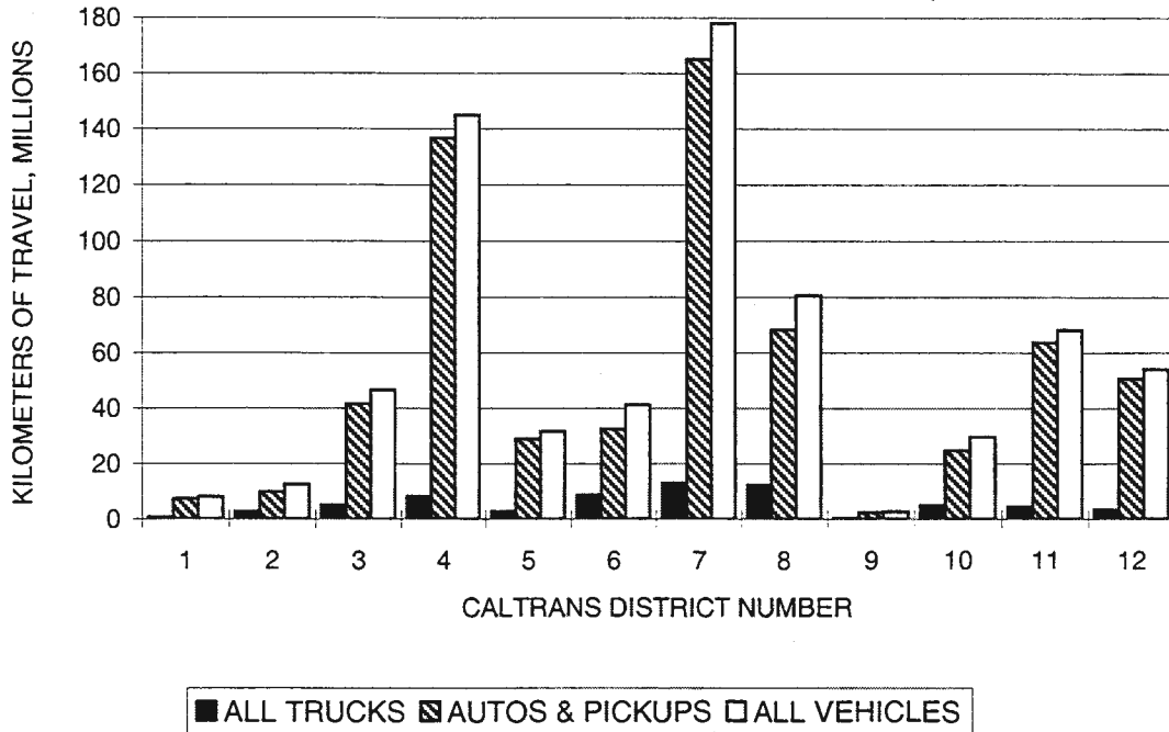
FIGURE B-2 1999 DAILY VEHICLE KILOMETERS OF TRAVEL BY DISTRICT AND VEHICLE TYPE
