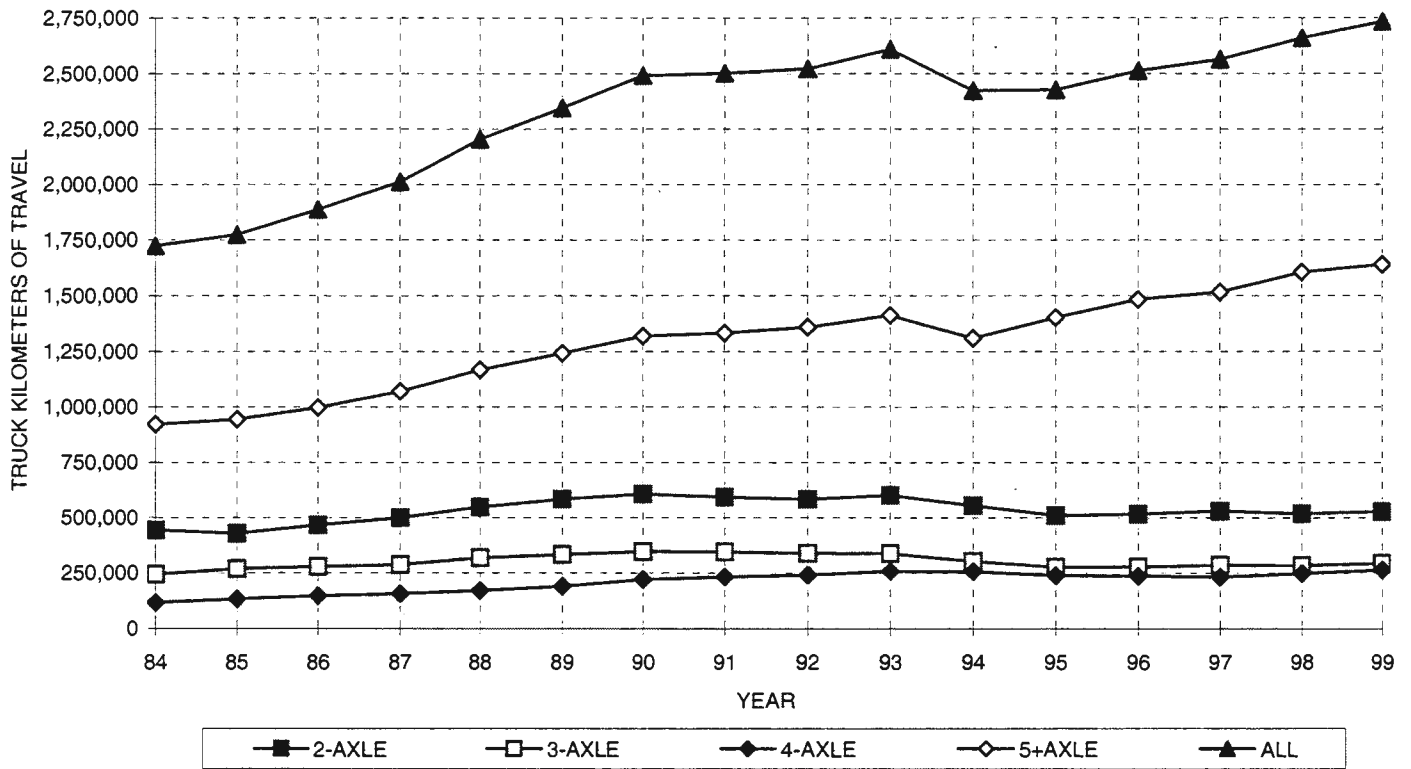
DISTRICT 2 - AVERAGE DAILY TRUCK KILOMETERS OF TRAVEL BY AXLE GROUP
