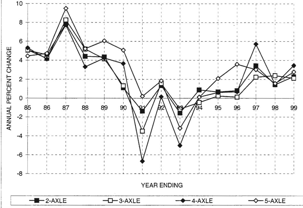
FIGURE A-7 ANNUAL % CHANGE IN TRUCK KILOMETERS OF TRAVEL BY AXLE GROUP On the California State Highway System
