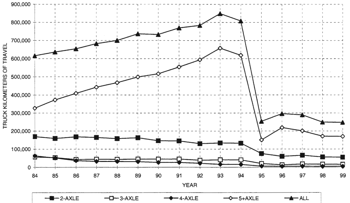
DISTRICT 9 - AVERAGE DAILY TRUCK KILOMETERS OF TRAVEL BY AXLE GROUP
