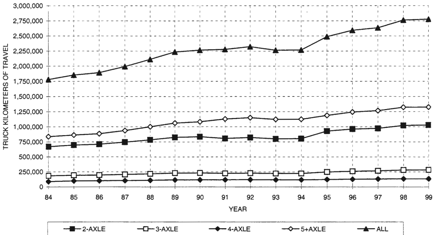
DISTRICT 5 - AVERAGE DAILY TRUCK KILOMETERS OF TRAVEL BY AXLE GROUP
