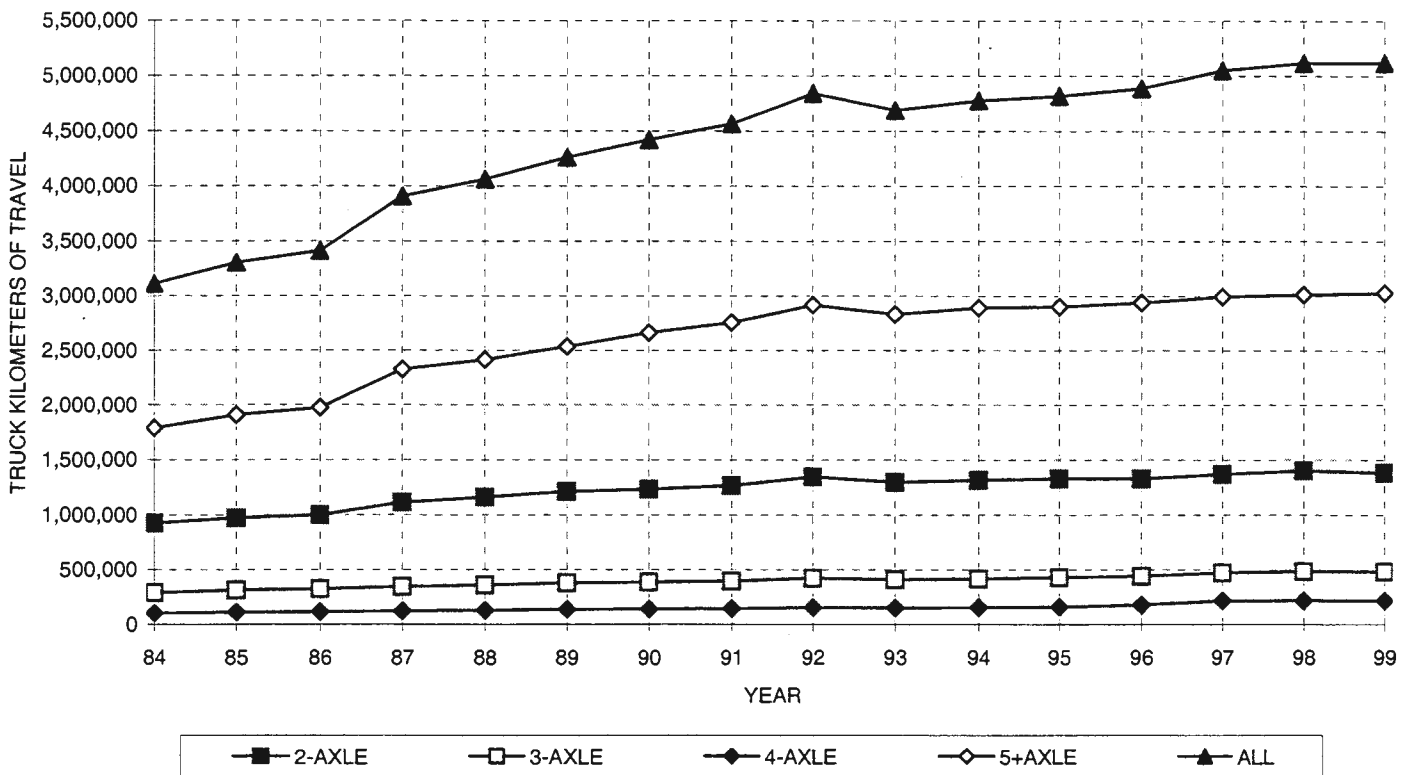
DISTRICT 3 - AVERAGE DAILY TRUCK KILOMETERS OF TRAVEL BY AXLE GROUP
