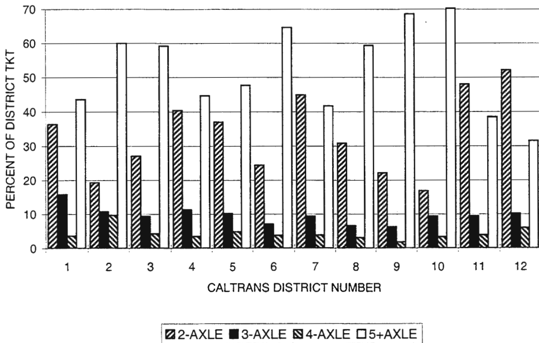
FIGURE B-6 PERCENT OF 1999 TRUCK KILOMETERS OF TRAVEL ACROSS AXLE GROUPS BY DISTRICT
