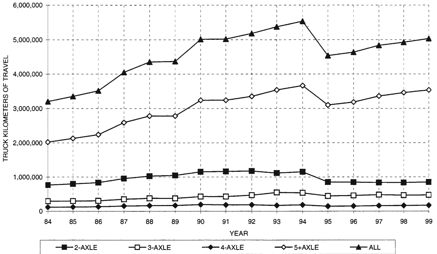
DISTRICT 10 - AVERAGE DAILY TRUCK KILOMETERS OF TRAVEL BY AXLE GROUP
