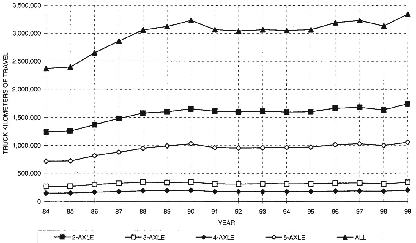
DISTRICT 12 - AVERAGE DAILY TRUCK KILOMETERS OF TRAVEL BY AXLE GROUP
