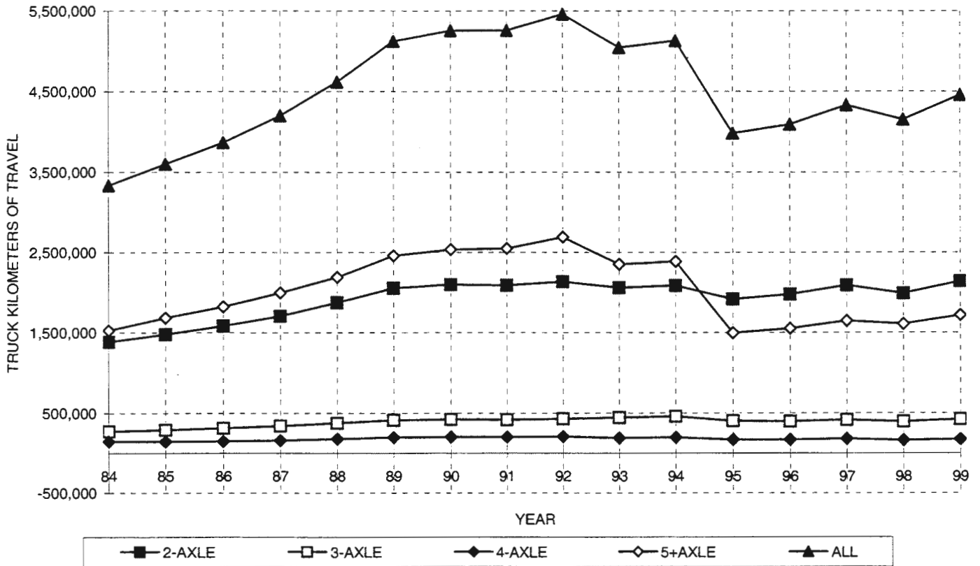
DISTRICT 11 - AVERAGE DAILY TRUCK KILOMETERS OF TRAVEL BY AXLE GROUP
