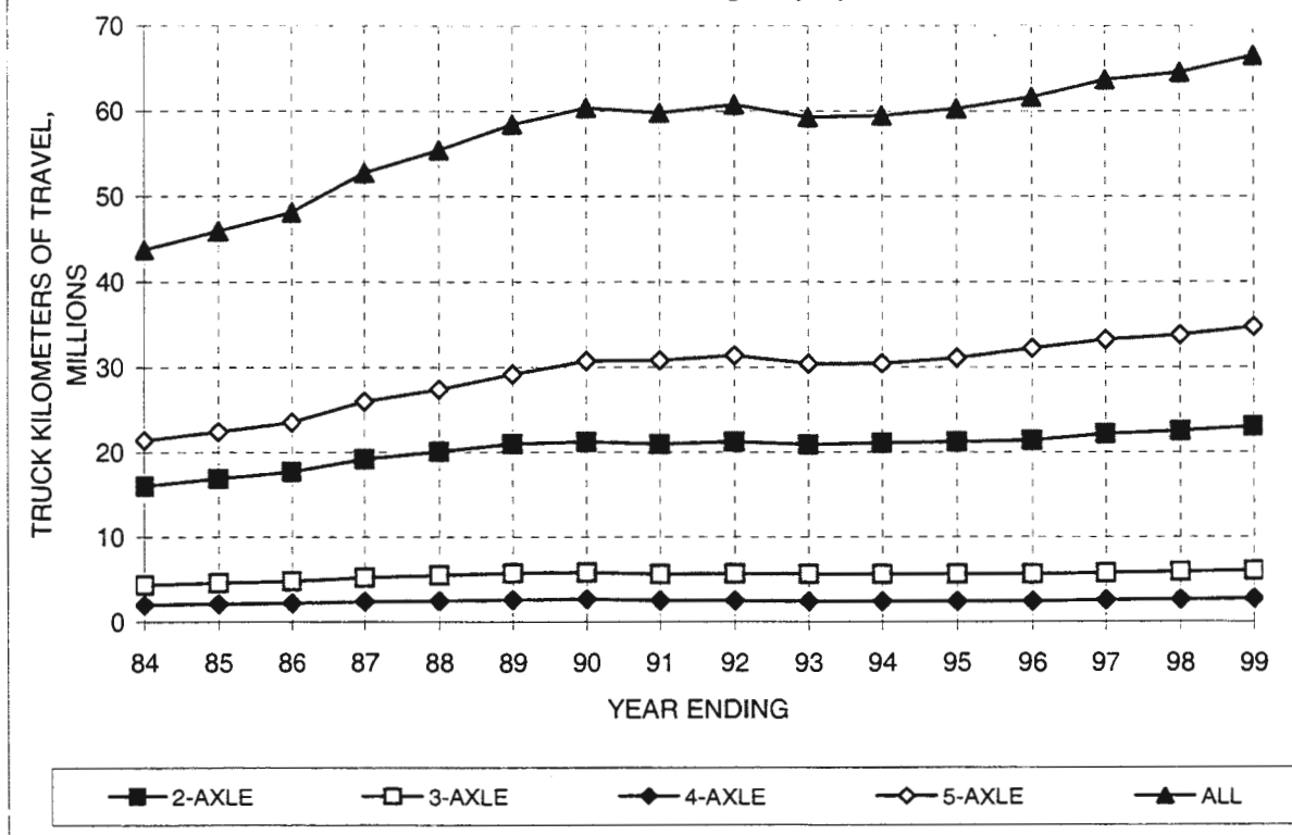
FIGURE A-4 AVERAGE DAILY TRUCK KILOMETERS OF TRAVEL BY AXLE GROUP On the California State Highway System
