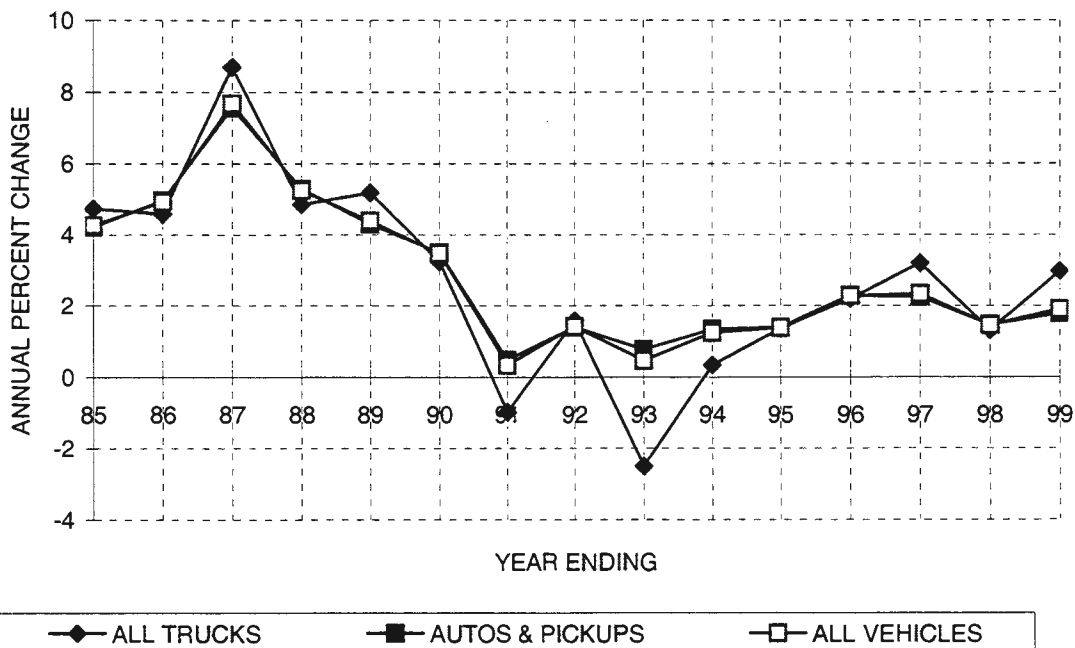
FIGURE A-3 ANNUAL PERCENT CHANGE IN VEHICLE KILOMETERS OF TRAVEL BY VEHICLE TYPE On the California State Highway System
