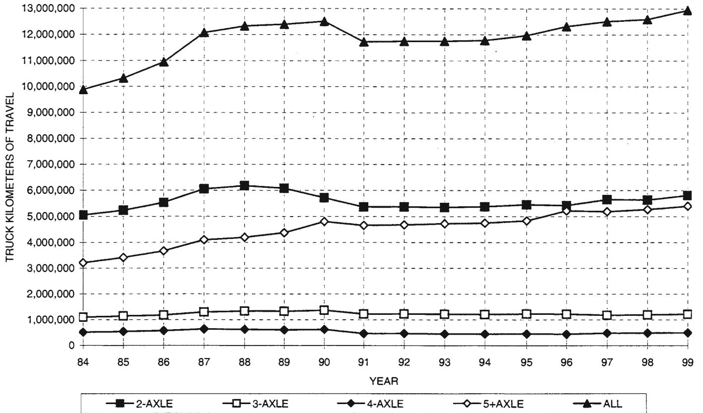
FIGURE B-13 DISTRICT 7-AVERAGE DAILY TRUCK KILOMETERS OF TRAVEL BY AXLE GROUP
