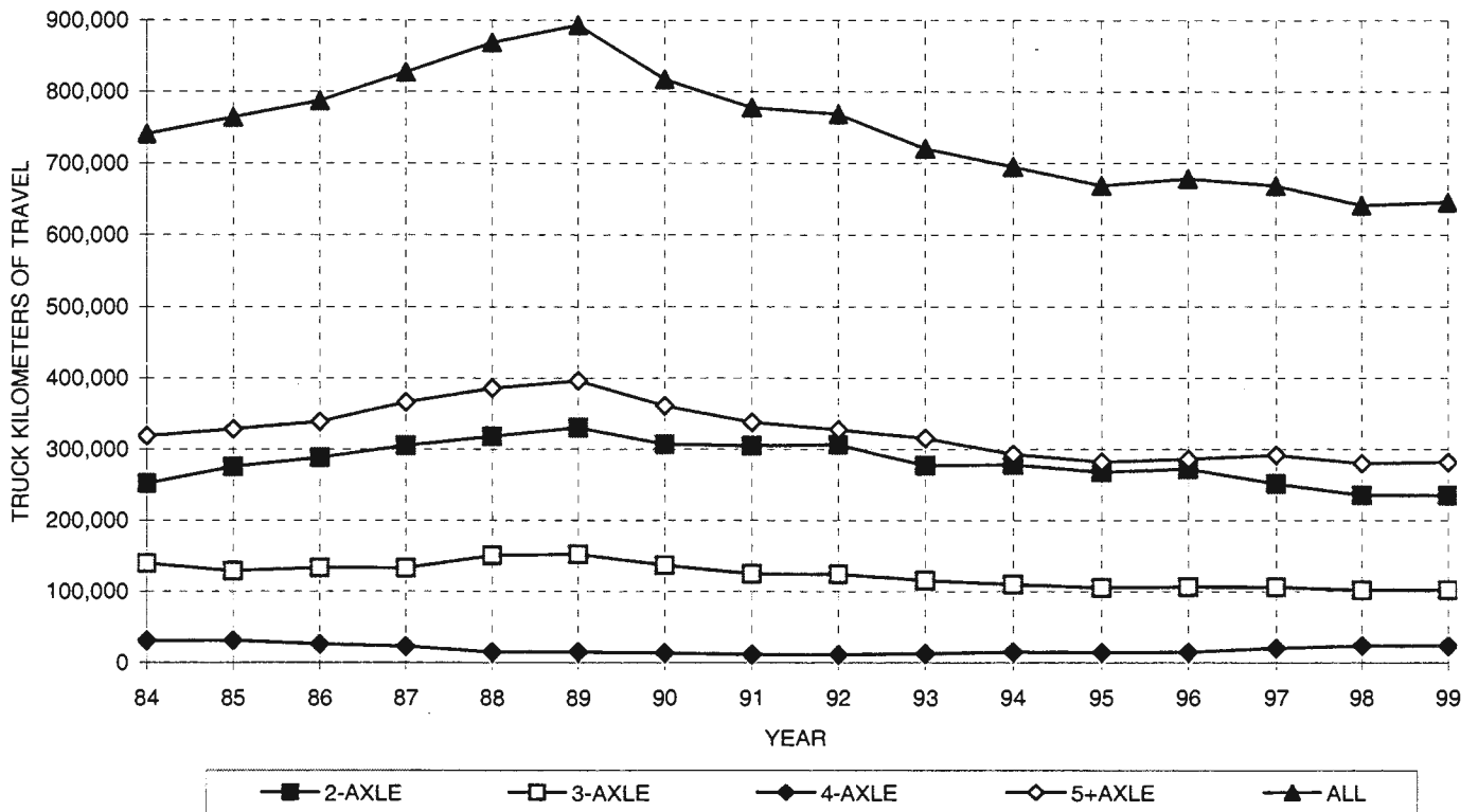
DISTRICT 1 - AVERAGE DAILY TRUCK KILOMETERS OF TRAVEL BY AXLE GROUP
