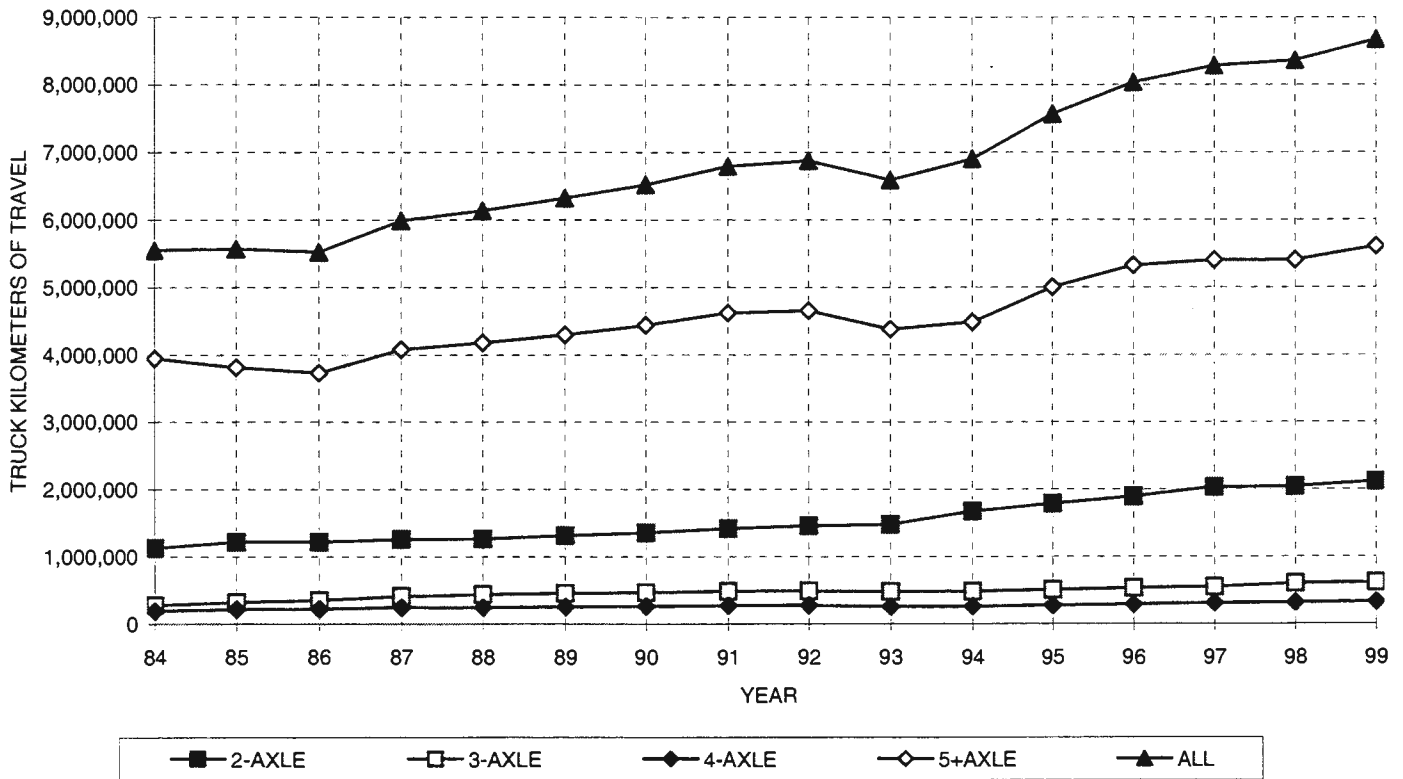
DISTRICT 6 - AVERAGE DAILY TRUCK KILOMETERS OF TRAVEL BY AXLE GROUP
