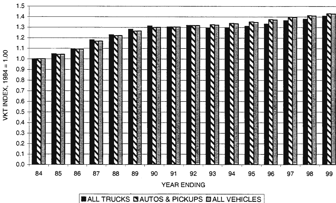
FIGURE A-2 VEHICLE KILOMETERS OF TRAVEL INDEX BY VEHICLE TYPE On the California State Highway System, 1984=1.00
