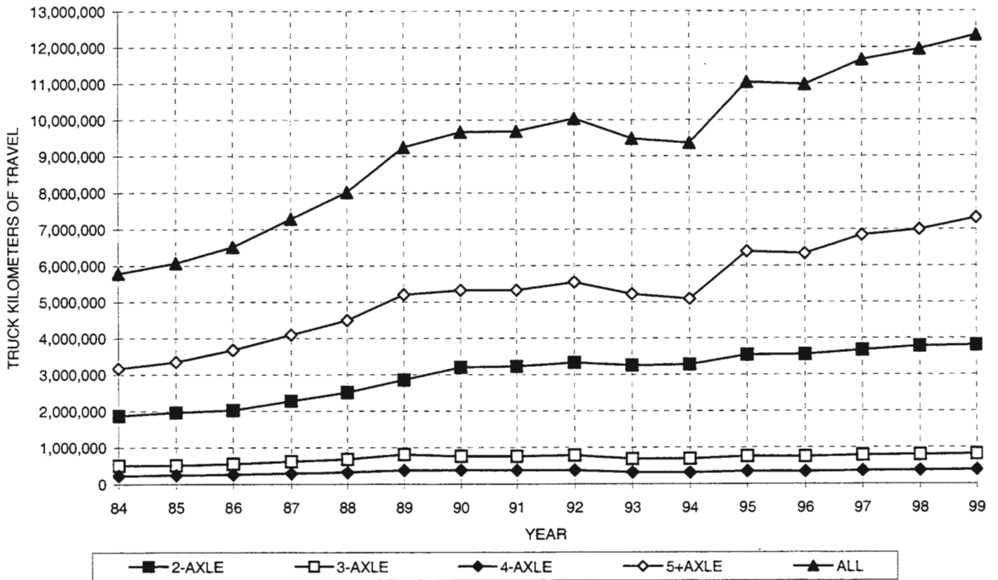
DISTRICT 8 - AVERAGE DAILY TRUCK KILOMETERS OF TRAVEL BY AXLE GROUP
