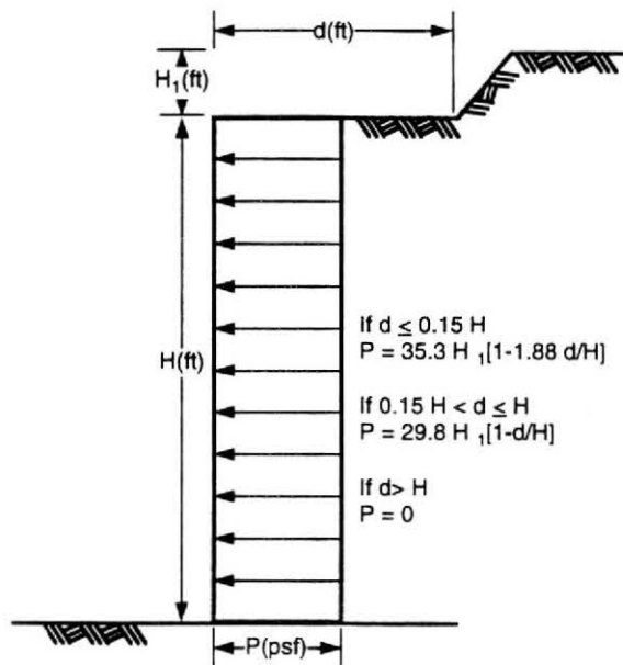
(a) Sloped Excavation Surcharge
