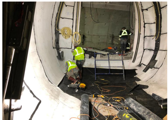
Tunnels: Waterproofing Install at Cross Passage CP-43
