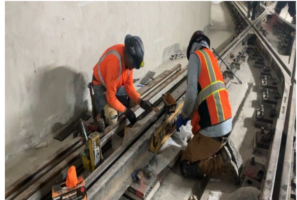
Bonded Joint Installation at DXO
