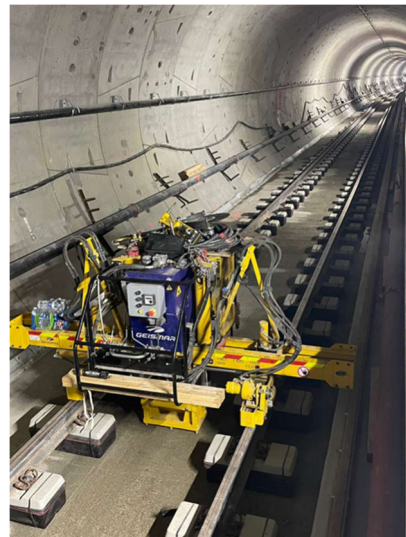
Track/Tunnels: Running Rail Installation in BL Tunnel
