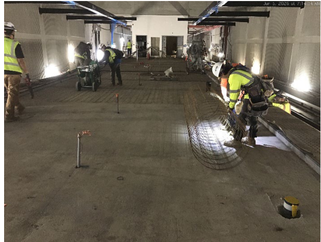
CCS Wire Mesh Installation Platform Level
