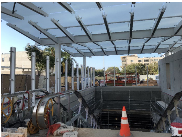
BDS Station Entry Portal
