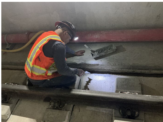
Punchlist - Patching of Track Drain Channel
