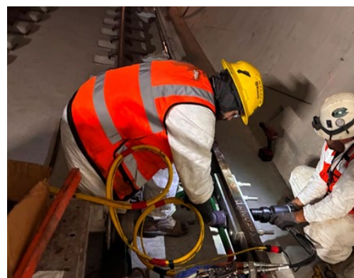
Tunnels/Track: Contact Rail Splice Joint Assemblies Installation
