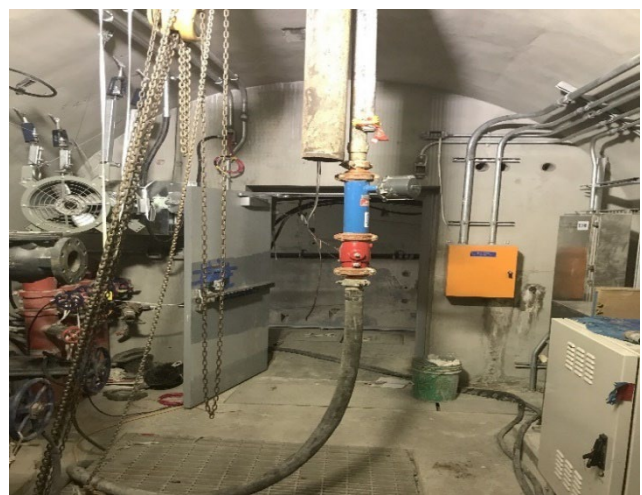
Installation of Discharge Flow Meter at CP27
