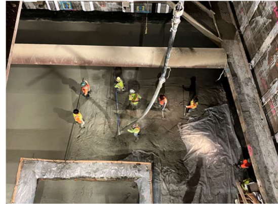
Westwood/UCLA Station: Concrete Placement at Southeast Entrance Invert
