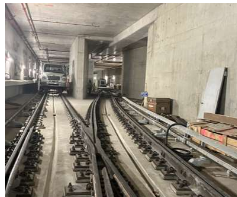
Tunnels/Track: Contact Rail Installation at East Double Crossover
