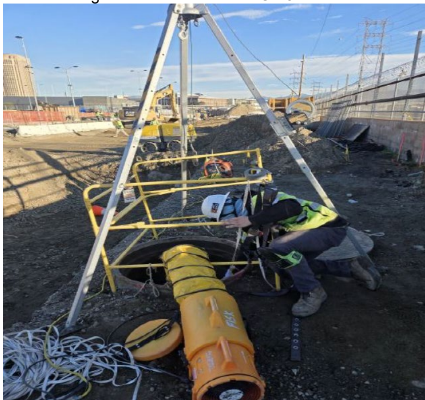
Demoing cable out of manhole C-15 mainline track
