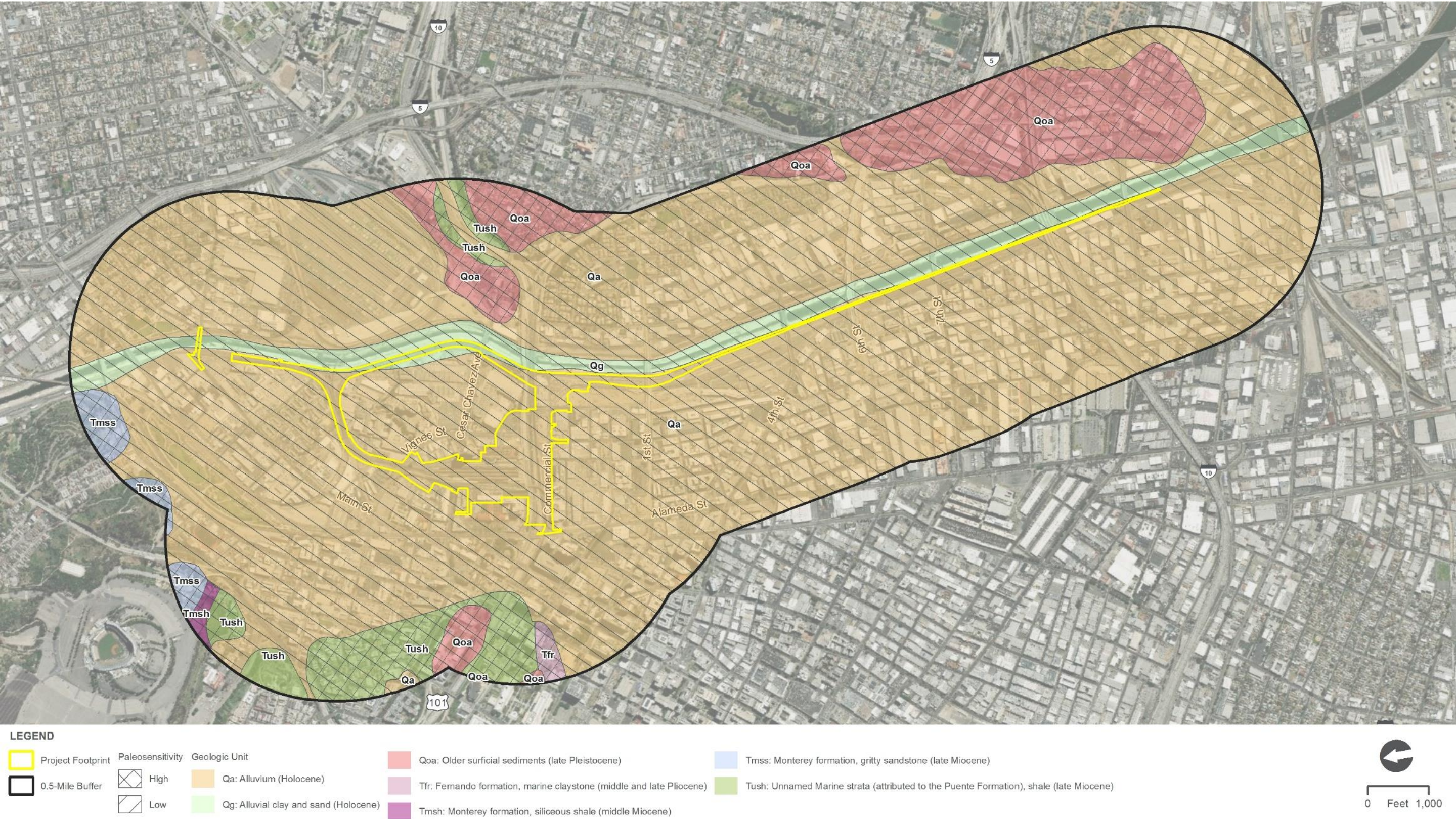
Figure 6-1. Link Union Station Geology
