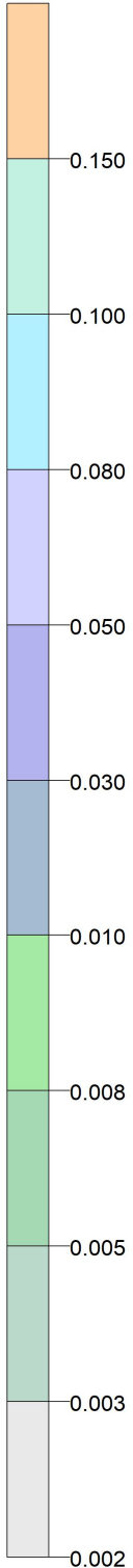
PLOT FILE OF ANNUAL VALUES AVERAGED ACROSS 5 YEARS FOR SOURCE GROUP: ALL Max: 0.150 [ug/m^3] at (386535.34, 3768645.66)
