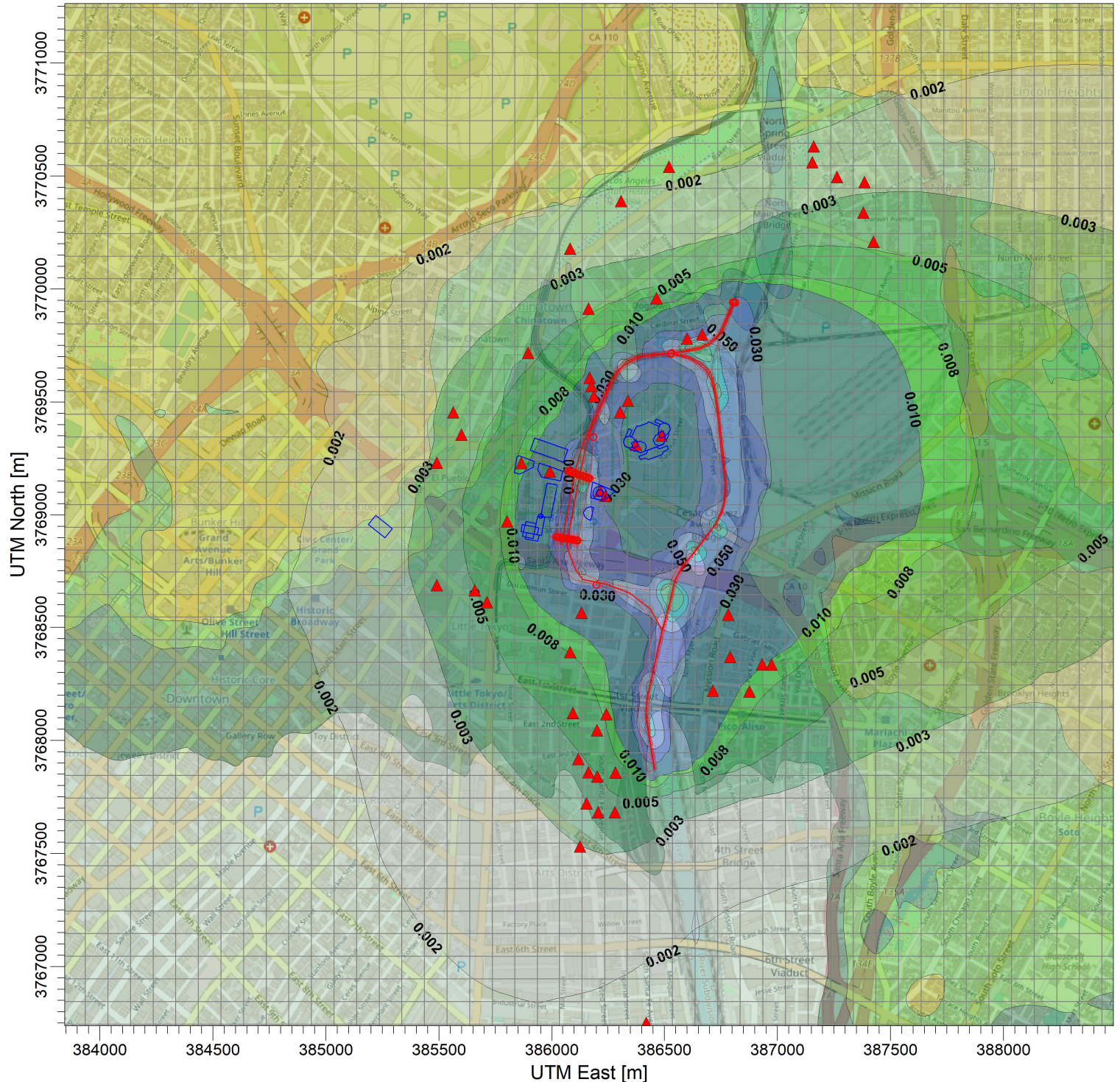
PLOT FILE OF ANNUAL VALUES AVERAGED ACROSS 5 YEARS FOR SOURCE GROUP: ALL Max: 0.150 [ug/m^3] at (386535.34, 3768645.66)
