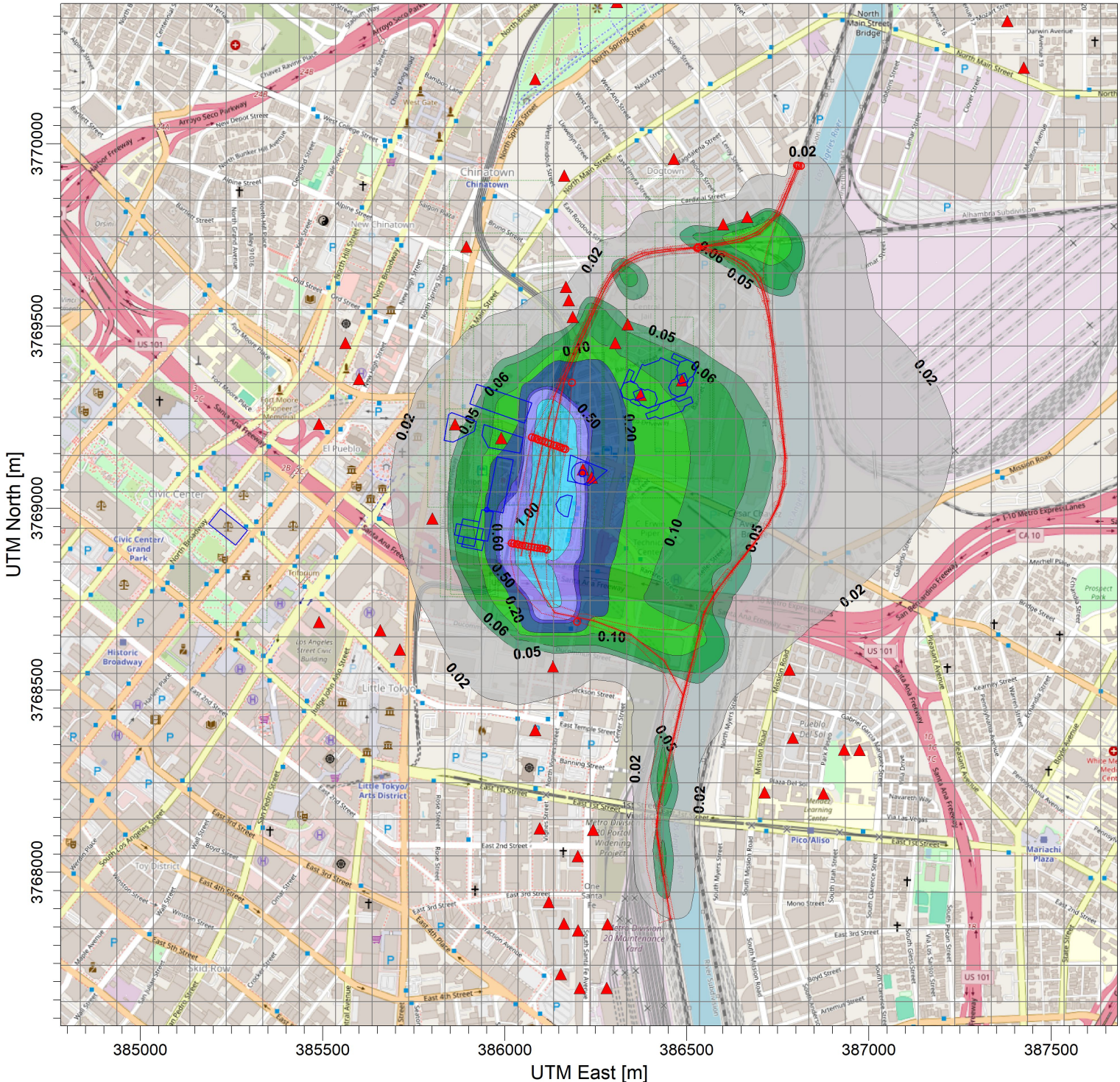
PLOT FILE OF ANNUAL VALUES AVERAGED ACROSS 5 YEARS FOR SOURCE GROUP: ALL Max: 2.08 [ug/m³] at (386135.34, 3769145.66)
