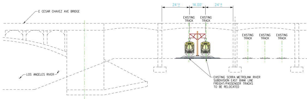
Figure 2.12 – Typical LRT Operational Cross-Sections Cesar Chavez Avenue Bridge
