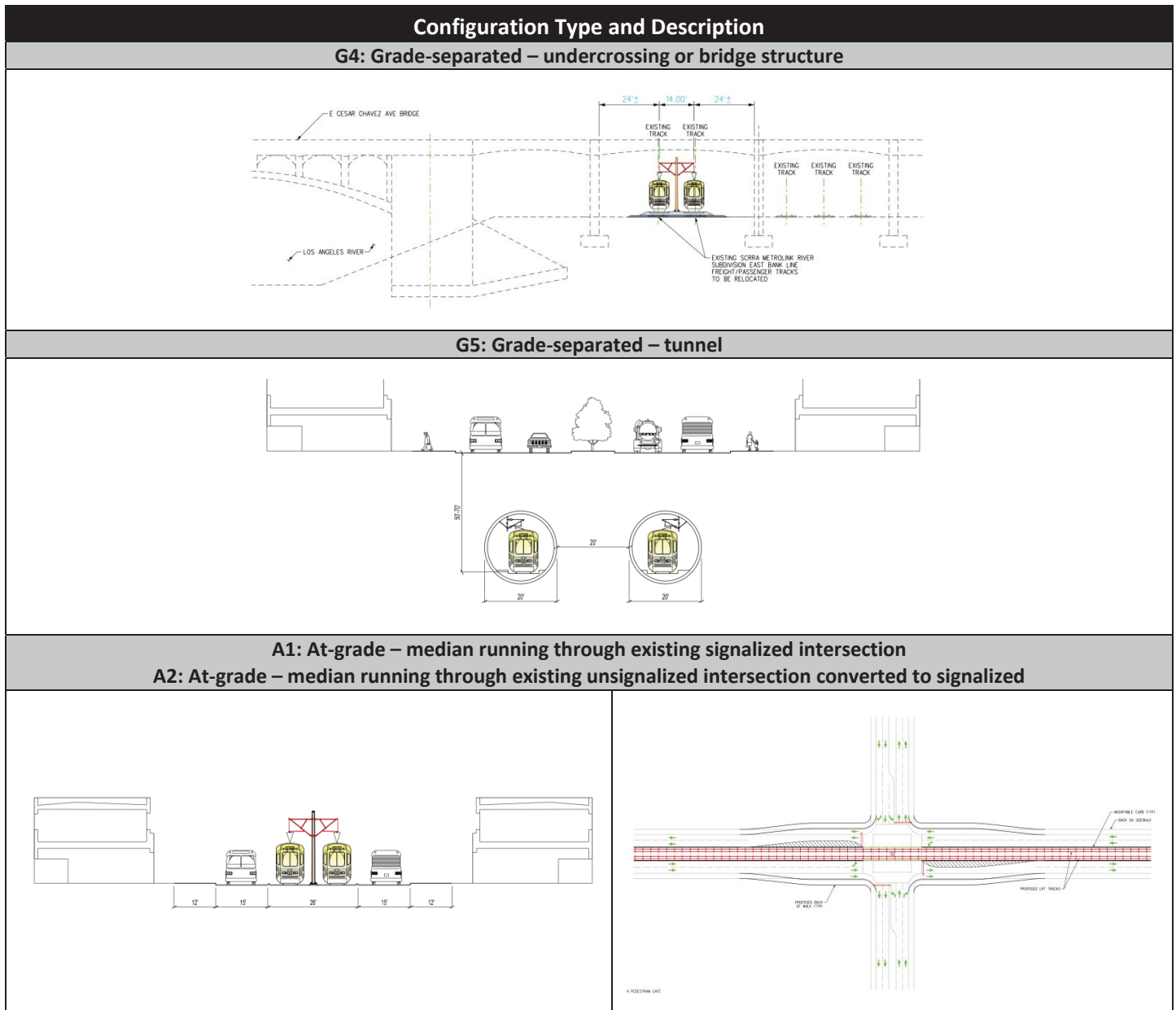
Figure 3.5 – Intersection Types
