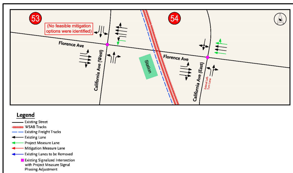
Figure 3-15. Intersection Nos. 53 and 54 Lane Configurations with Mitigation Measures
