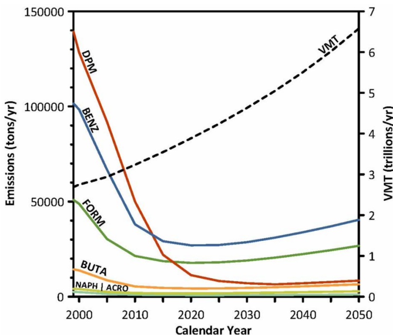
Figure 3.1-1. National MSAT Emission Trends 1999–2050 for Vehicles Operating on Roadways Using USEPA’s MOBILE6.2 Model
