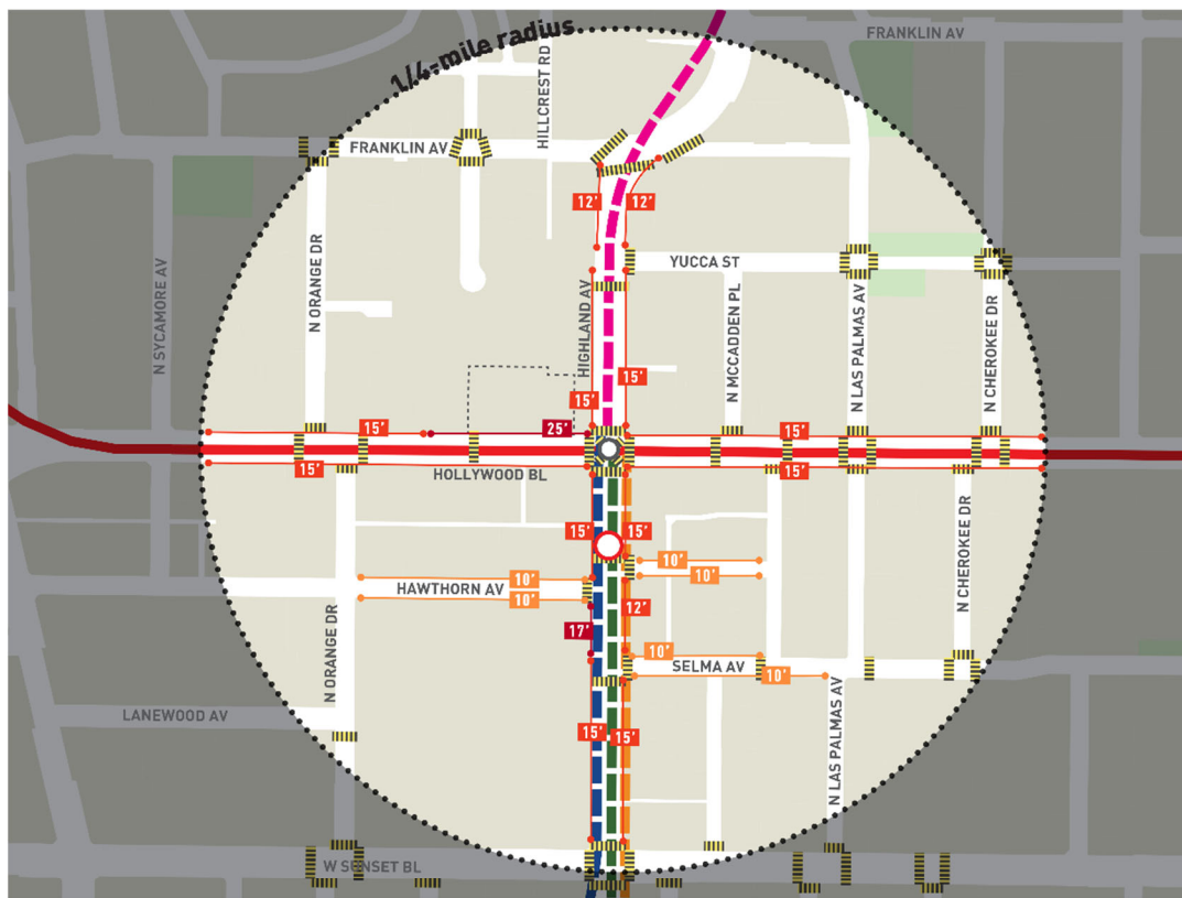
FIGURE 5-40. PEDESTRIAN SIDEWALK WIDTH AT HOLLYWOOD/HIGHLAND STATION
