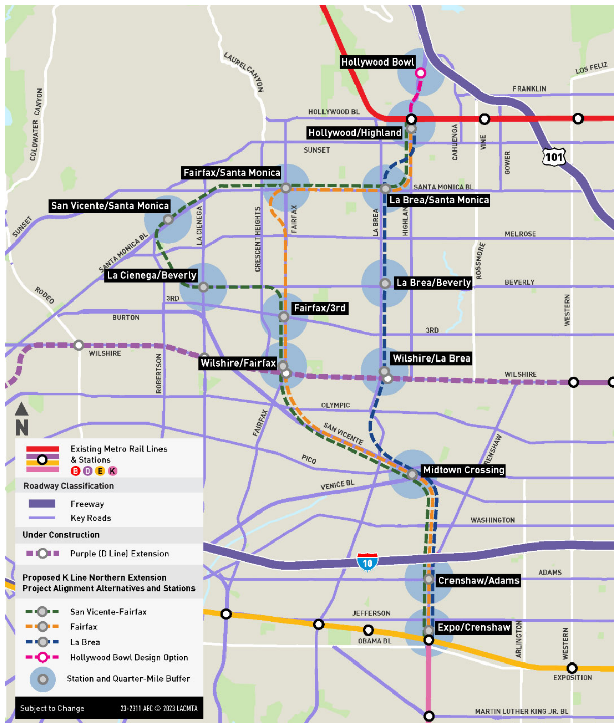
FIGURE 5-17. FREEWAY AND ARTERIAL NETWORKS IN THE STATION RESOURCE STUDY AREAS
