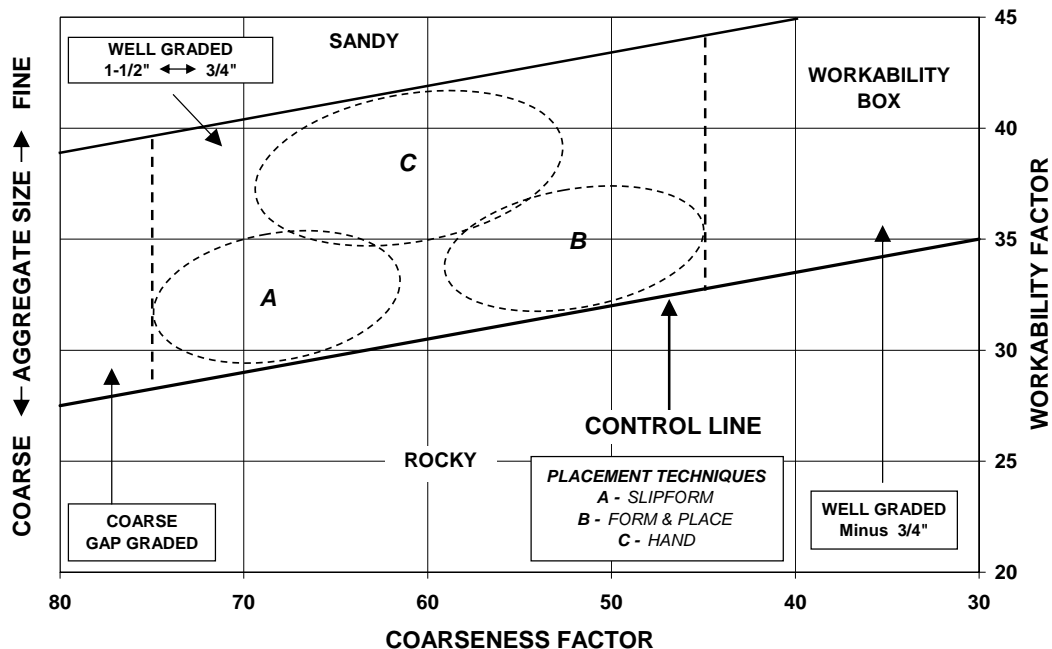
Fig. 16- Air Force Aggregate Proportioning Guide with construction-related areas.
