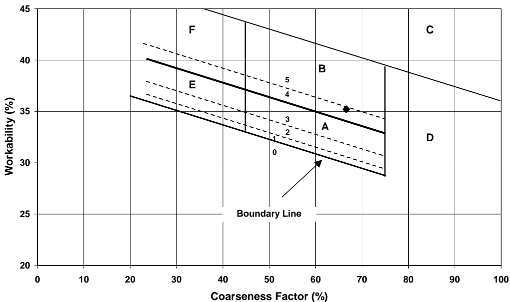
Fig. 51-Iowa DOT CF chart- better mixture.
