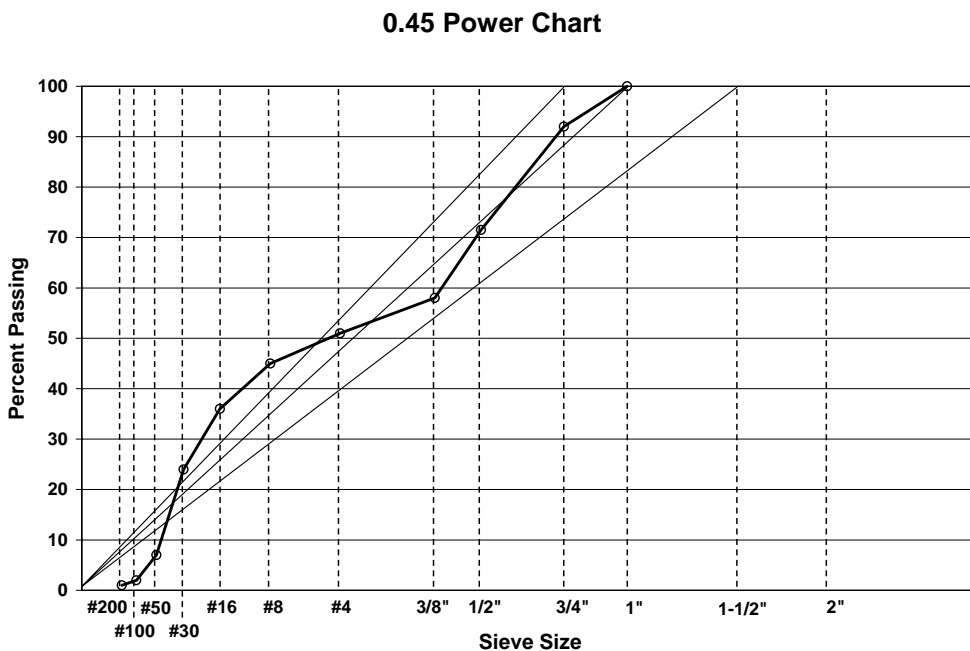
Fig. 21- Example of a gap graded mixture, Iowa DOT specifications, 0.45 power chart.
