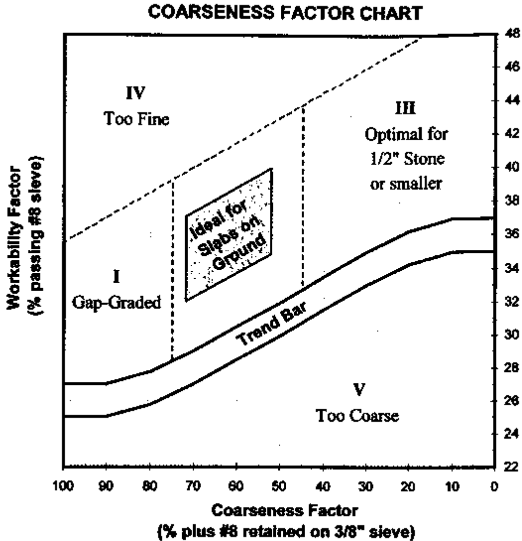
Fig. 11-Optimum location on CF chart for slabs-on-ground.
