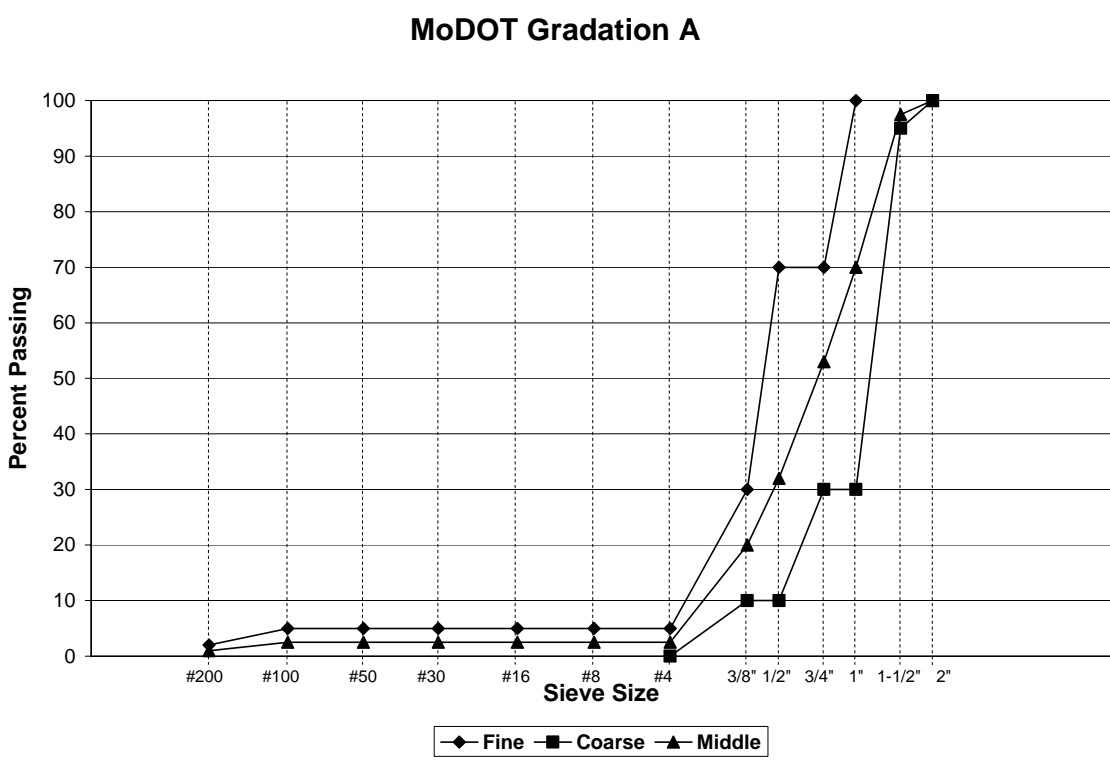
Fig. 42-Gradation A limits.
