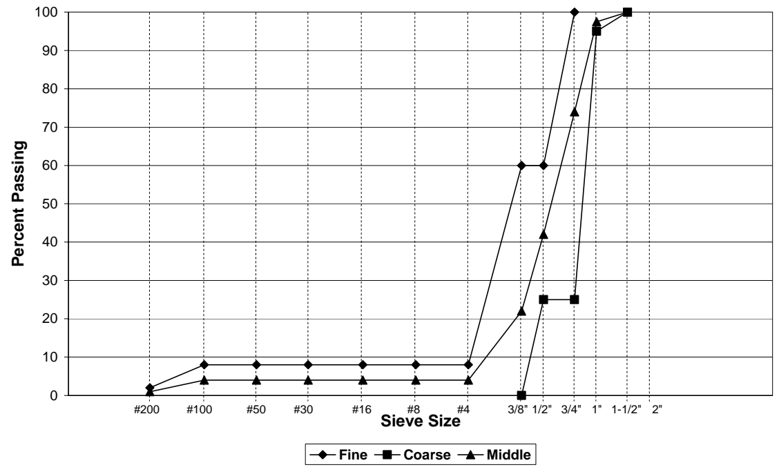
Fig. 43-Gradation B limits.
