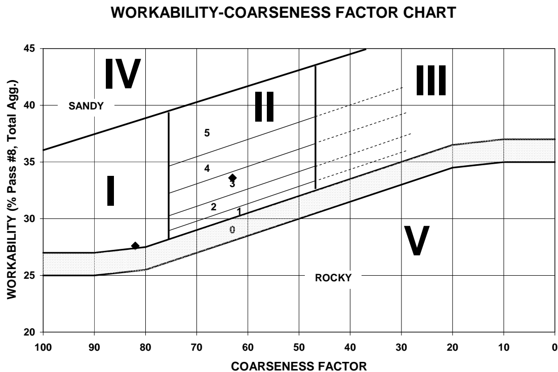
Fig. 10- Wilson and Richardson's 's traditional and optimized mixes.
