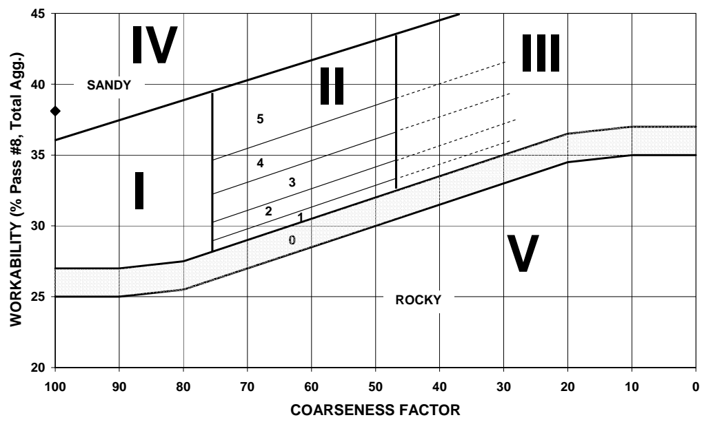
Fig. 46-Shilstone CF chart--problem mixture, B_{cf} .
