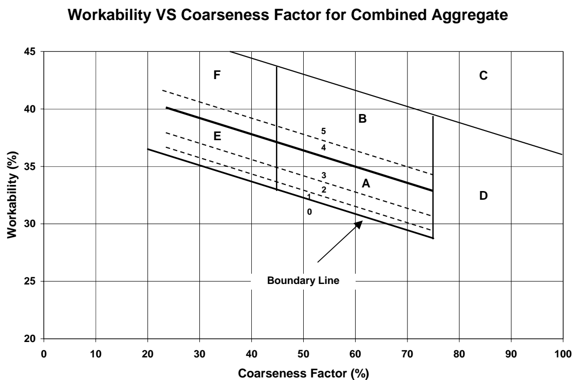
Fig. 19- Iowa DOT Coarseness Factor Chart.
