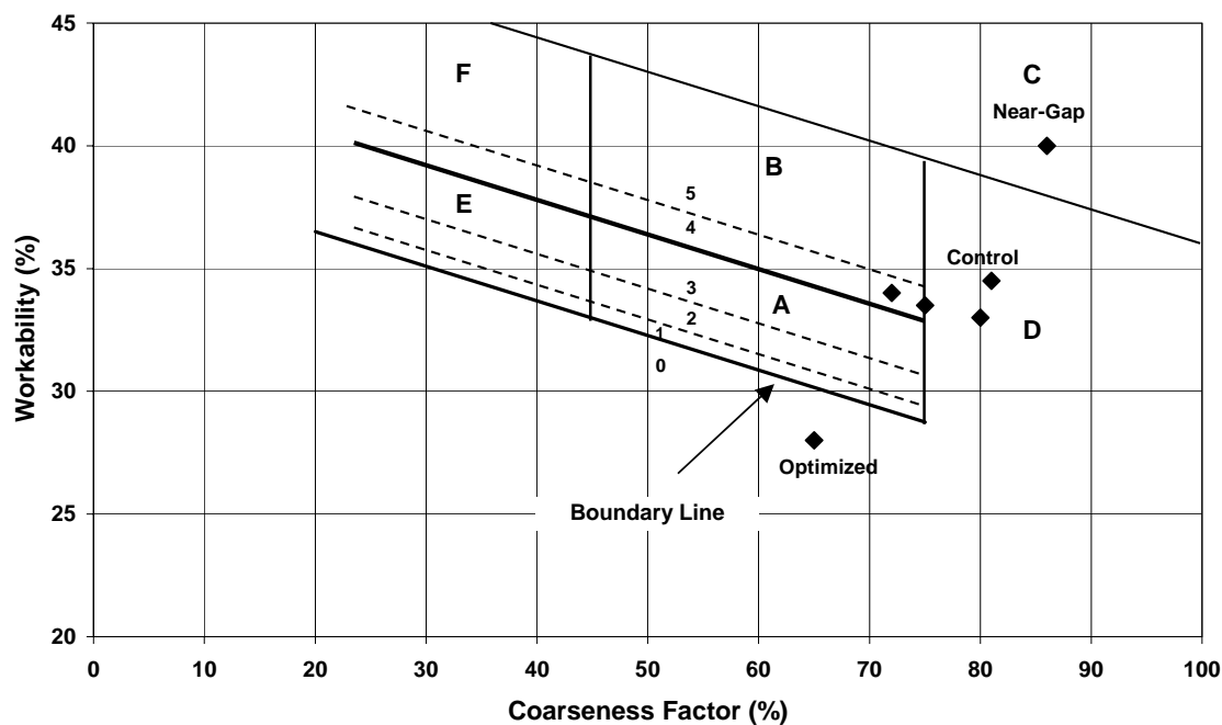
Fig. 33- Wisconsin DOT durability study-Iowa DOT Coarseness Factor chart.
