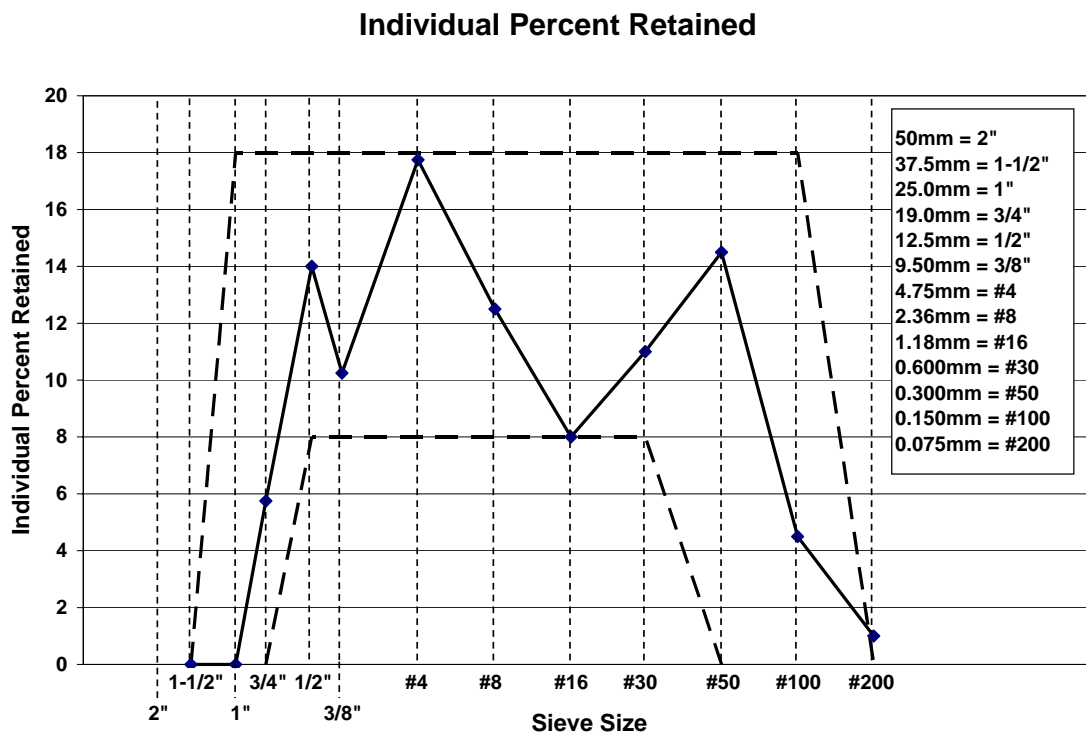
Fig. 22-Example of a well graded mixture, Iowa DOT specifications, Individual Percent Retained.
