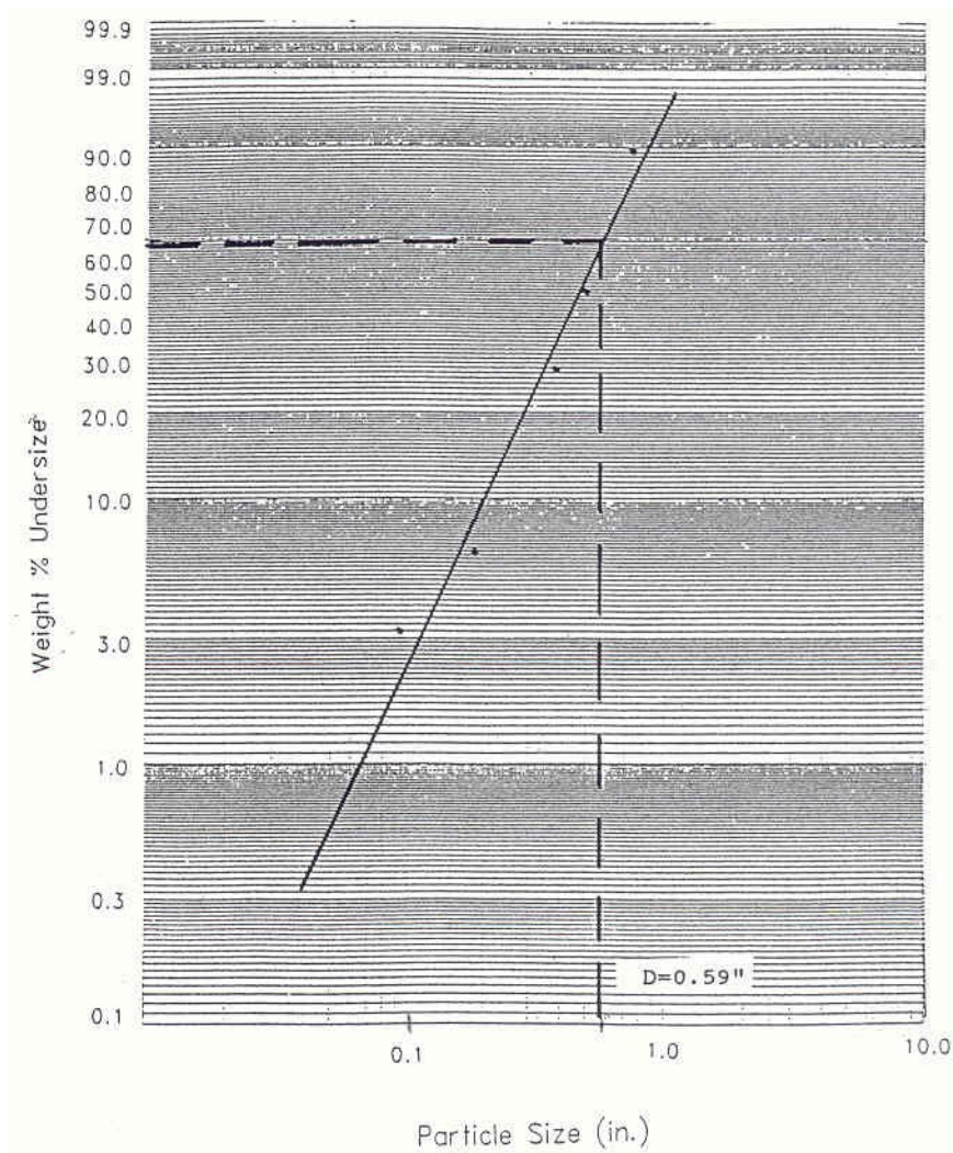
Fig. 39- Rosin-Rammler Plot for coarse aggregate.
