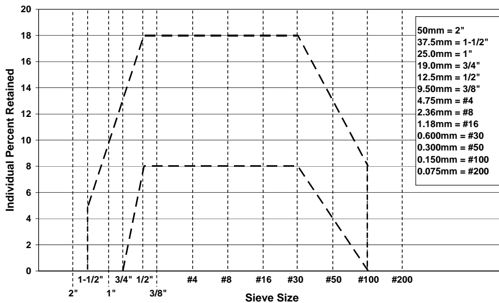
Fig. 37- Shilstone 8-18 band.
