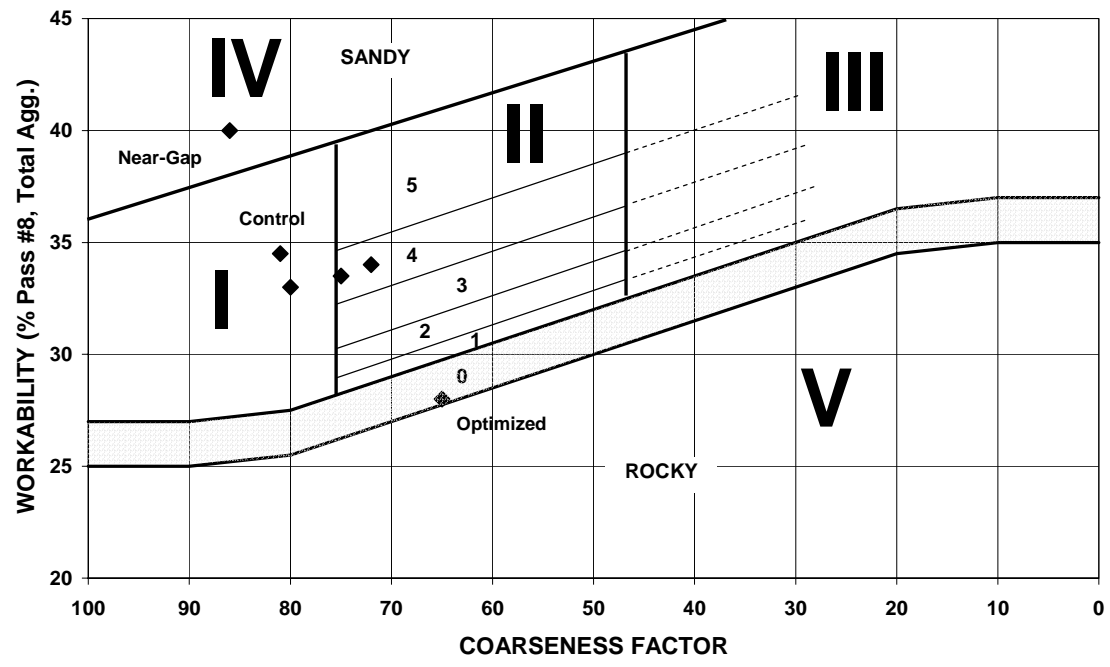
Fig. 31- Wisconsin DOT durability study-Shilstone Coarseness Factor chart.
