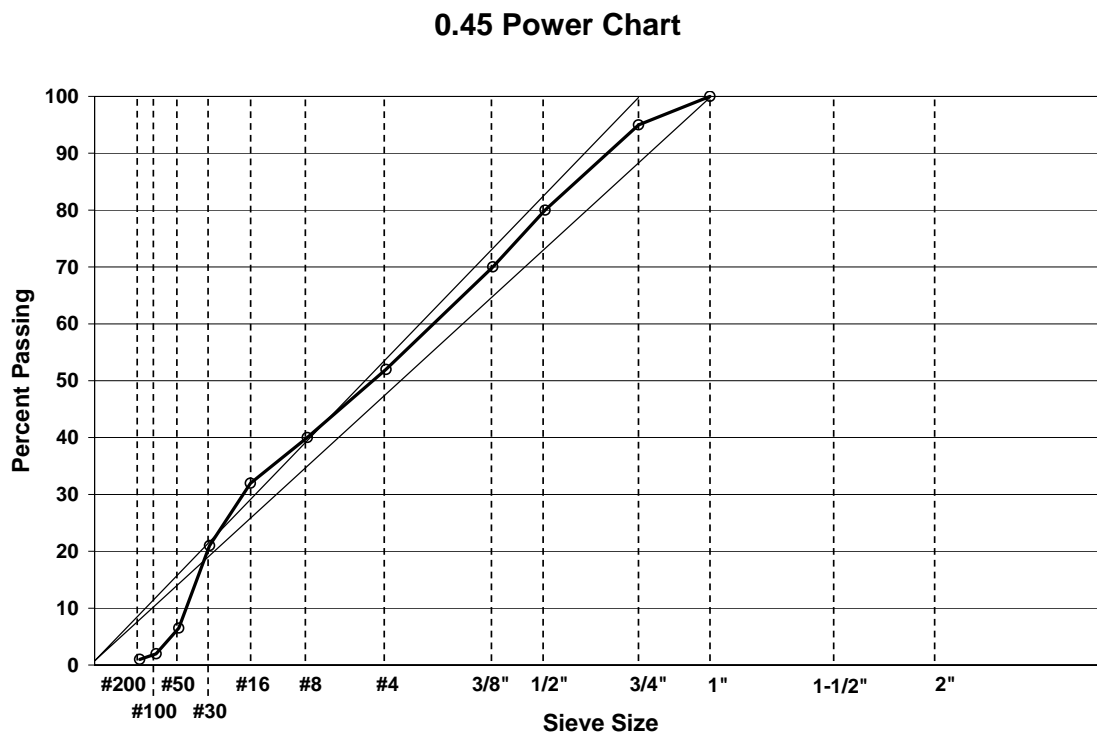
Fig. 8- Shilstone's 0.45 power chart.
