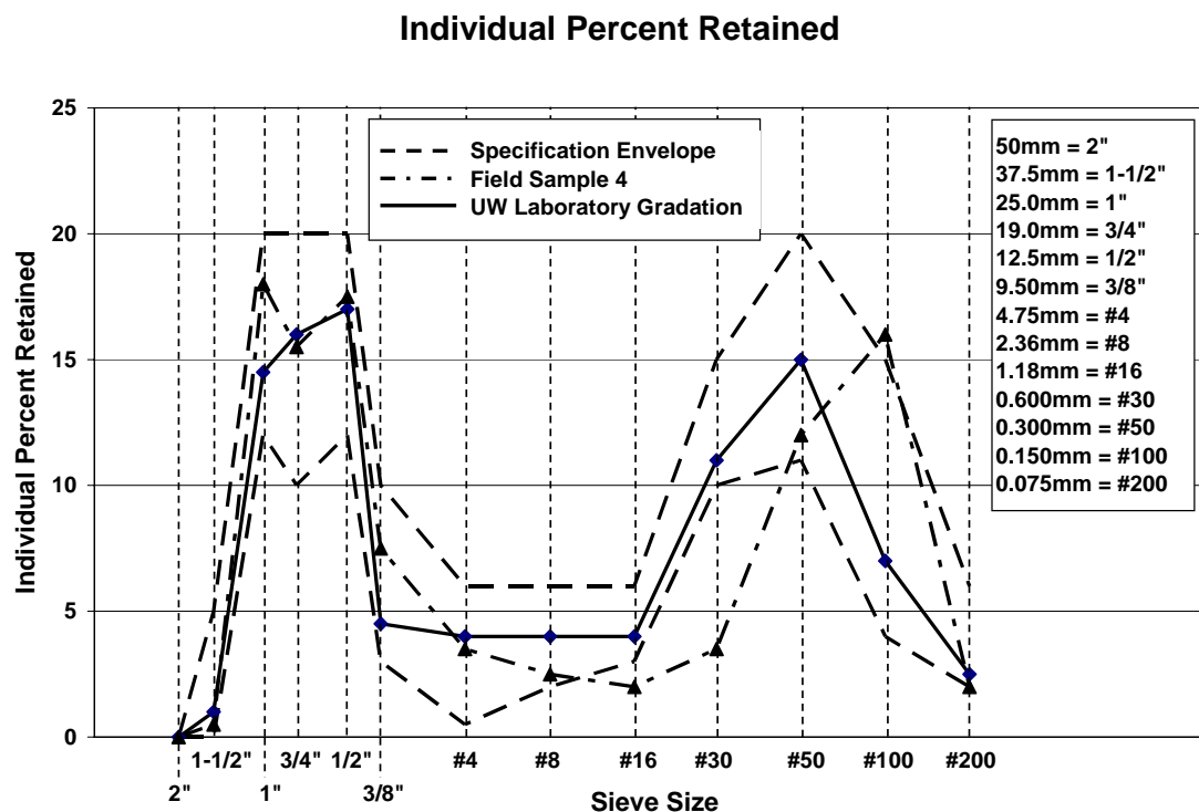
Fig. 27- Wisconsin DOT gap graded pavement mixtures.
