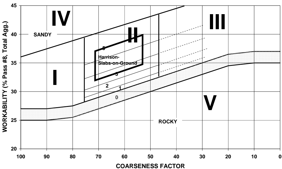
Fig. 35-Harrison vs. Shilstone recommendations.
