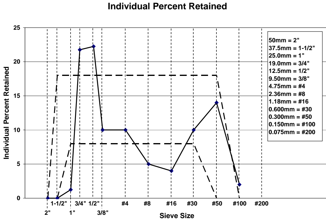
Fig. 14- Example of a problem mix-large percentage of large stone.
