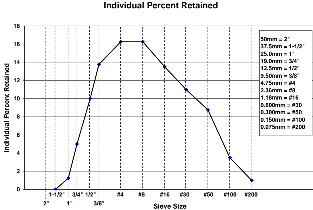
Fig. 2- Ideal "haystack" gradation, Individual Percent Retained.
