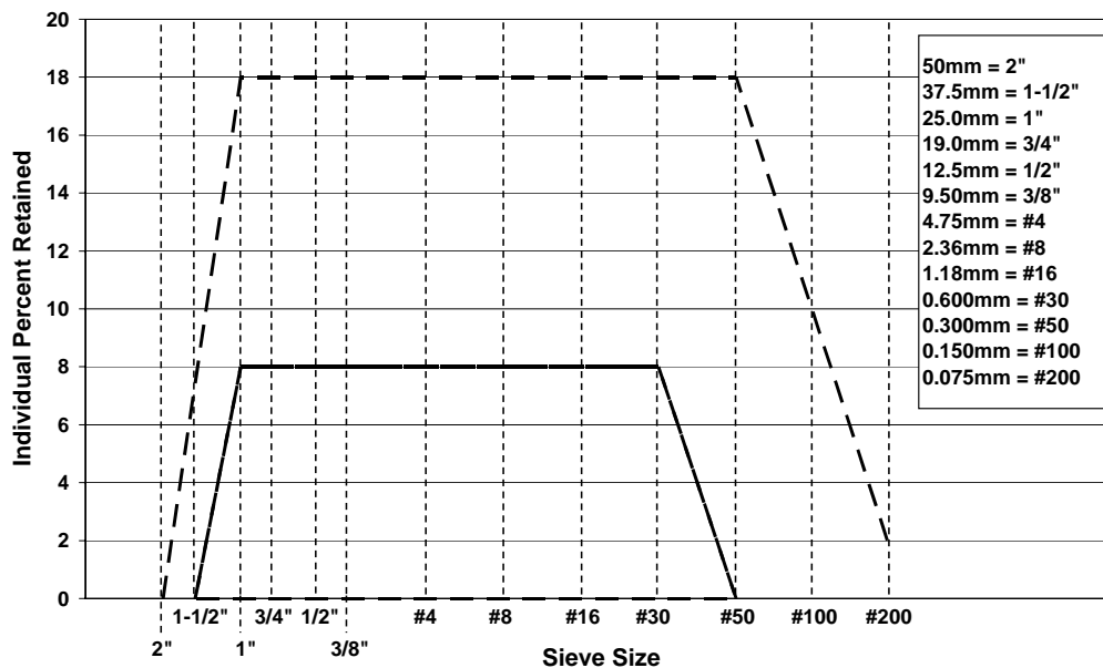
Fig. 36-MnDOT 8-18 band.
