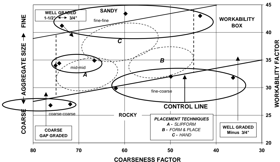
Fig. 55- Summary of MoDOT gradations on USAF Guide.
