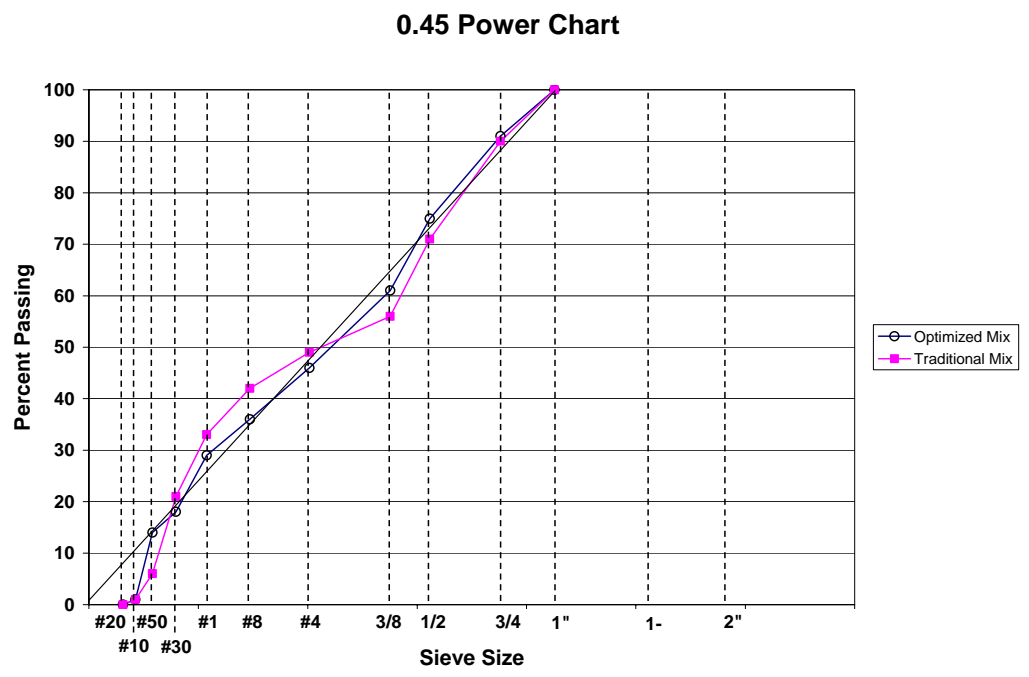
Fig. 25- Iowa DOT barrier wall mixtures-0.45 power chart.
