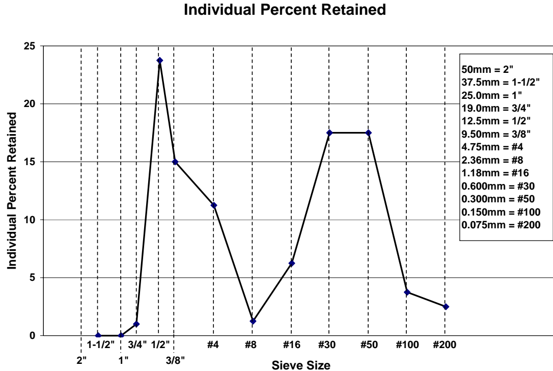
Fig. 3- Double hump, Individual Percent Retained.
