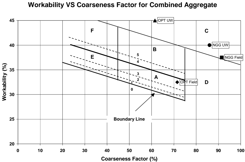
Fig. 29- Wisconsin DOT gap graded and optimized mixtures on Coarseness Factor Chart.
