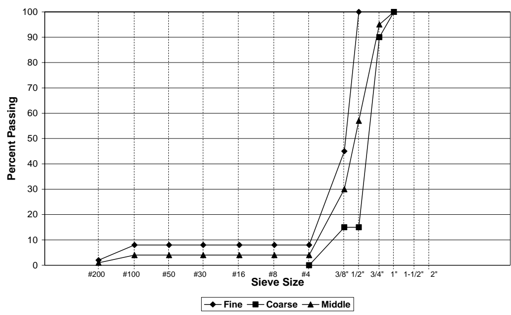
Fig. 44-Gradation D limits.
