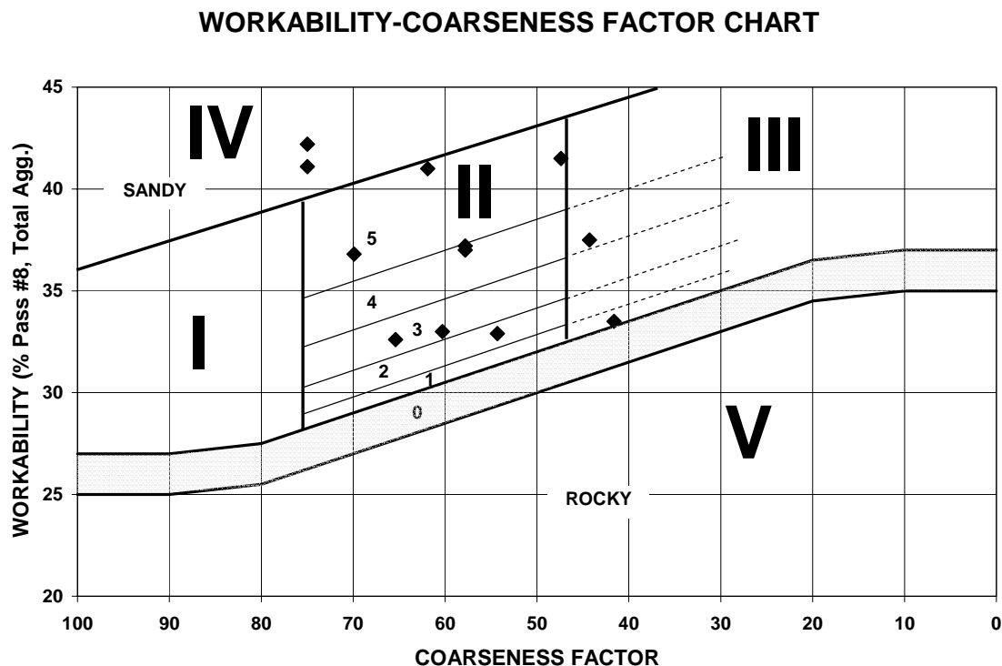
Fig. 9- Effect of varying gradation within ASTM C-33 limits.
