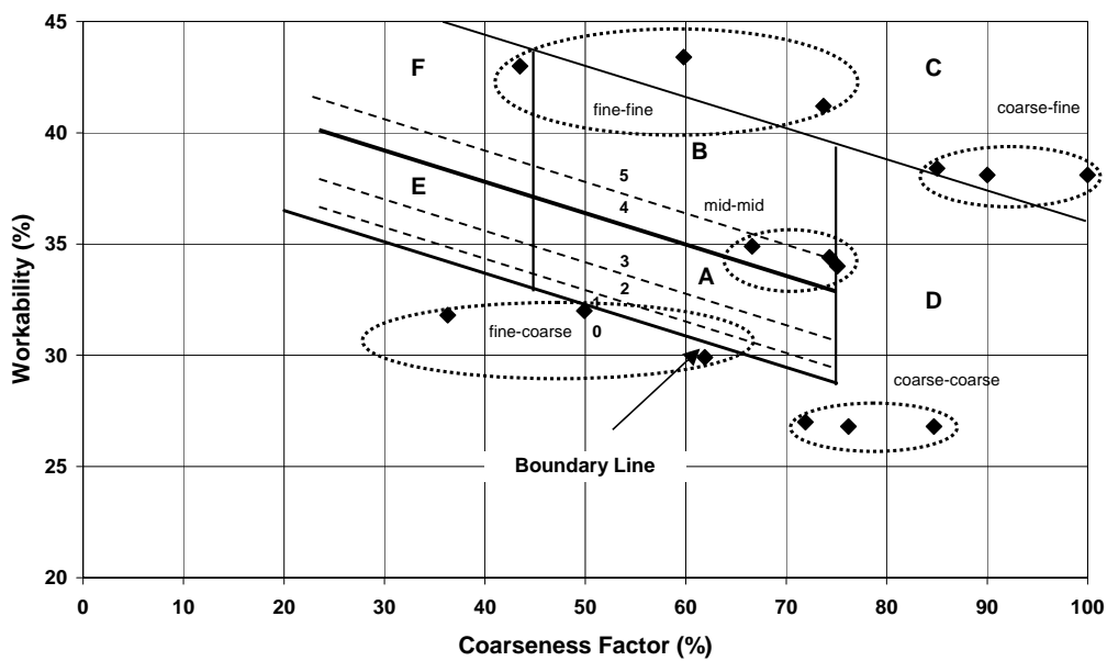
Fig. 54- Summary of MoDOT gradations on Iowa DOT CF chart.
