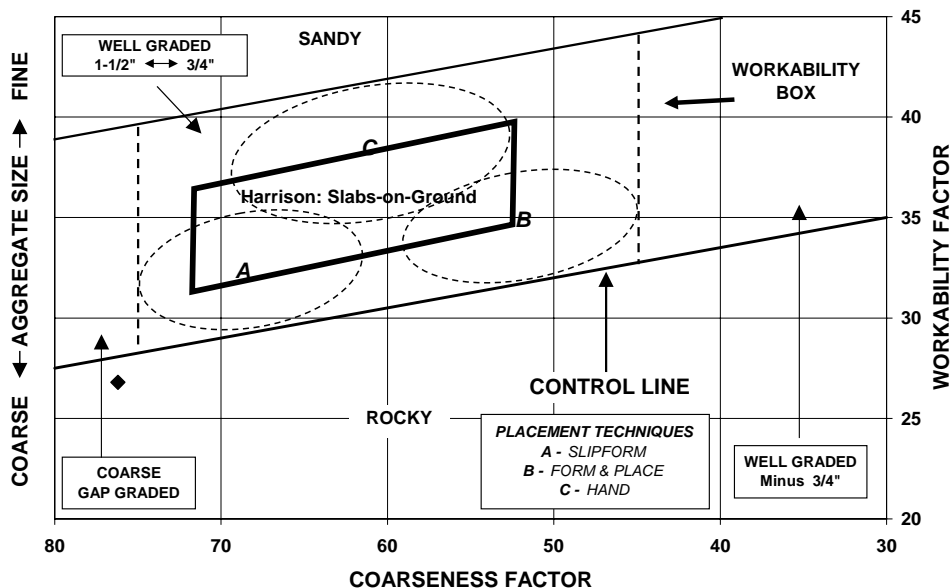
Fig. 34-Harrison vs. USAF recommendation.
