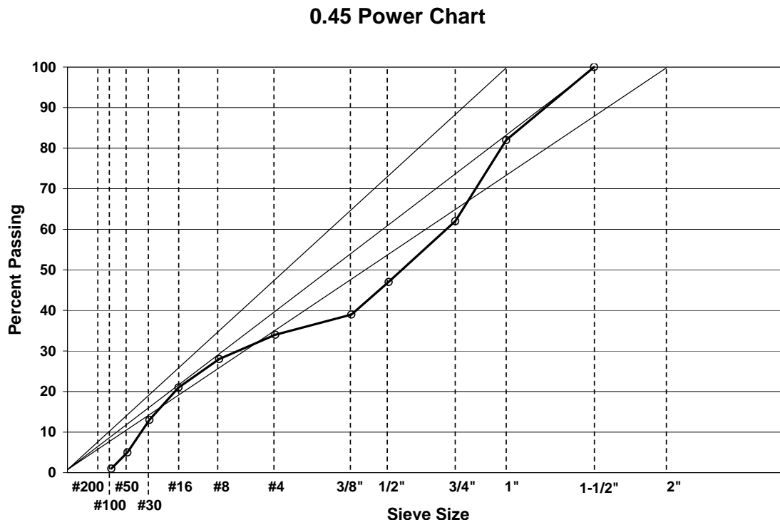
Fig. 18- Air Force 0.45 power chart.
