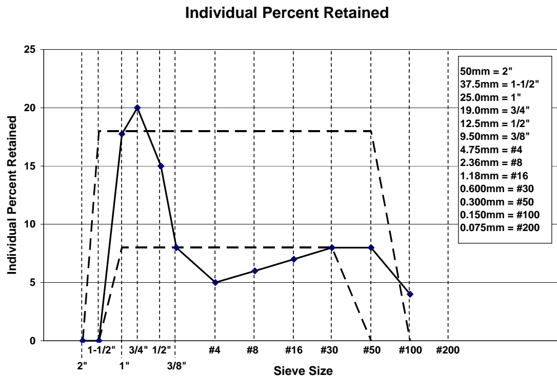
Fig. 13- Example of a problem mix-more than two adjacent sieves between two peaks.
