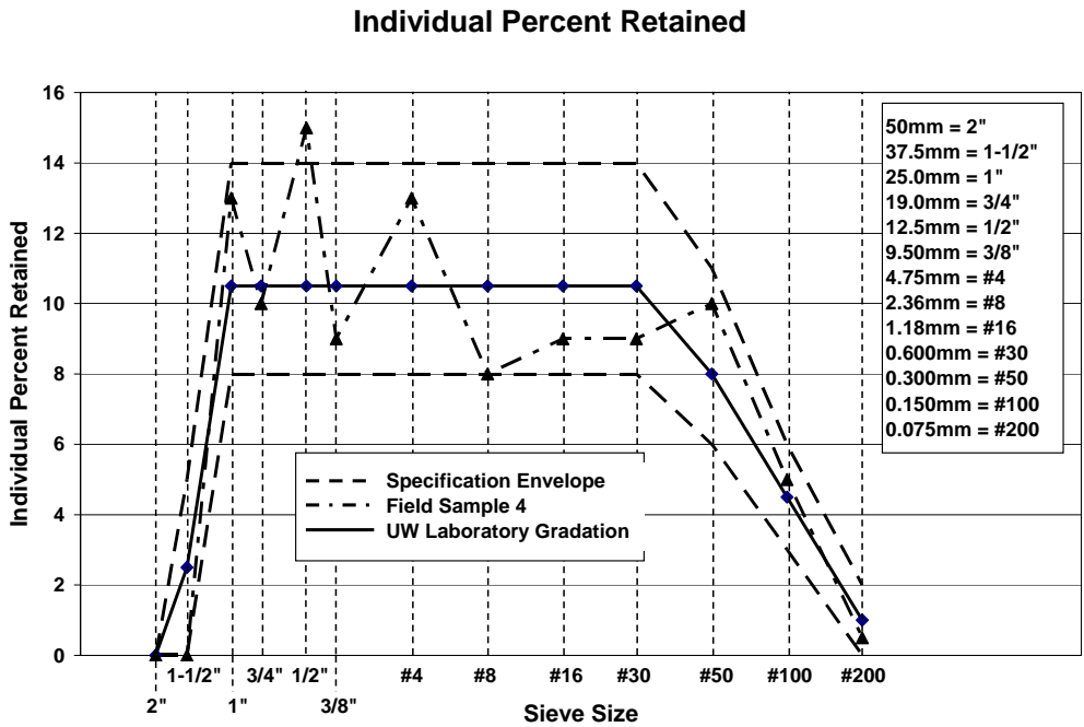
Fig. 28- Wisconsin DOT optimized pavement mixtures.
