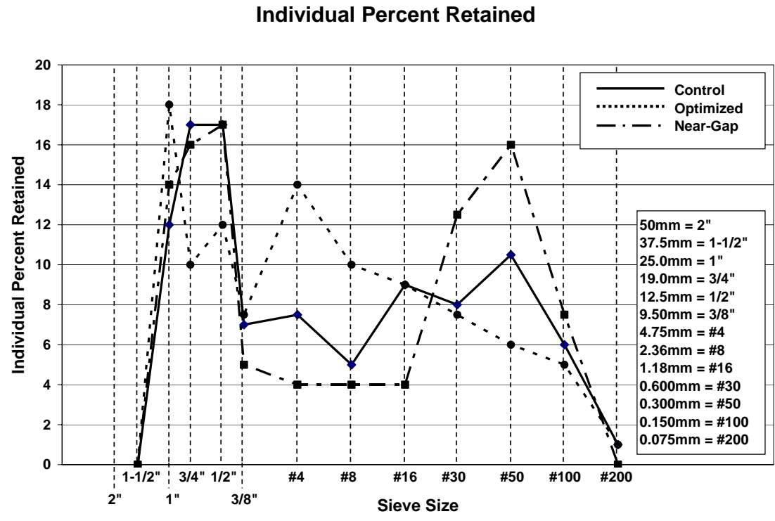
Fig. 30- Wisconsin DOT durability study-optimized and gap graded mixtures.
