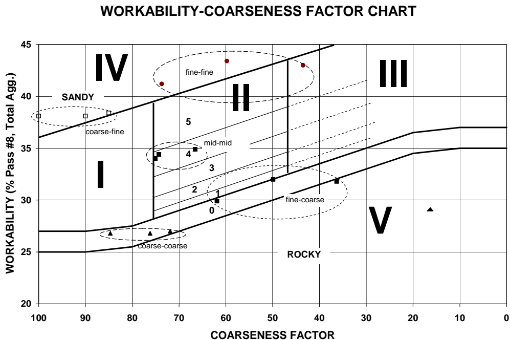
Fig. 53- Summary of MoDOT gradations on Shilstone CF chart.
