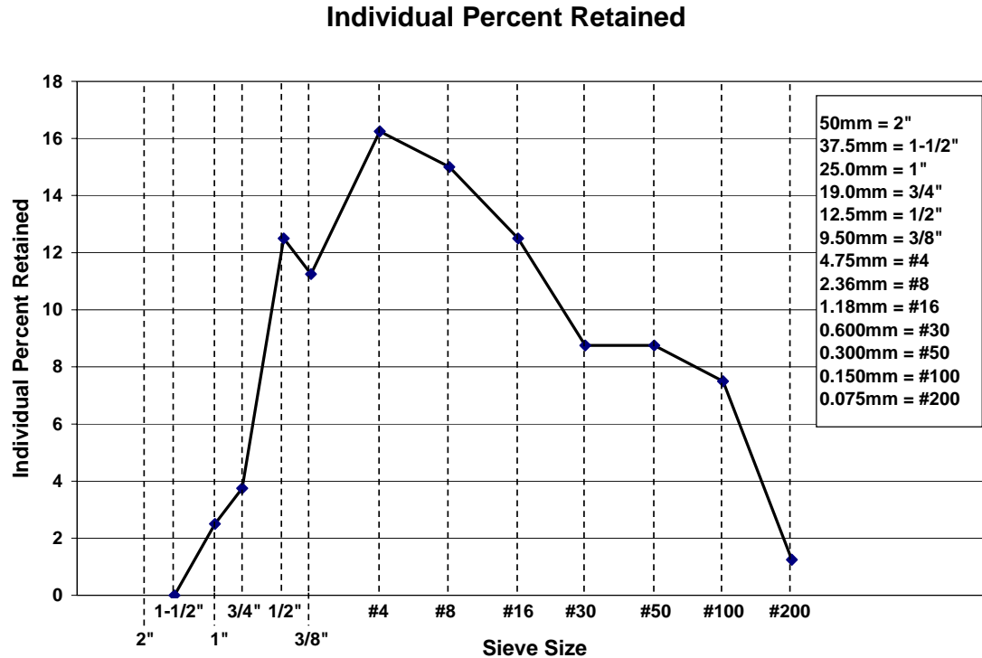
Fig. 5- ASTM C 33 and 1923 sand combined gradation.
