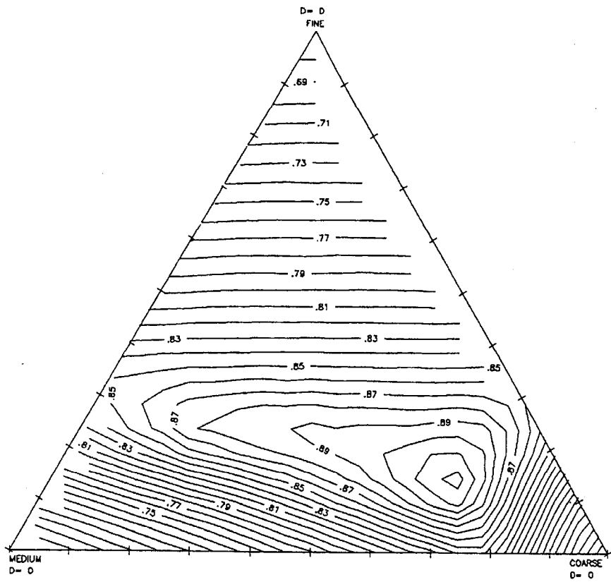
Fig. 41- Packing Handbook example ternary chart.
