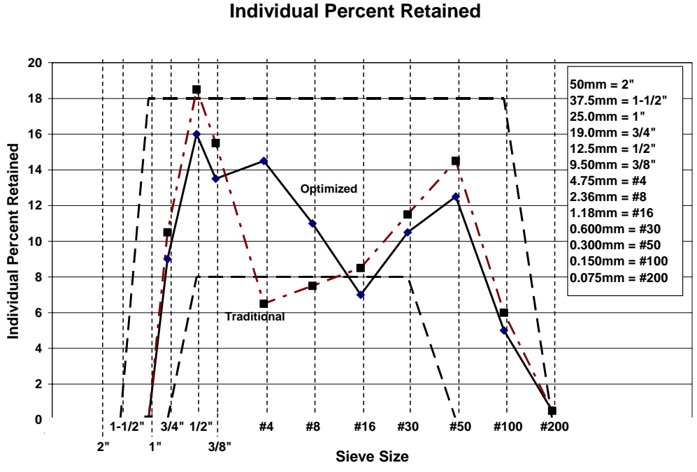
Fig. 24- Iowa DOT barrier wall mixtures-Individual Retained chart.
