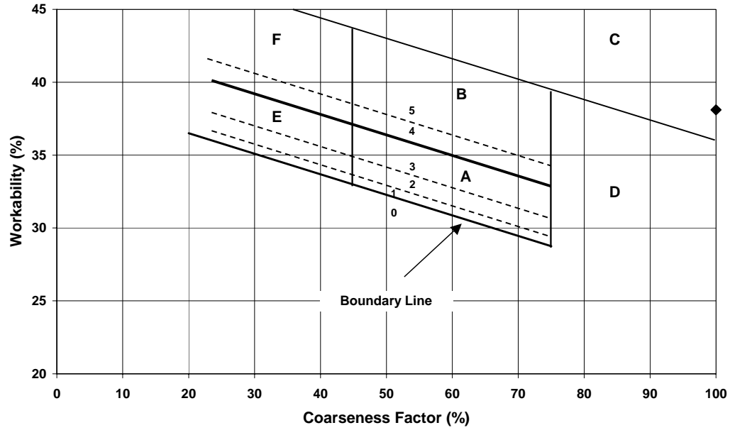
Fig. 47-Iowa DOT CF plot--problem mixture, B_{cf} .
