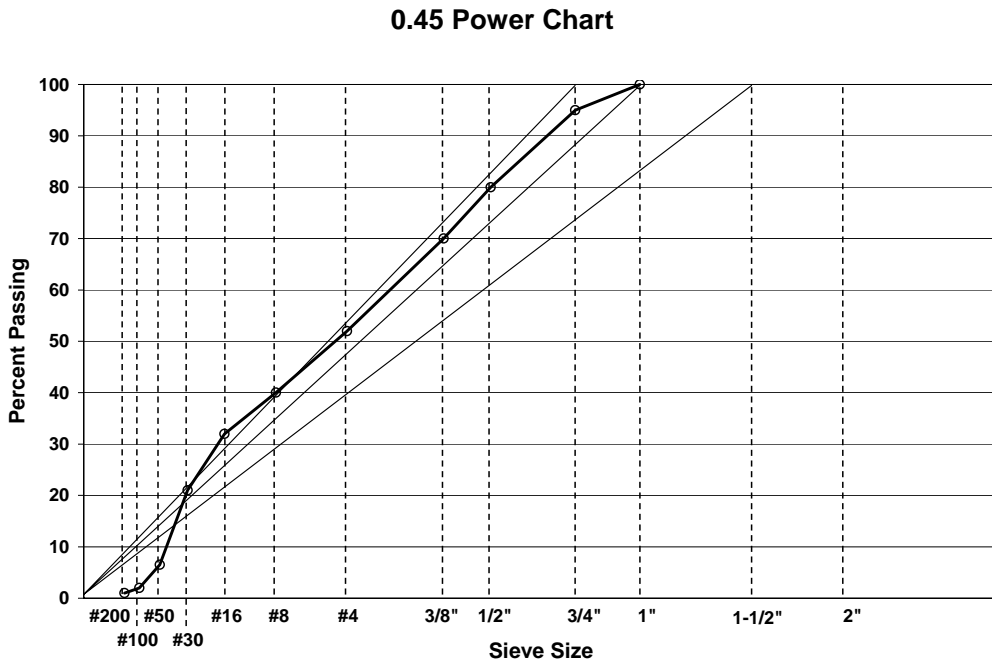
Fig. 20- Example of a well graded mixture, Iowa DOT specifications 0.45 power chart.
