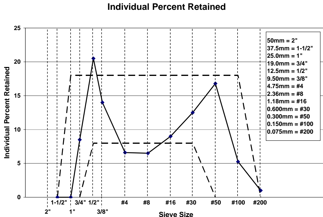
Fig. 23-Example of a gap graded mixture, Iowa DOT specifications, Individual Percent Retained.
