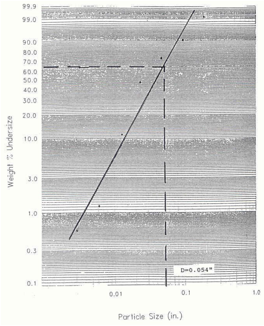
Fig. 38- Rosin-Rammler Plot for sand.
