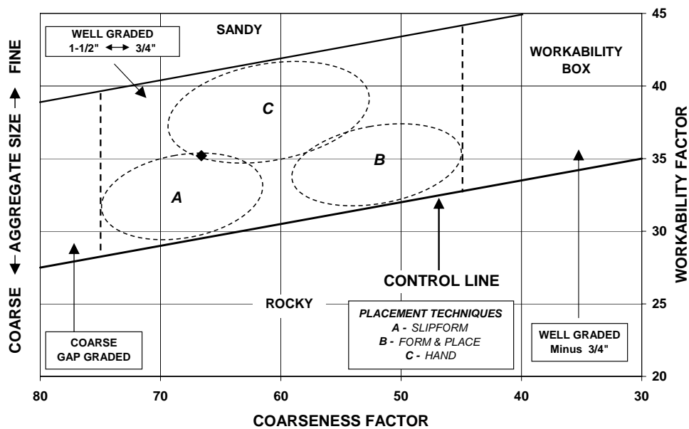
Fig. 52-USAF Aggregate Proportioning Guide-better mixture.
