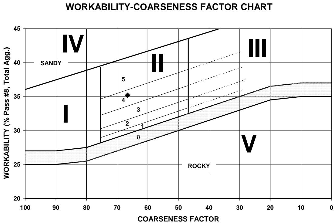
Fig. 49-IPR- better mixture.
