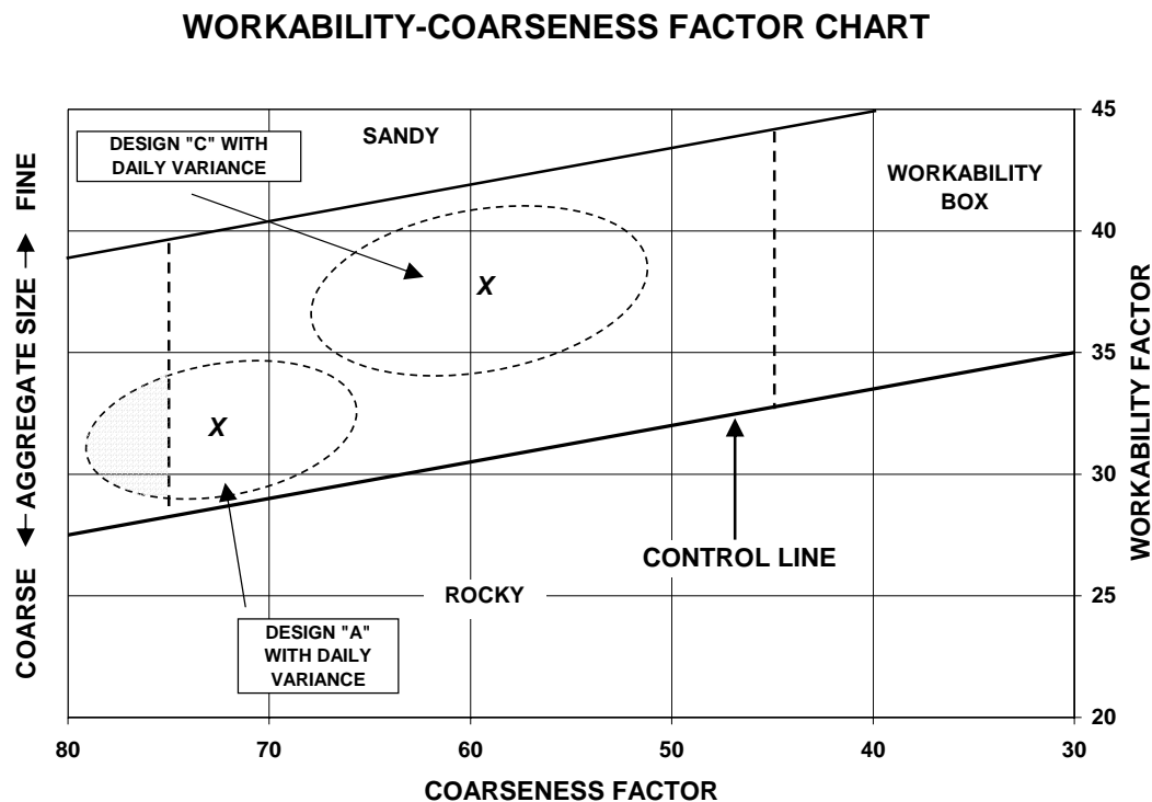
Fig. 17-Air Force Aggregate Gradation Guide showing effect of variation in gradation.
