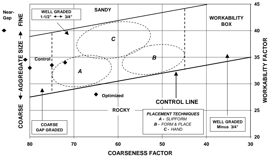
Fig. 32- Wisconsin DOT durability study-USAF Aggregate Gradation Guide.
