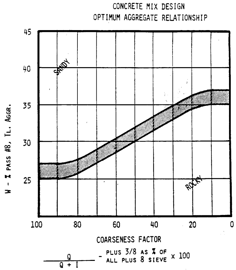
Fig. 6- Original Shilstone Coarseness Factor chart.
