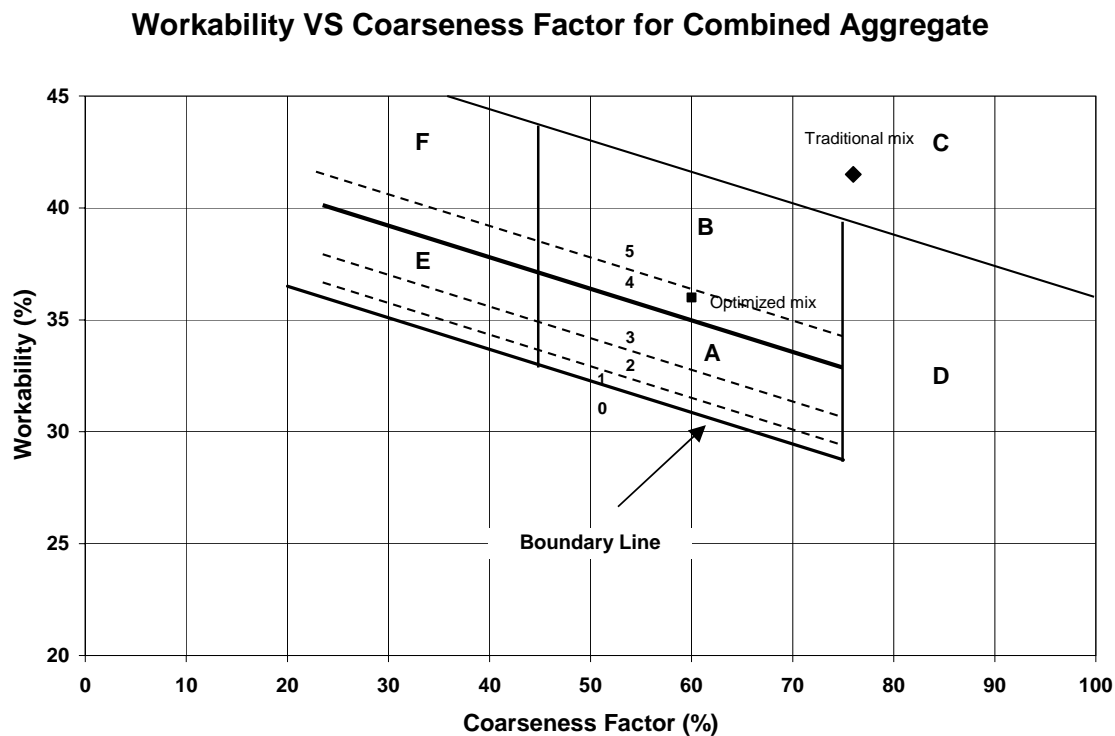
Fig. 26-Iowa DOT barrier wall mixtures-Coarseness Factor chart.
