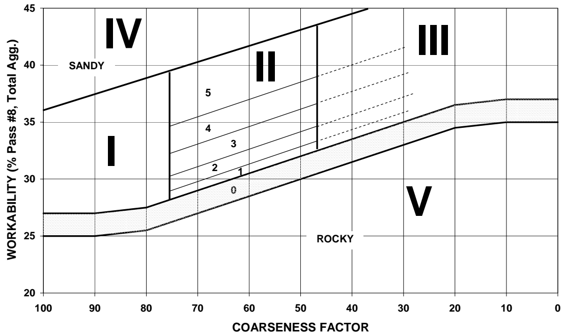
Fig. 7- Revised Shilstone Coarseness Factor chart.
