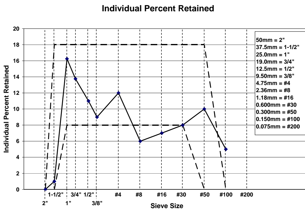
Fig. 12-Example of an acceptable mix.
