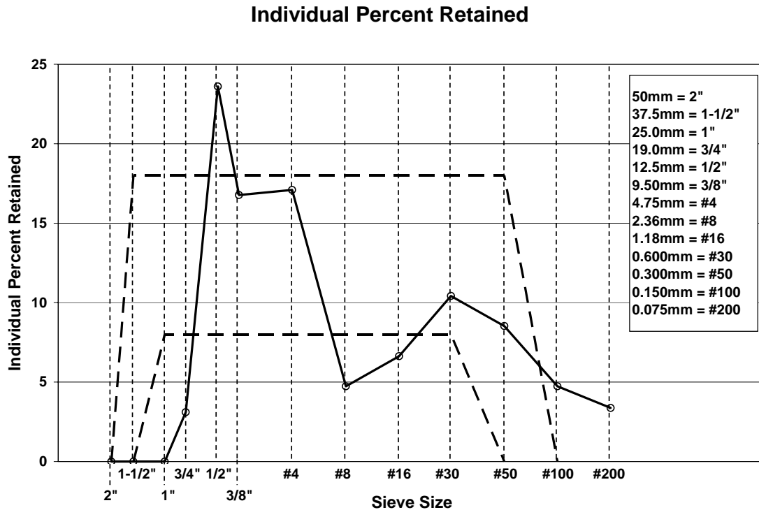
Fig. 49-IPR- better mixture.
