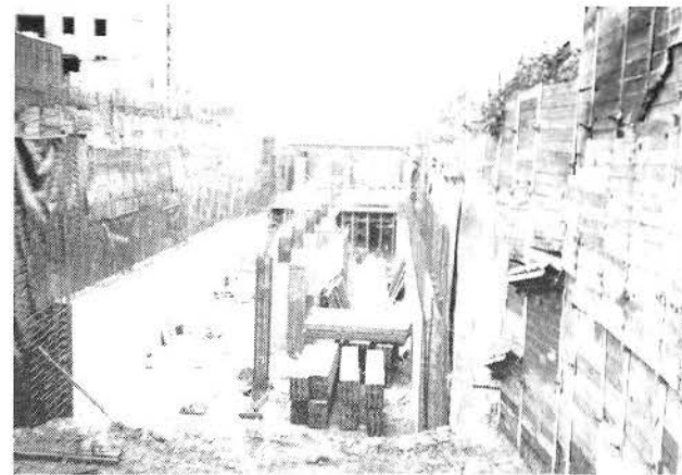
END VIEW OF STATION CONSTRUCTION PROGRESS FROM BONNIE BRAE ST. FACING WEST
