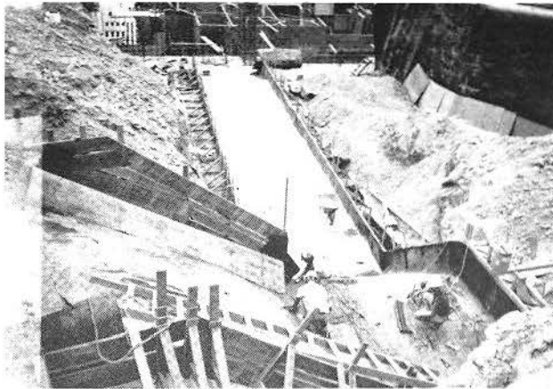
INSTALLATION OF HDPE LINER IN THE EMERGENCY STAIR #7 AREA
