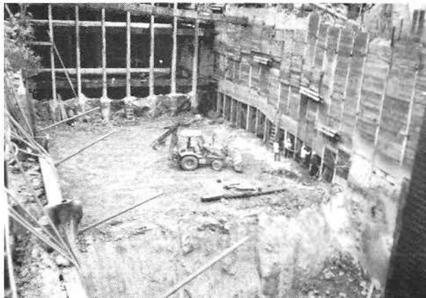
EXCAVATION AND EXCAVATION SUPPORT ARE CONTINUING AT THE A175/A171 INTERFACE
