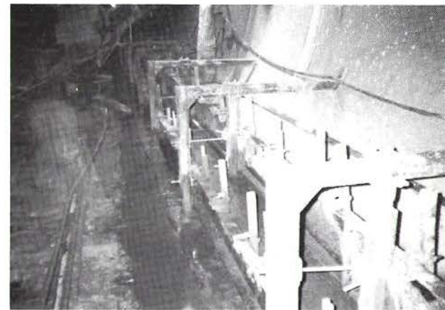
CONCRETE IN WALKWAY FORM IN 1ST STEP; 1ST LIFT (VIEW 2)
