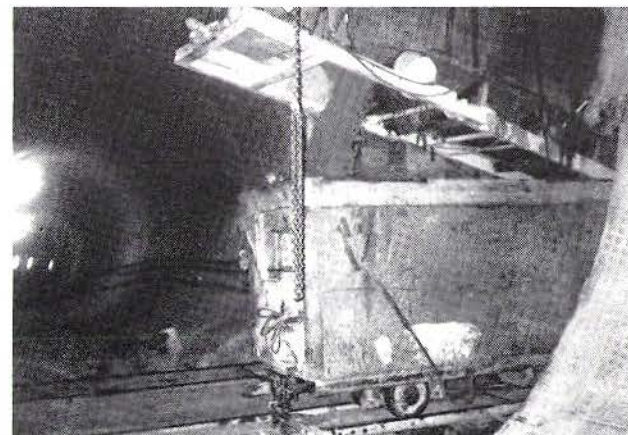
TEMPORARY MUCK REMOVAL SYSTEM AT START OF AR TUNNELING
