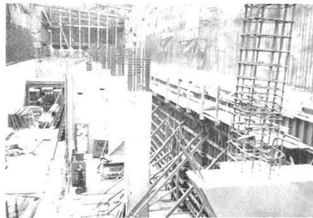
INTERIOR WALLS AT EAST END OF STATION AT BEGINNING OF DOUBLE CROSSOVER
