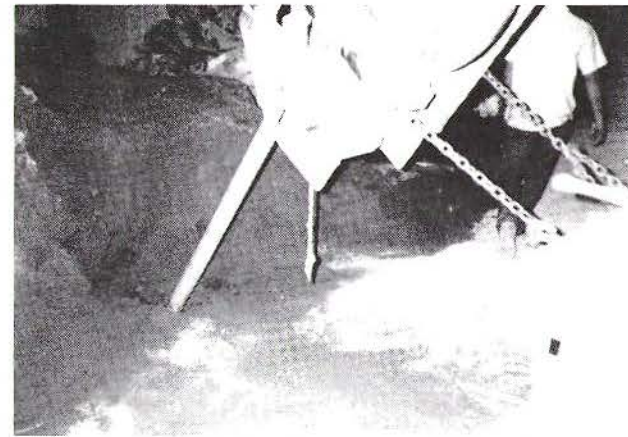
COMPACTION GROUT HOLE DRILLING AT LA JEWELERS MALL
