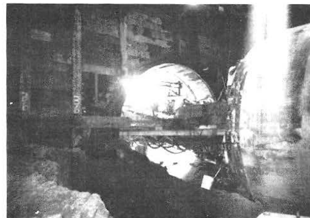
THE A141 BORING MACHINE AS IT HAS BORED THROUGH THE STATION'S NORTH BULKHEAD (1 TUNNEL COMPLETED)
