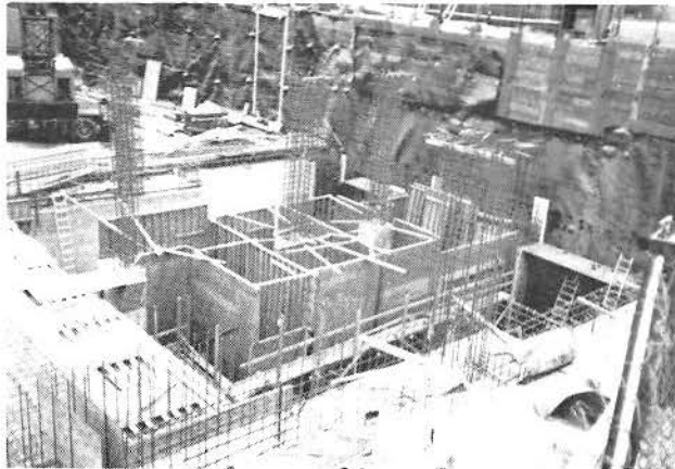
INTERIOR WALLS BEING FORMED BETWEEN BASE SLAB AND MEZZANINE AT WEST END OF STATION
