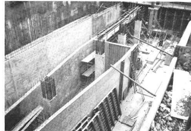
INTERIOR WALLS AT DOUBLE CROSSOVER FROM COLUMN LINE 12 TO 16
