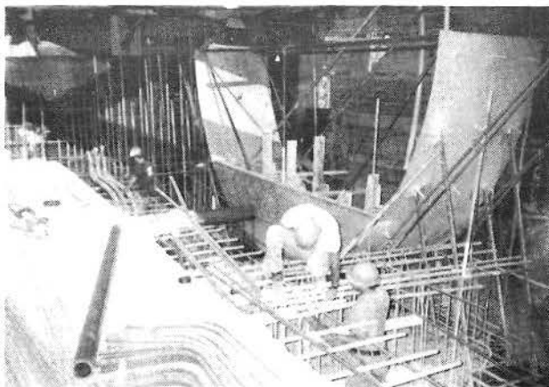
THE STATION SOUTH BULKHEAD WITH THE TUNNEL END RINGS SHOWING AND REBAR FOR INVERT 16
