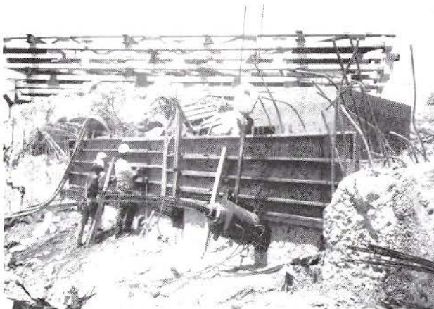
SLURRY WALL TIEBACK ANCHOR STRESSING AND PLACEMENT OF FORMS FOR THE TEMPORARY VEHICLE BRIDGE CAP BEAM
