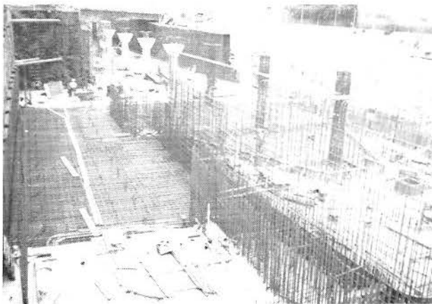
END VIEW OF STATION AND NORTH PASSAGEWAY, CONSTRUCTION PROGRESS FROM ALVARADO ST. FACING EAST
