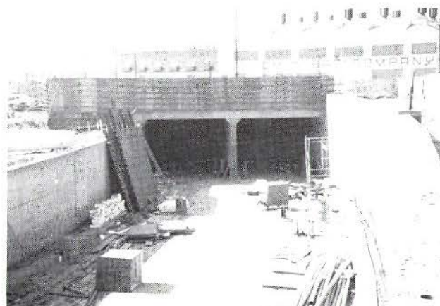
BOX STRUCTURE PORTAL - WING WALL FORMS IN PLACE
