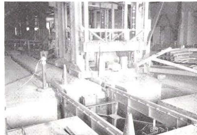
CAR HOIST MACHINE INSTALLED. TRUCK HOIST READY FOR INSTALLATION. CAR SUPPORT MACHINERY IN BACKGROUND
