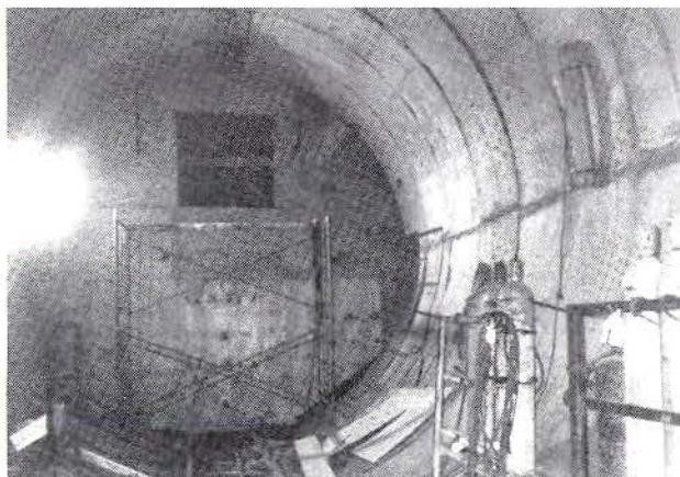
TEMPORARY VENTILATION BULKHEAD AT END OF AL TUNNEL
