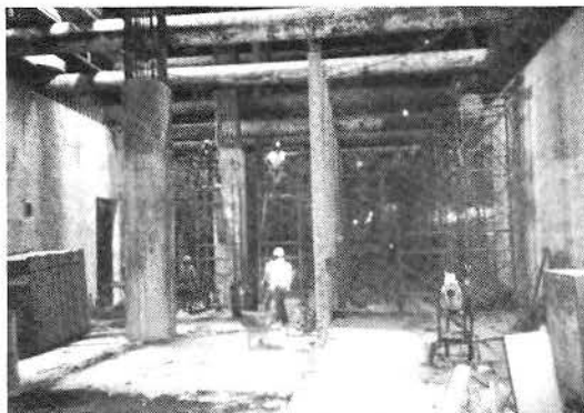
STATION'S INVERT 15/14 - ALSO VISIBLE ARE THE COLUMNS AND EXTERIOR/INTERIOR WALLS AND THE SCAFFOLDING FOR MEZZANINE SLAB AREA 14
