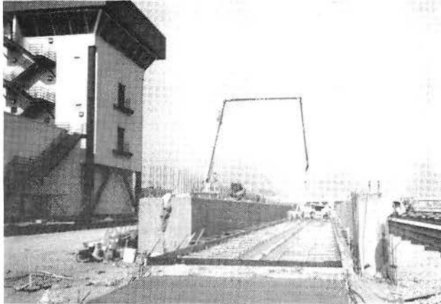
CONCRETE POUR FOR HEAVY CAR CLEANING PLATFORM
