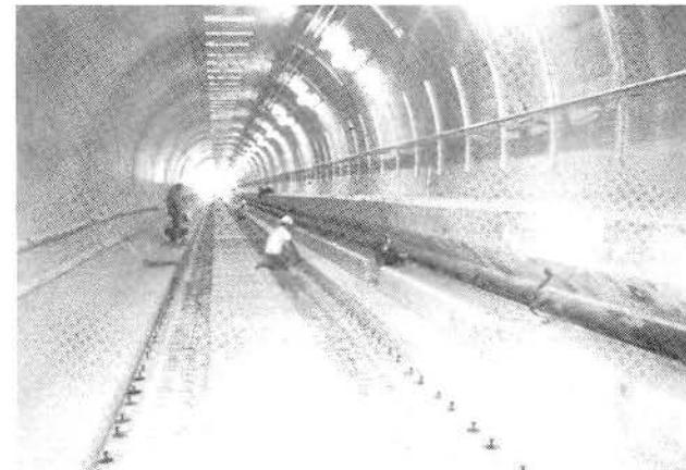
LATERAL ADJUSTMENTS BEING MADE ON FLOATING SLABS IN AL TUNNEL
