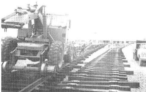
UNLOADING CWR STRINGS FROM RAIL TRAIN FOR RA AND MR-3 TRACKS
