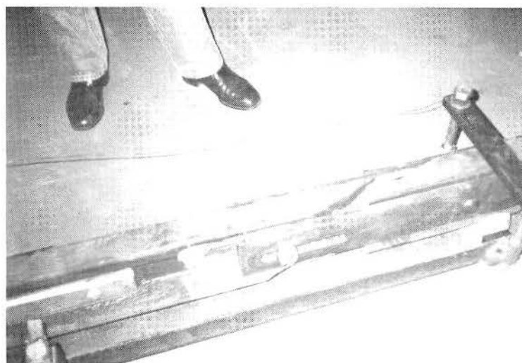
EXPANSION JOINT DURING QUALIFICATION TESTING
