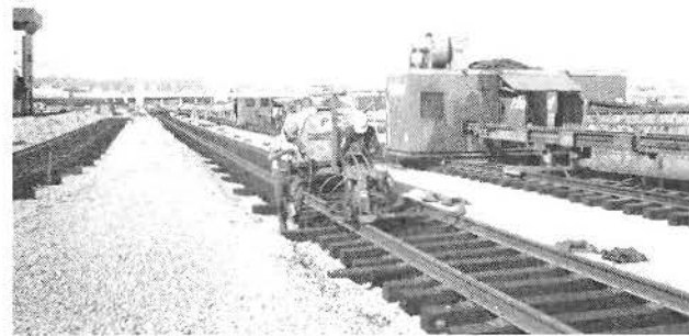
SPIKING TRACK 10 AND WELDING PLANT SET ON TRACK 9 IN OPERATION
