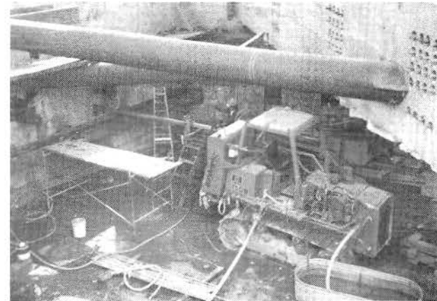
DRILLING HORIZONTAL GROUT HOLES FOR CHEMICAL GROUTING PRIOR TO TUNNEL EXCAVATION
