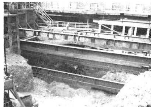
SOUTHEAST ENTRANCE EXCAVATION AND EXCAVATION SUPPORT SYSTEM
