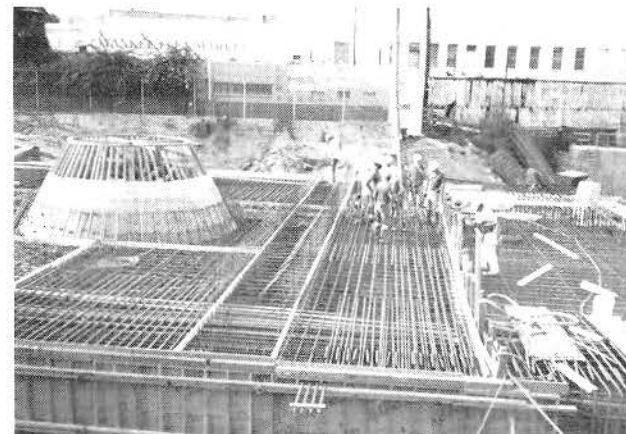
INITIAL PLACEMENT OF CONCRETE FOR ROOF SLAB NEAR STATION SKYLIGHT
