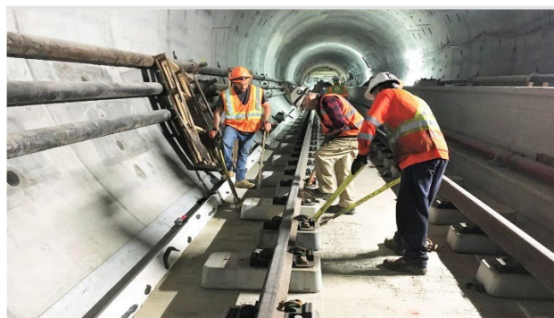
Reach 4 (Tail Track) Track Installation
