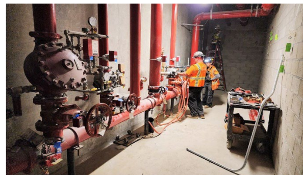
Sprinkler Valve Installation at Wilshire/Fairfax Station
