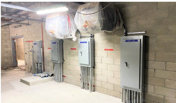
Wilshire/La Cienega Station Power Panel Installation
