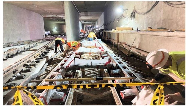
Concrete Placement at Wilshire/La Brea Crossover
