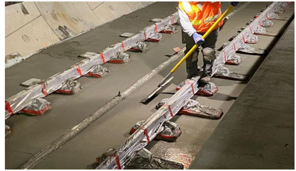
Reach 4 (Tail Track) Track Concrete Infill
