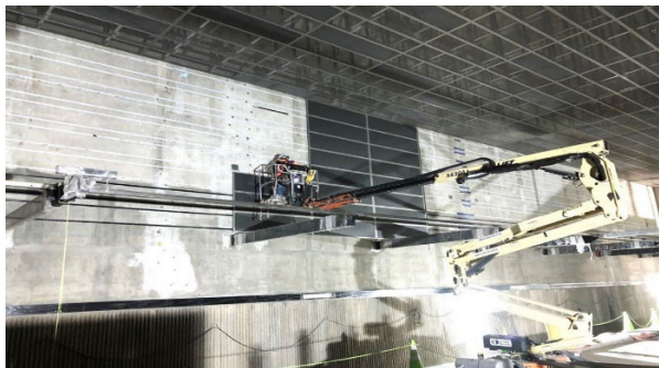
Panel Installation at Wilshire/Fairfax Station
