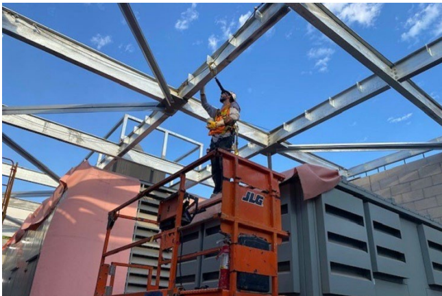
Wilshire/La Cienega Station Emergency Generator Steel Roof Installation
