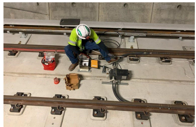
Reach 4 Tunnel (Tail Track) Train Control Installation
