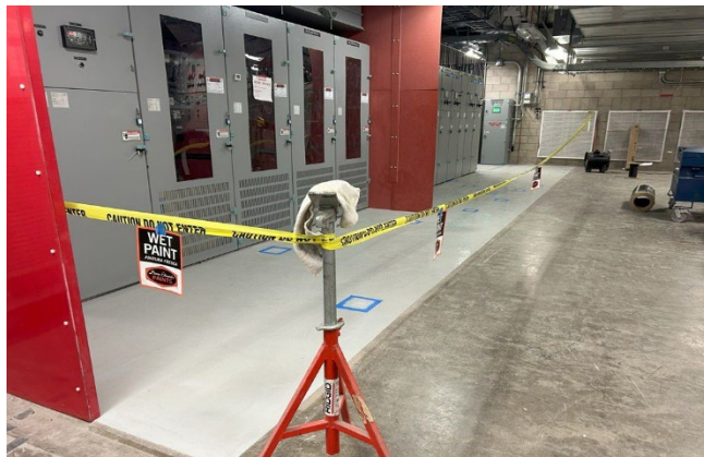
Wilshire/La Brea Station TPSS Room 206
