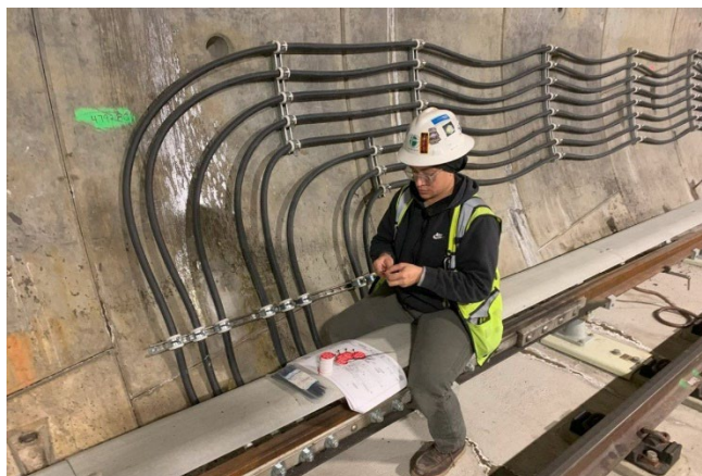
Reach 2 Tunnel (La Brea to Fairfax) Labeling Feeder Cables
