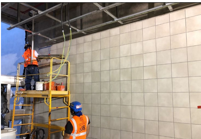
Wilshire/La Cienega Station Entrance Structure Wall Tile Placement
