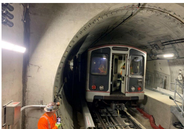
Reach 3 (Fairfax to La Cienega) Dead Car Train Test Entering Wilshire/La Cienega Station
